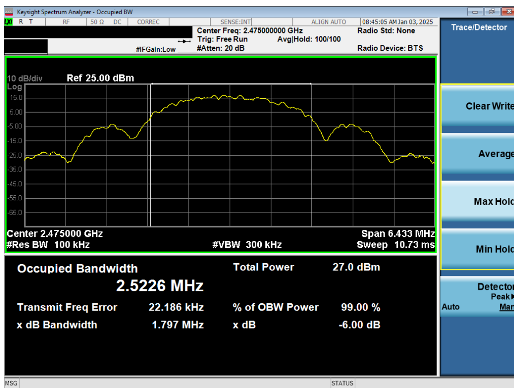
Plot 7-6. 6dB BW & 99% OBW Antenna WF7b (802.15.4, Ch. 25)
