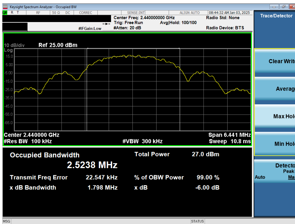
Plot 7-5. 6dB BW & 99% OBW Antenna WF7b (802.15.4, Ch. 18)
