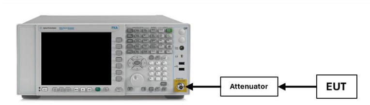
Figure 7-1. Test Instrument & Measurement Setup
