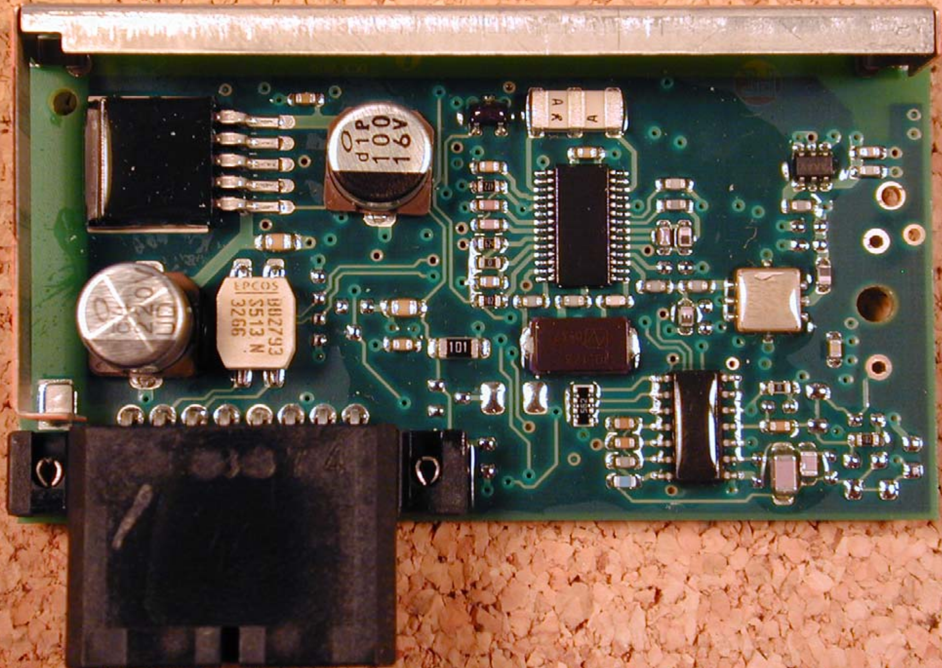
PCB (top)
