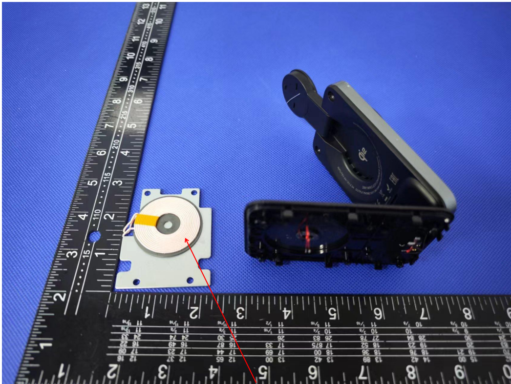
EARPHONE Antenna
