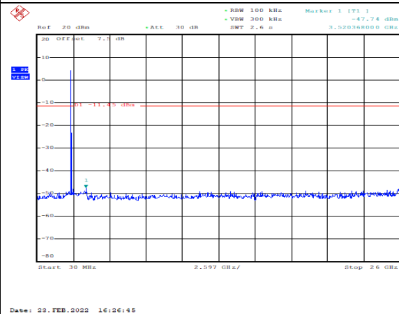
Conducted spurious emission: Ch19, 30MHz~26GHz
