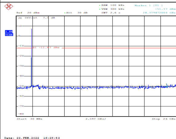
Conducted spurious emission: Ch39, 30MHz~26GHz
