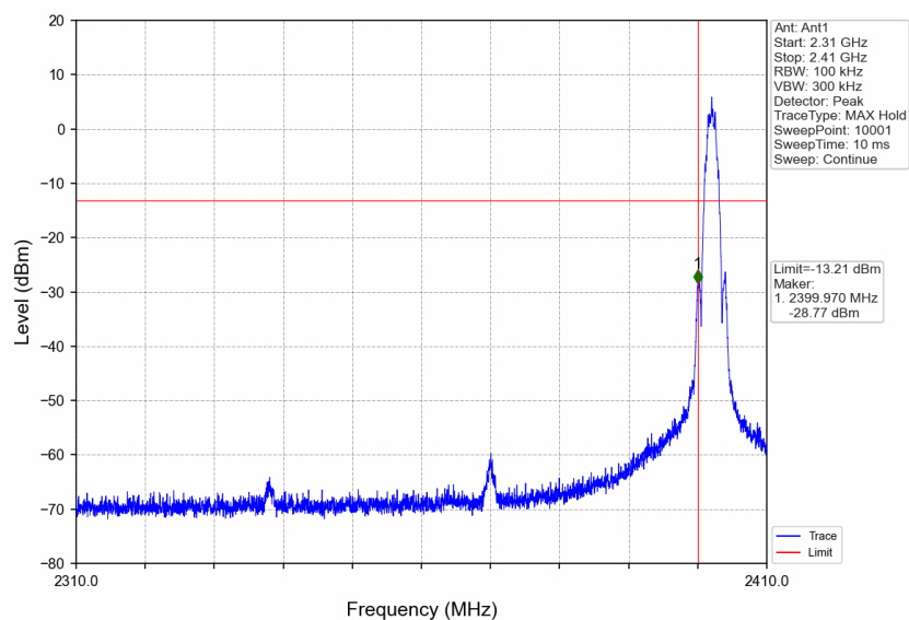
2M_LCH_2402MHz_DataRate= Ant1_NTNV
