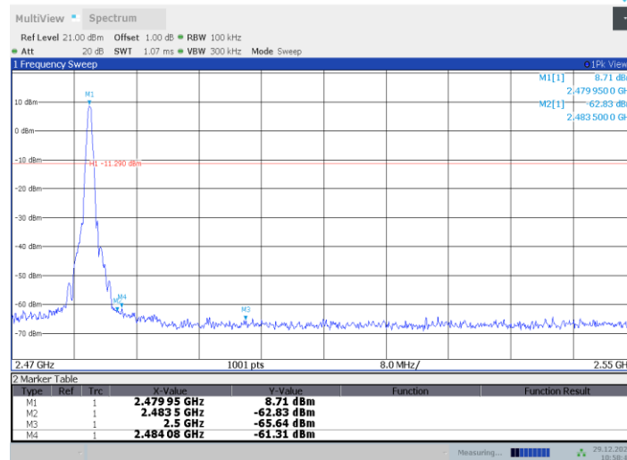
DH5_Ant6_High_2480
