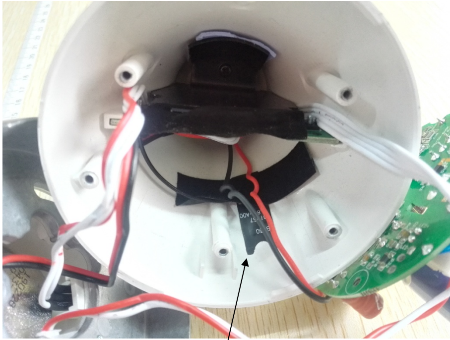
5.8G antenna location
