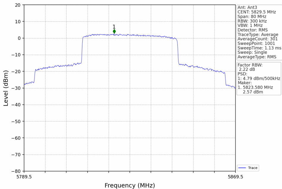
40M_HCH_5829.5MHz_Ant3_NTNV
