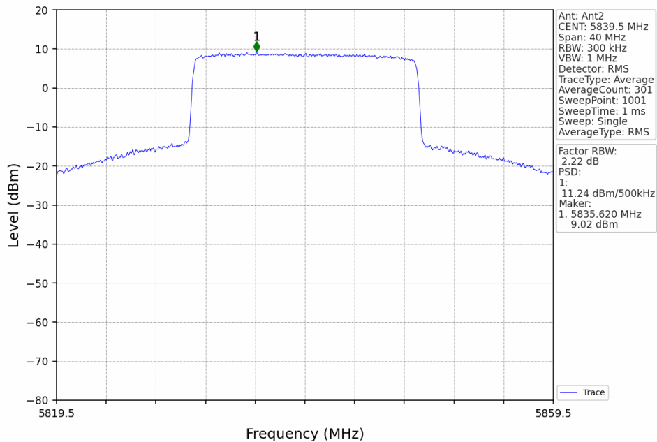
20M_HCH_5839.5MHz_Ant2_NTNV
