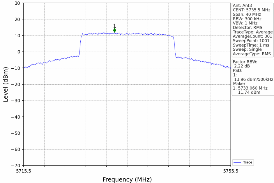
20M_LCH_5735.5MHz_MIMO_NTNV
