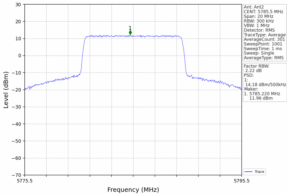
10M_MCH_5785.5MHz_Ant2_NTNV
