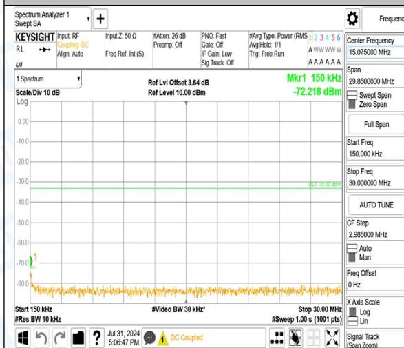
Band2_3MHz_QPSK_18900_15RB#0_1000~3000_1000~3000
