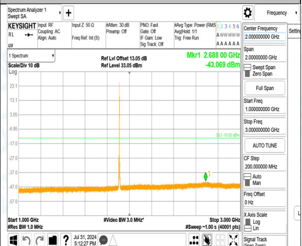
Band2_3MHz_16QAM_19185_1RB#14_1000~3000_1000~3000
