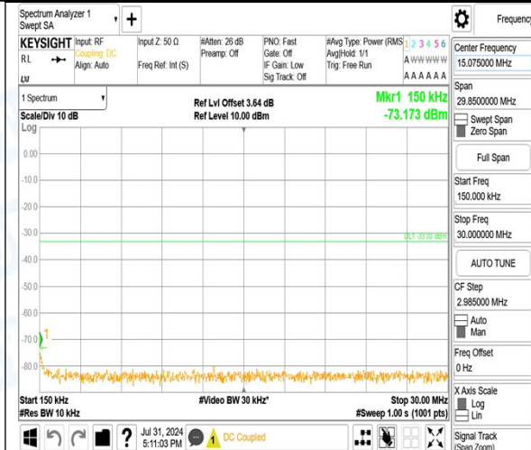
Band2_3MHz_QPSK_19185_1RB#14_1000~3000_1000~3000
