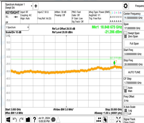
Band2_3MHz_QPSK_18900_15RB#0_0.15~30_0.15~30
