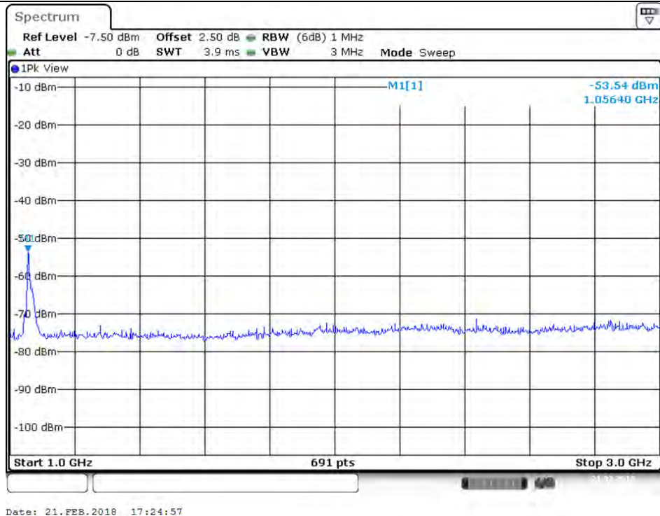
Plot on Configuration VHT20 / 5240 MHz / Peak / Port 2 / 1GHz~3GHz
