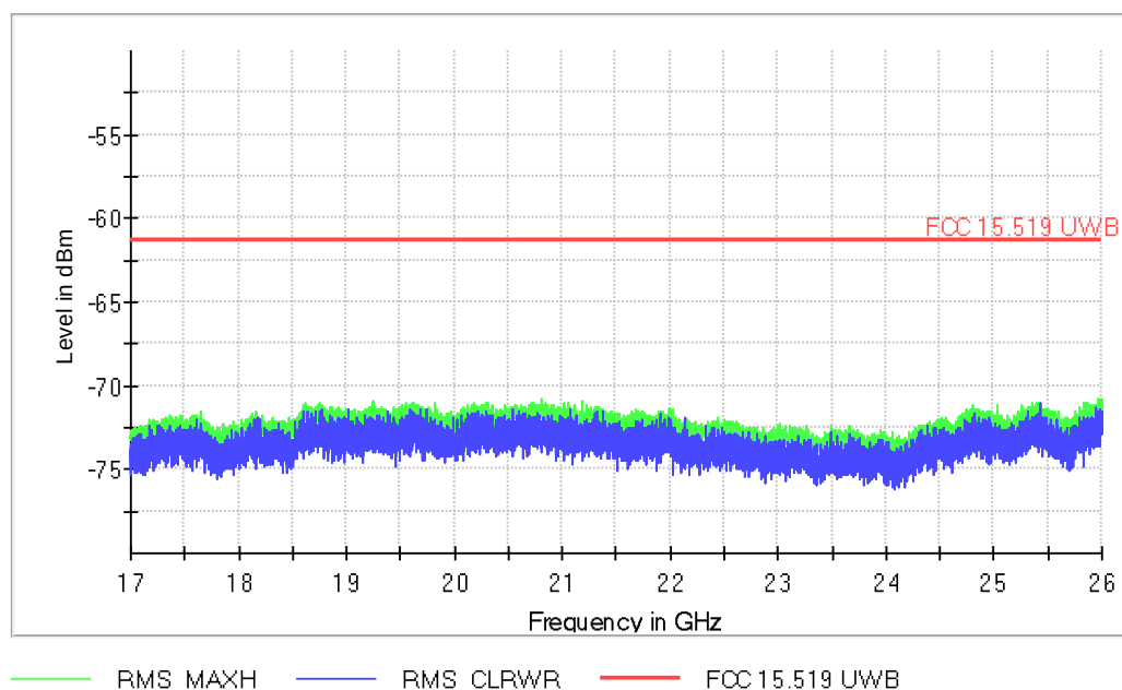
FCC 15.519_17GHz-26GHz
