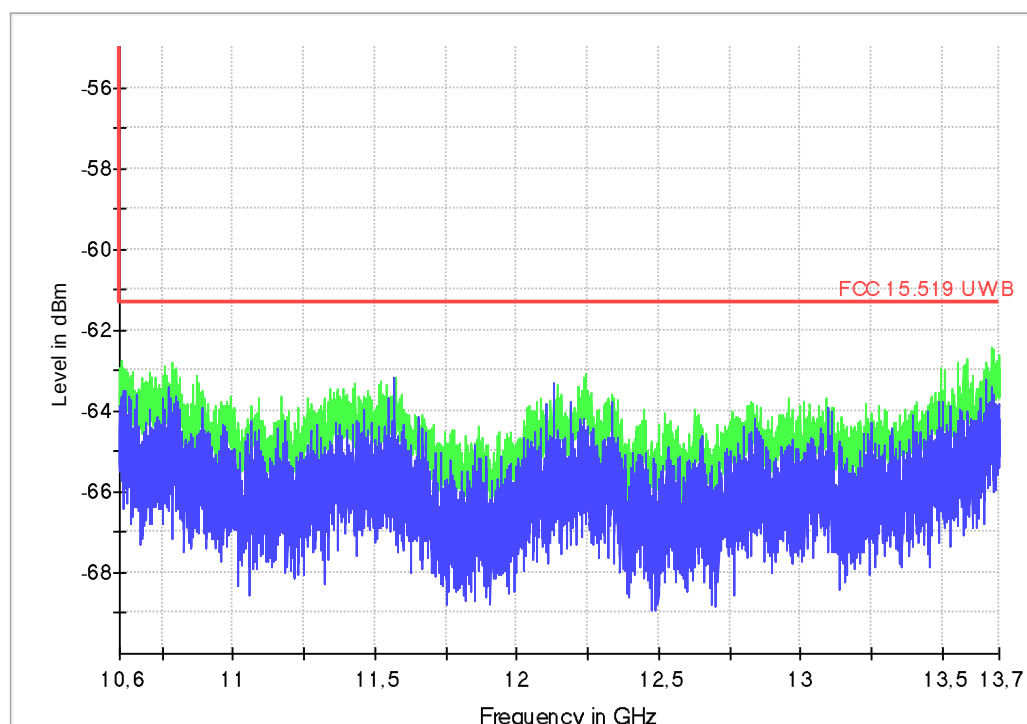
FCC 15.519_10.6-13.7GHz
