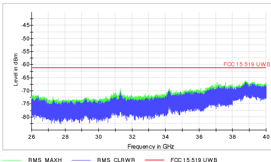
FCC 15.519_26GHz-40GHz
