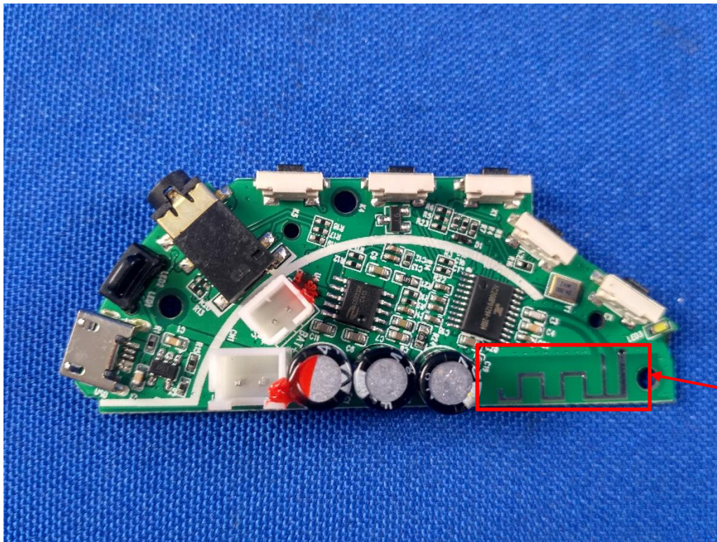
Antenna 2402-2480MHz
