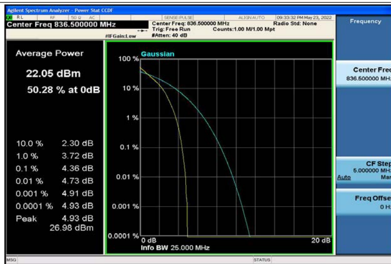
Band5-3MHz-QPSK-20525-15RB#0
