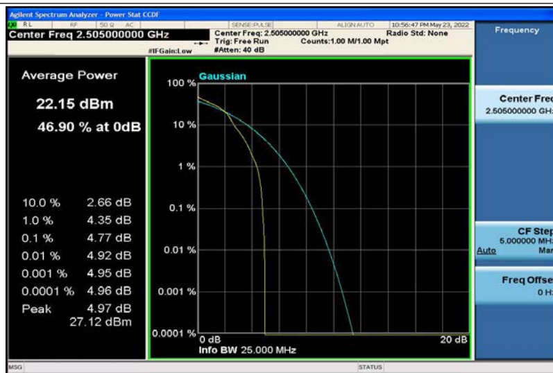
Band7-10MHz-16QAM-20800-1RB#0
