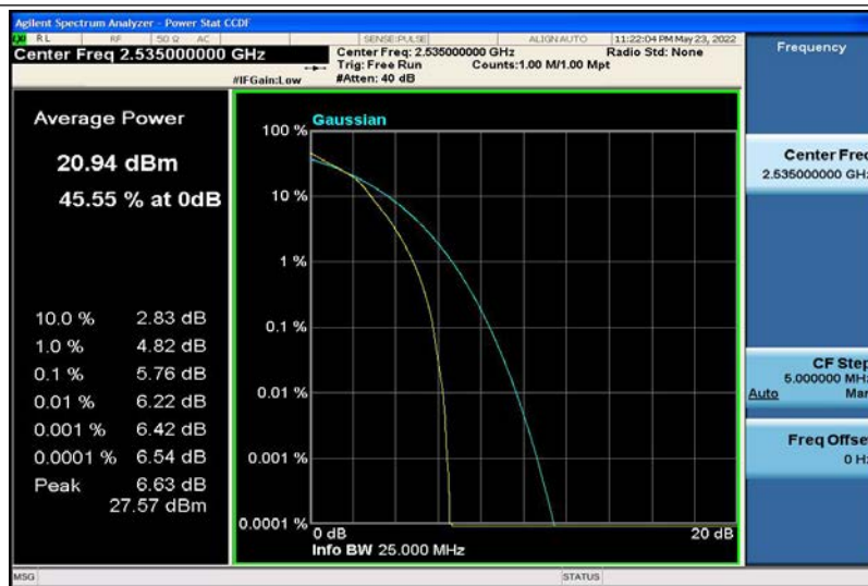
Band7-15MHz-16QAM-21100-75RB#0
