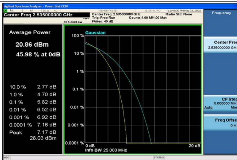
Band7-20MHz-16QAM-21100-100RB#0
