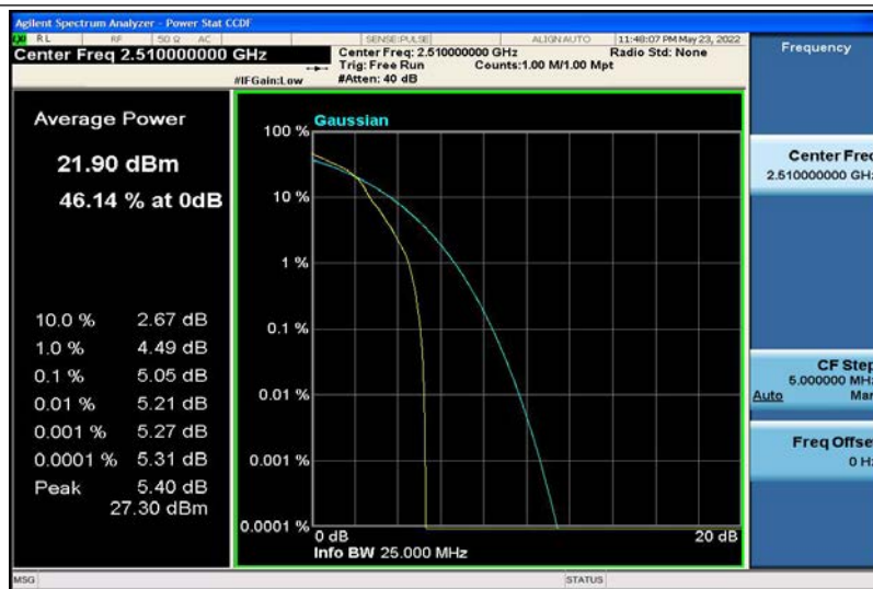
Band7-20MHz-16QAM-20850-1RB#0
