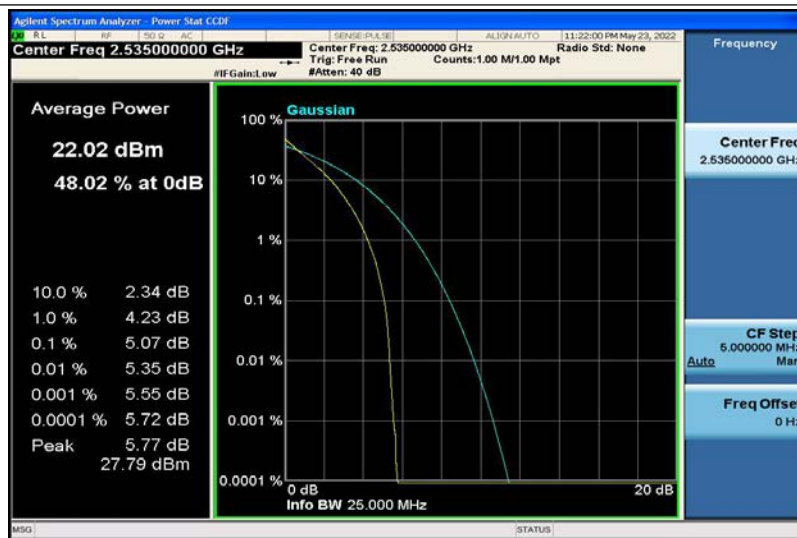
Band7-15MHz-QPSK-21100-75RB#0
