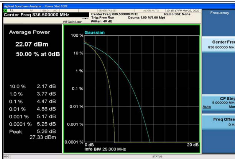
Band5-10MHz-QPSK-20525-50RB#0
