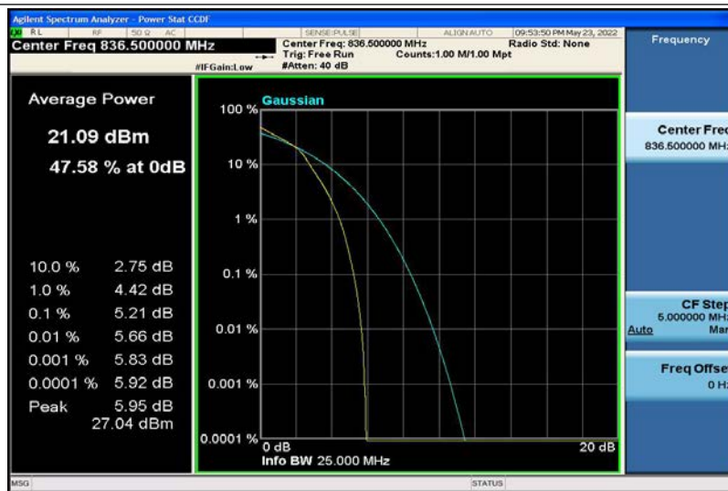
Band5-5MHz-16QAM-20525-25RB#0
