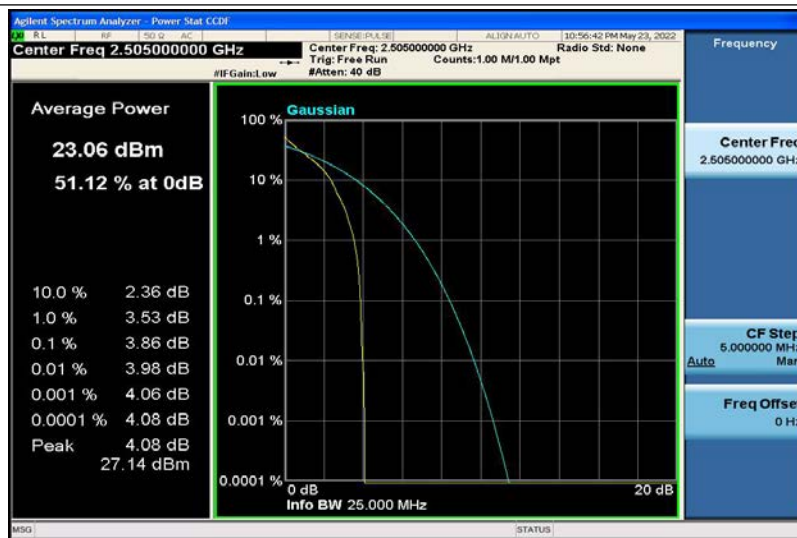
Band7-10MHz-QPSK-20800-1RB#0
