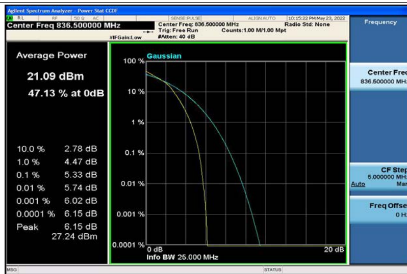
Band5-10MHz-16QAM-20525-50RB#0
