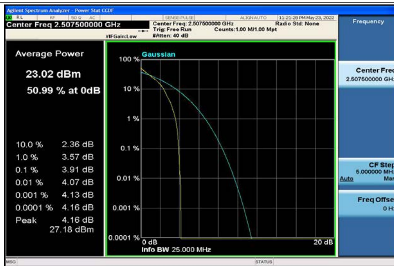
Band7-15MHz-QPSK-20825-1RB#0
