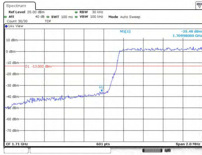
Band4-1.4MHz-QPSK-19957-6RB#0
