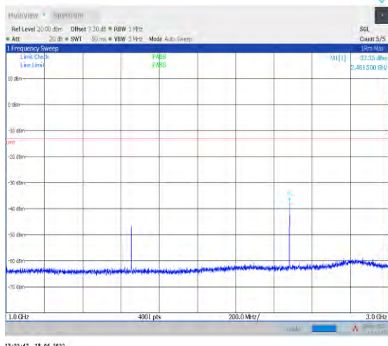
1-N5--15-20-M-1-DFT-PI2BPSK-Inner_1RB_Left-1@ 1-1000-3000-Ant1--37.35--13-PASS
