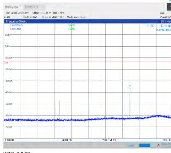
1-N5--15-20-H-1-DFT-PI2BPSK-Inner_1RB_Left-1@ 1-1000-3000-Ant1--37.44--13-PASS
