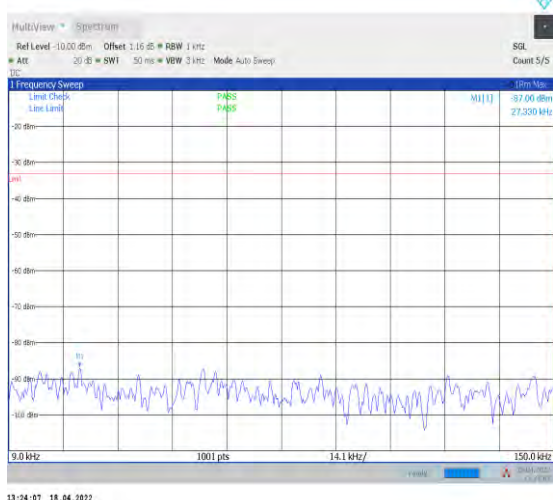
1-N5--15-20-H-1-DFT-PI2BPSK-Inner_1RB_Left-1@ 1-0.009-0.15-Ant1--87.00--33-PASS
