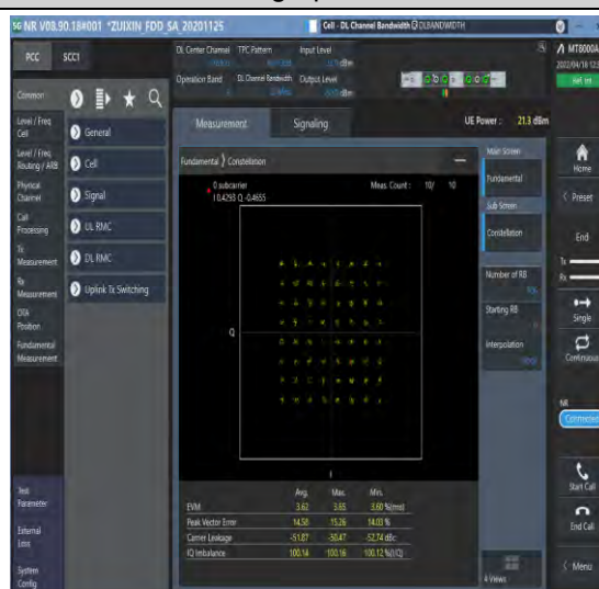
1-N5--15-20-M-8-CP-64QAM-Outer_Full-106@0-Ant1-see graph-PASS
