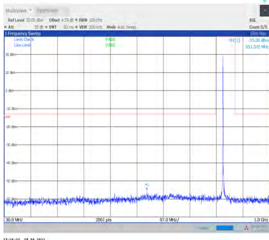
1-N5--15-20-H-1-DFT-PI2BPSK-Inner_1RB_Left-1@ 1-30-1000-Ant1--55.30--13-PASS
