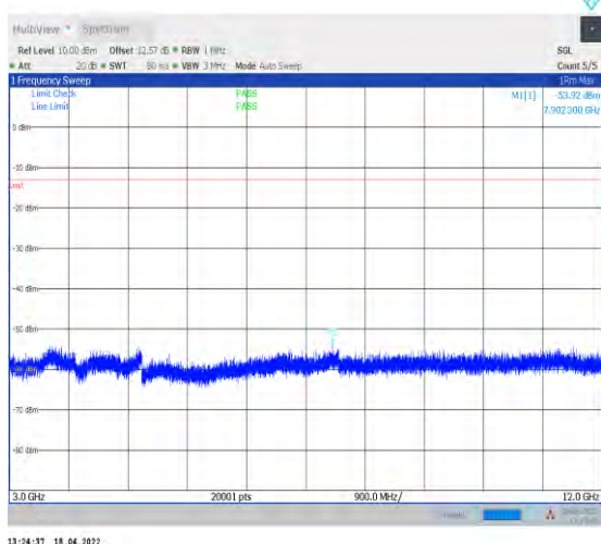
1-N5--15-20-H-1-DFT-PI2BPSK-Inner_1RB_Left-1@ 1-3000-12000-Ant1--53.92--13-PASS
