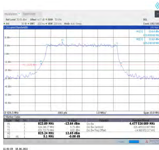
1-N5--15-5-L-4-DFT-64QAM-Outter_Full-25@0-Ant1-4 4.478-5.100-≤5-PASS
