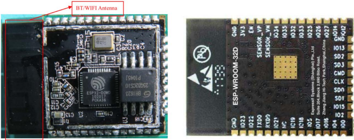
Figure 1.1-4: Wi-Fi/BLE module without RF shield
