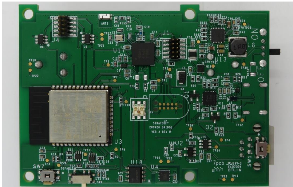
Figure 1.1-1: Top view
