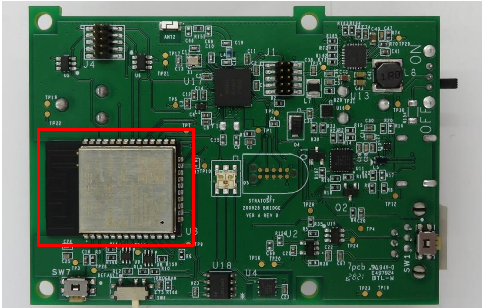
Figure 1.1-3: Wi-Fi/BLE module location
