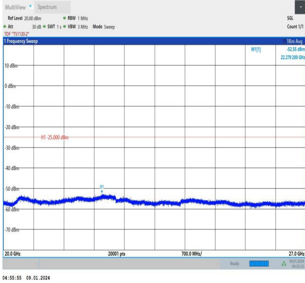
Band41_10MHz_QPSK_41540_1RB#49_20000~27000_2000 0~27000
