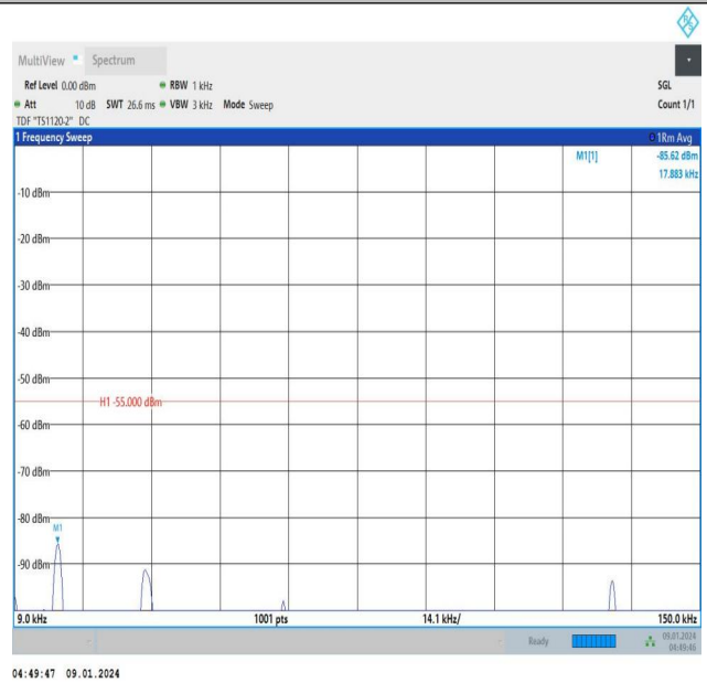
Band41_10MHz_16QAM_39700_1RB#0_0.009~0.15_0.009~0.15
