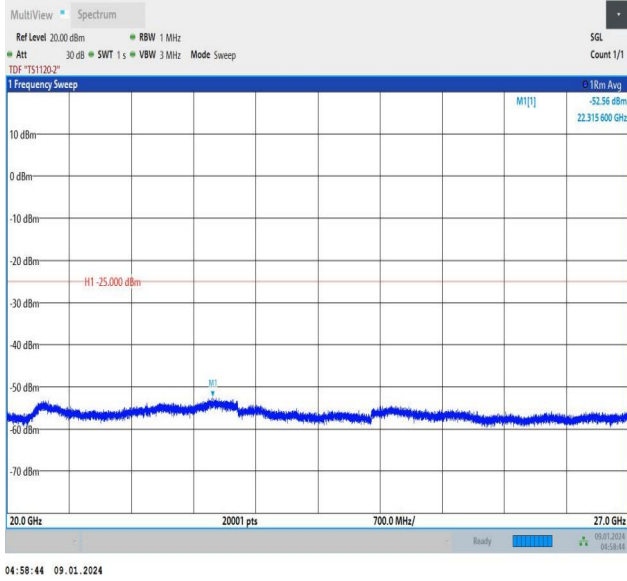
Band41_10MHz_QPSK_41540_50RB#0_20000~27000_2000 0~27000
