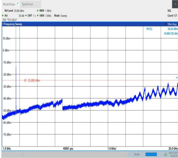
Band41_15MHz_QPSK_39725_1RB#0_1000~20000_1000~20000
