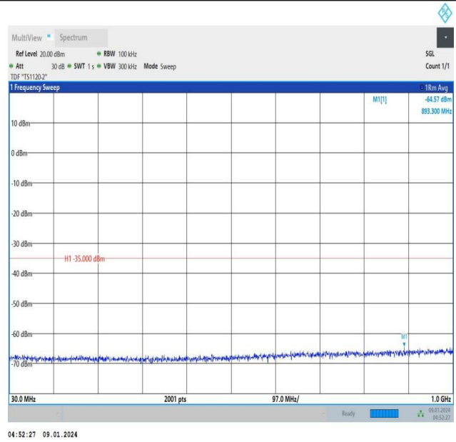
Band41_10MHz_16QAM_40620_1RB#0_30~1000_30~1000
