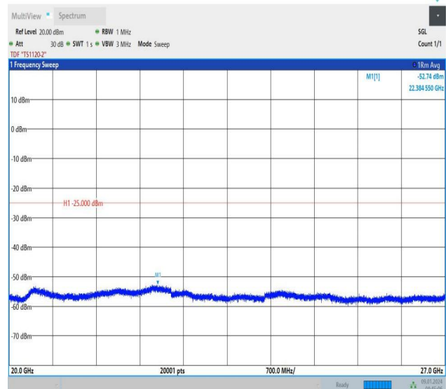
Band41_5MHz_16QAM_40620_25RB#0_20000~27000_20000~27000
