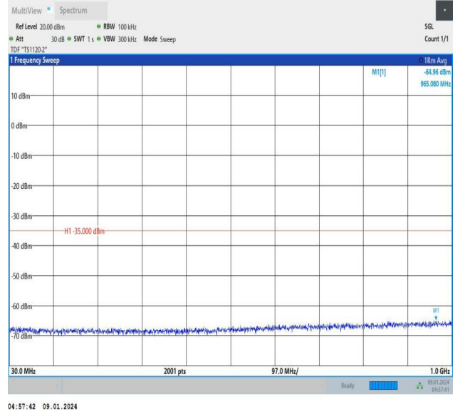
Band41_10MHz_QPSK_40620_50RB#0_30~1000_30~1000
