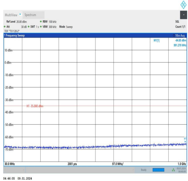
Band41_5MHz_16QAM_41565_1RB#0_30~1000_30~1000
