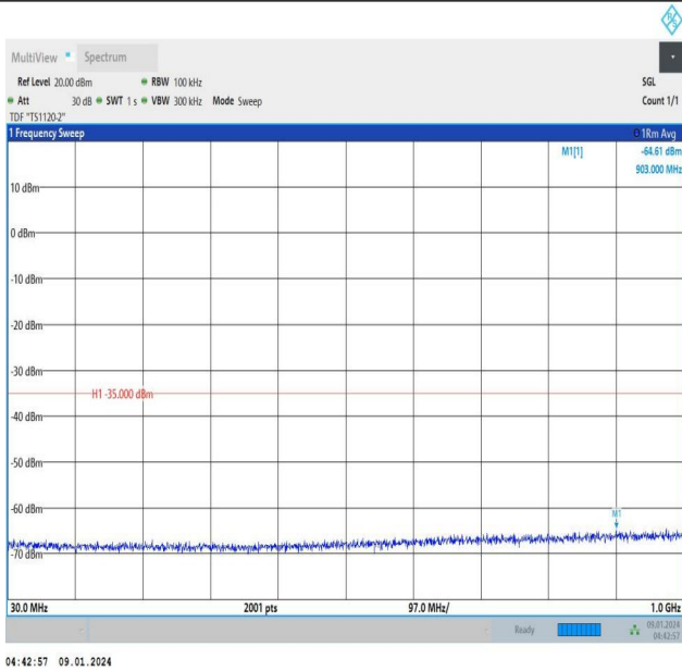
Band41_5MHz_QPSK_40620_1RB#24_30~1000_30~1000
