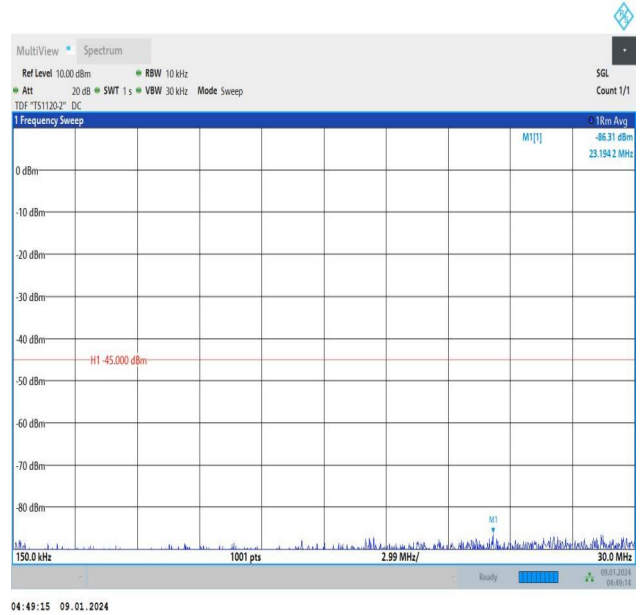
Band41_10MHz_QPSK_39700_1RB#0_0.15~30_0.15~30
