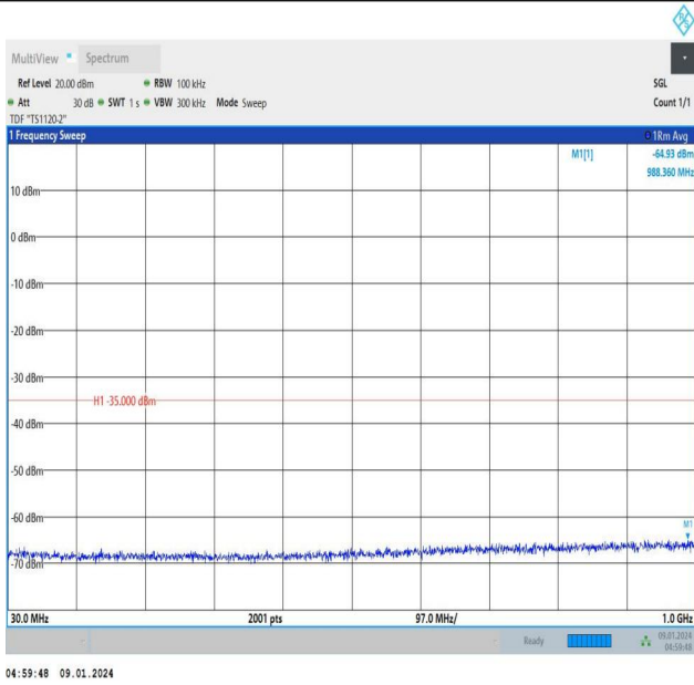
Band41_15MHz_16QAM_39725_1RB#0_30~1000_30~1000
