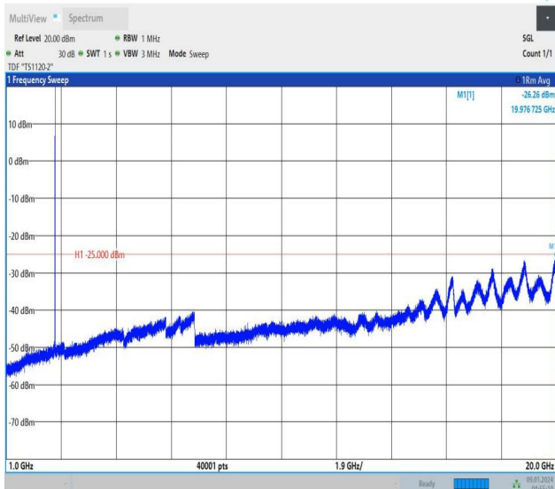
Band41_10MHz_16QAM_41540_1RB#0_1000~20000_1000~20000
