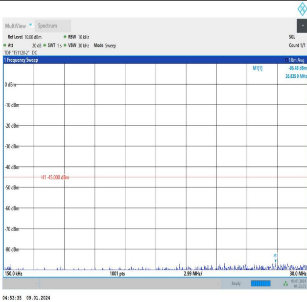
Band41_10MHz_16QAM_40620_1RB#49_0.15~30_0.15~30
