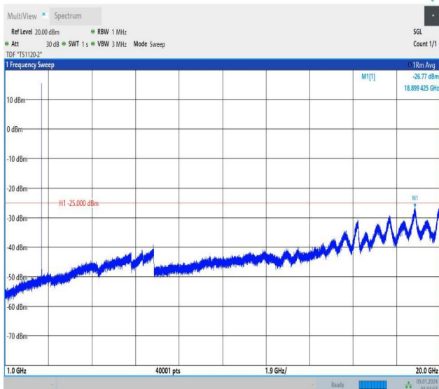
Band41_5MHz_16QAM_40620_25RB#0_1000~20000_1000~20000
