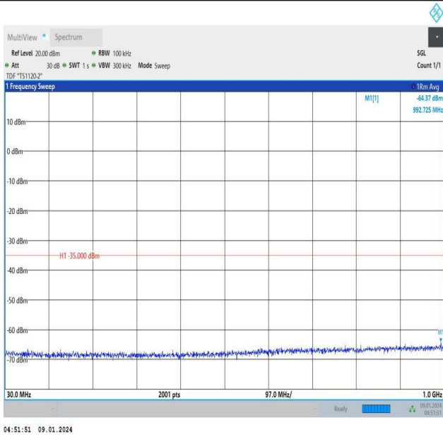
Band41_10MHz_QPSK_40620_1RB#0_30~1000_30~1000
