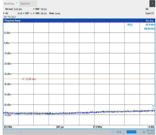
Band41_10MHz_16QAM_41540_1RB#0_30~1000_30~1000
