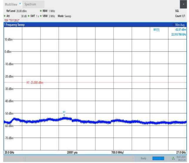
Band41_10MHz_16QAM_39700_1RB#49_20000~27000_20000~27000
