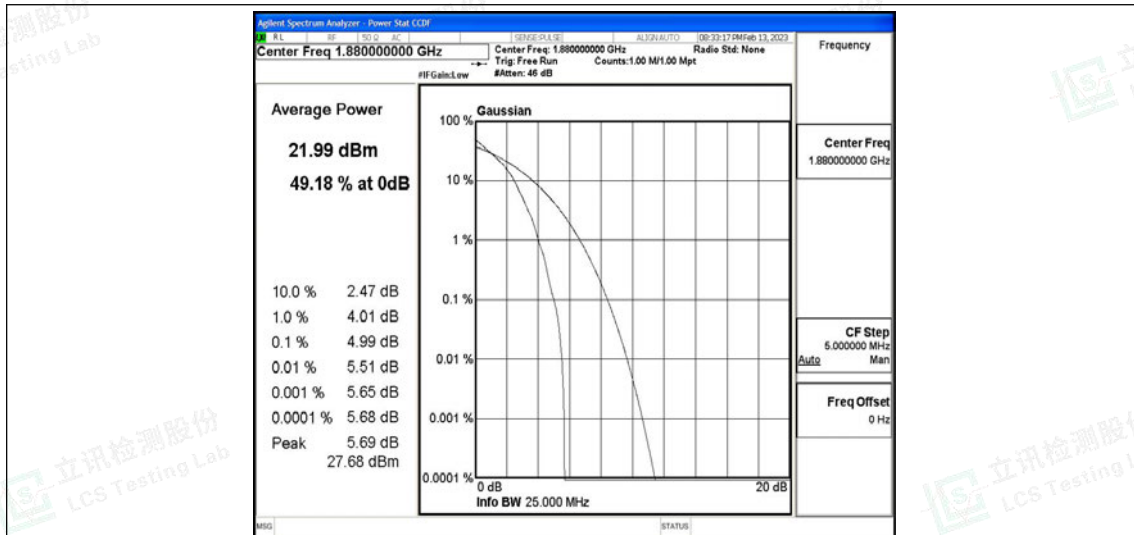
Band2-1.4MHz-QPSK-18900-6RB#0
