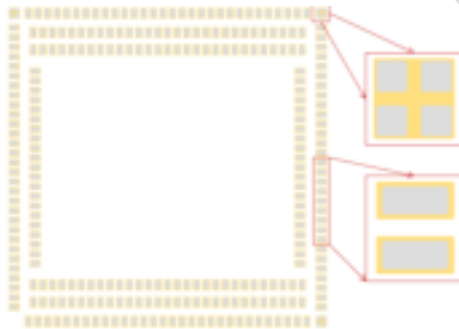
Figure 1-8. Stencil Aperture
