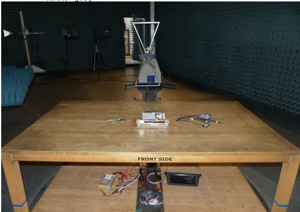
Photo 2: Test setup for radiated measurements (Enclosure, semi-anechoic chamber, 30 MHz to 1 GHz, intentional radiator §15)
