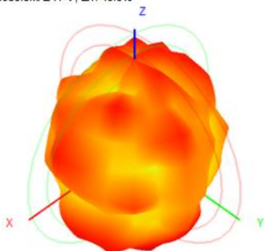
5850.0MHz H+V, Eff: 48.0%
