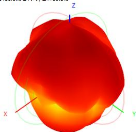
2450.0MHz H+V, Eff: 59.5%
