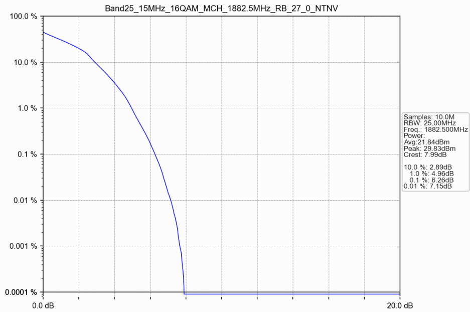
Band25 15MHz 16QAM MCH 1882.5MHz RB 27 0 NTNV
