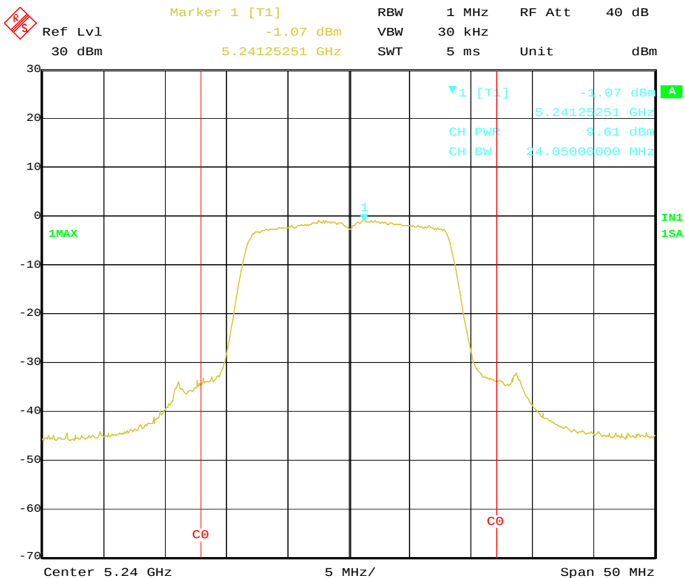
Plot 1-1b. Conducted Transmit Output Power of 5240MHz (OFDM, 6Mbps)
