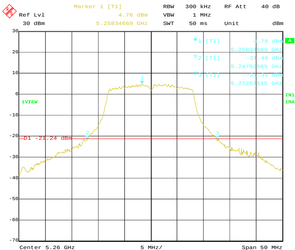
Plot 1-2a. 26dB Bandwidth of 5260MHz (OFDM, 6Mbps)
