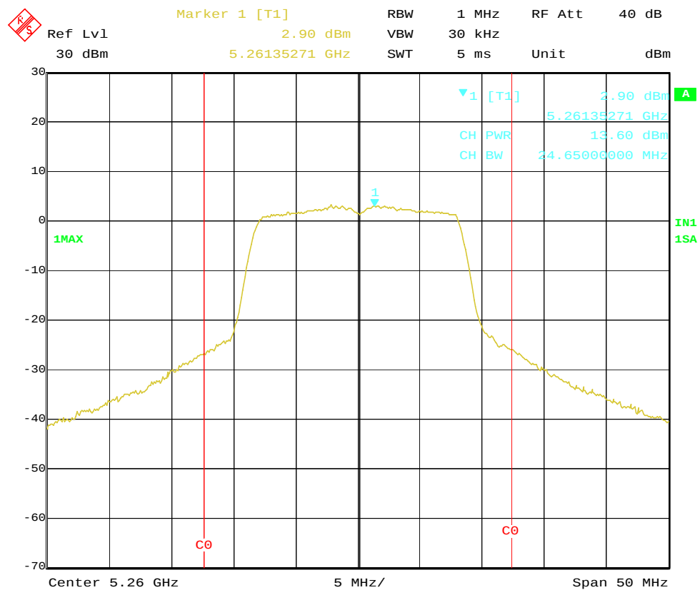
Plot 1-2b. Conducted Transmit Output Power of 5260MHz (OFDM, 6Mbps)
