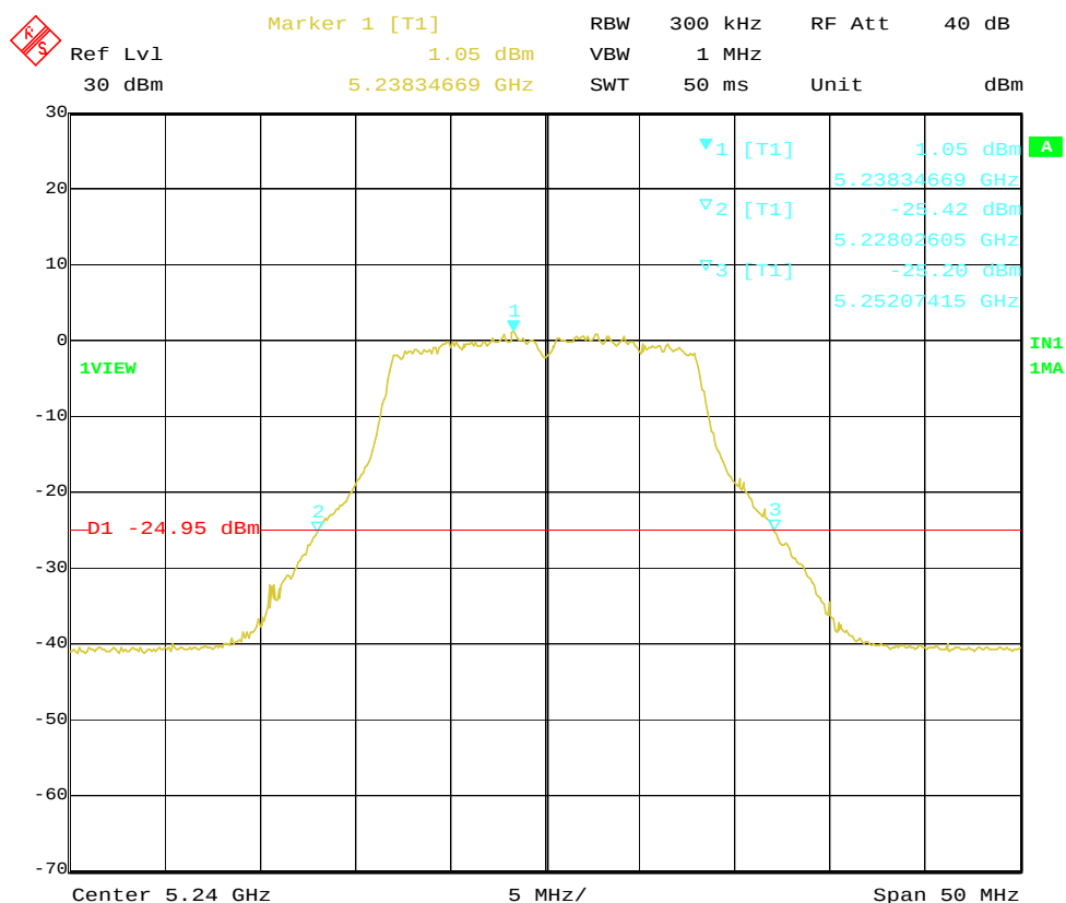
Plot 1-1a. 26dB Bandwidth of 5240MHz (OFDM, 6Mbps)
