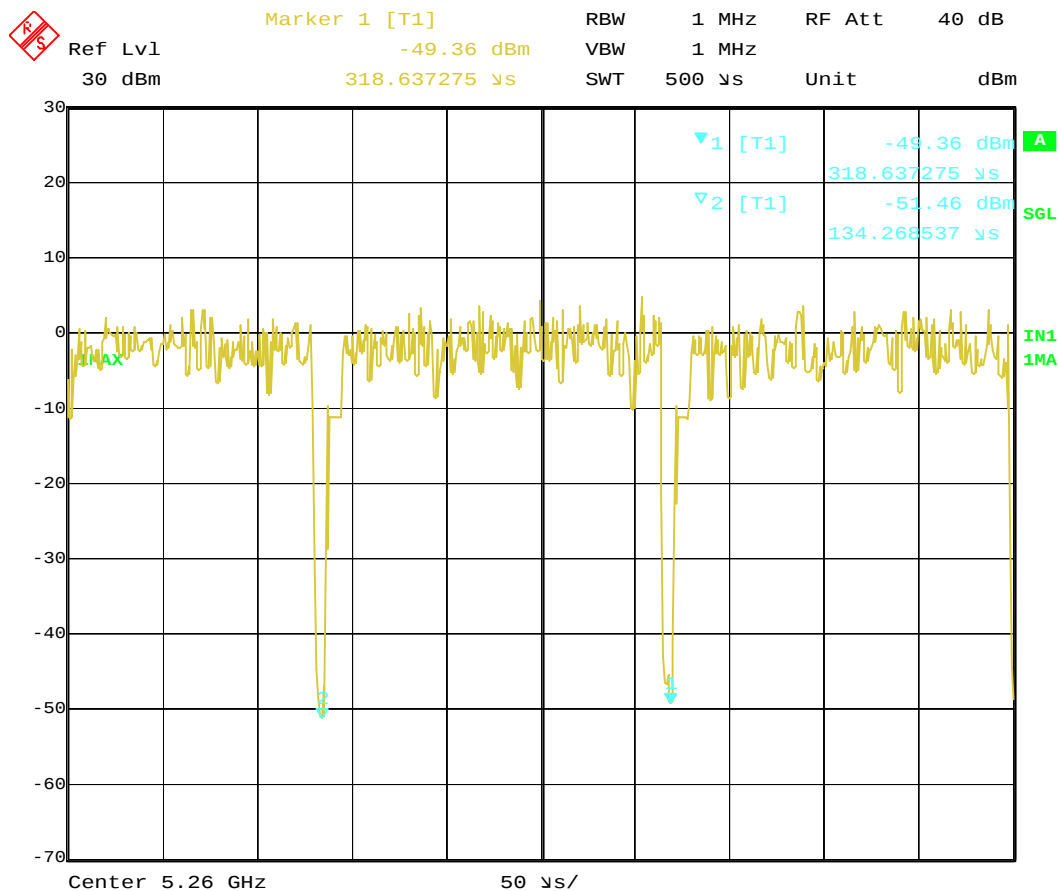
Plot 1-0 Transmission Pulse Duration
