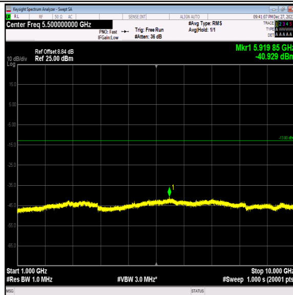
Band5-4233-2-1000~10000MHz-PASS
