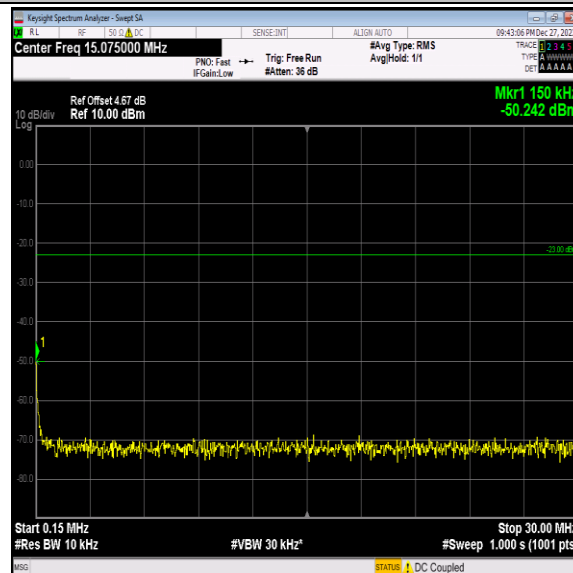
Band5-4182-3-0.15~30MHz-PASS
