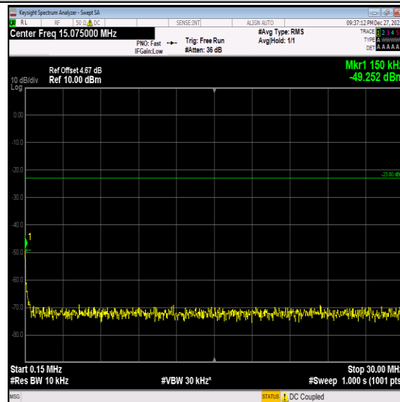
Band5-4233-1-0.15~30MHz-PASS
