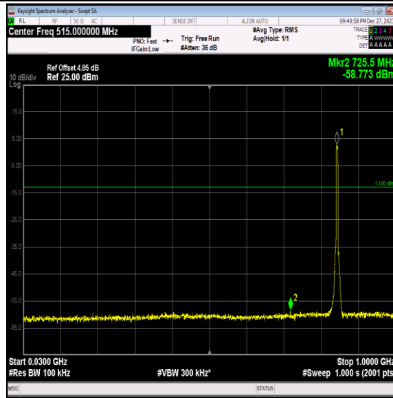
Band5-4233-2-30~1000MHz-PASS
