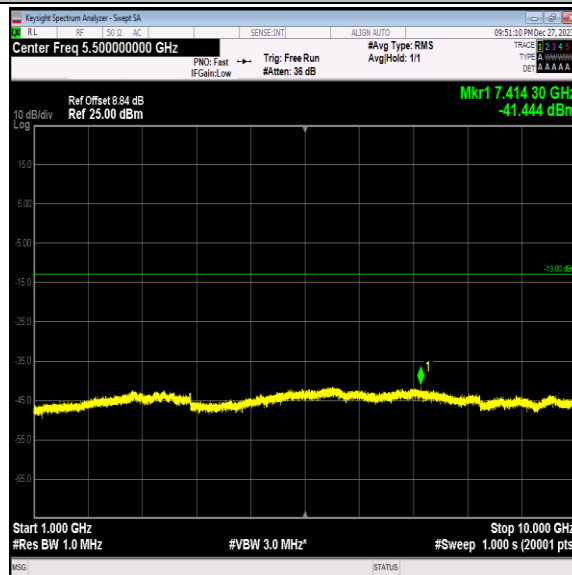
Band5-4233-5-1000~10000MHz-PASS
