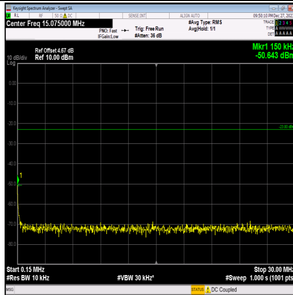
Band5-4182-5-0.15~30MHz-PASS
