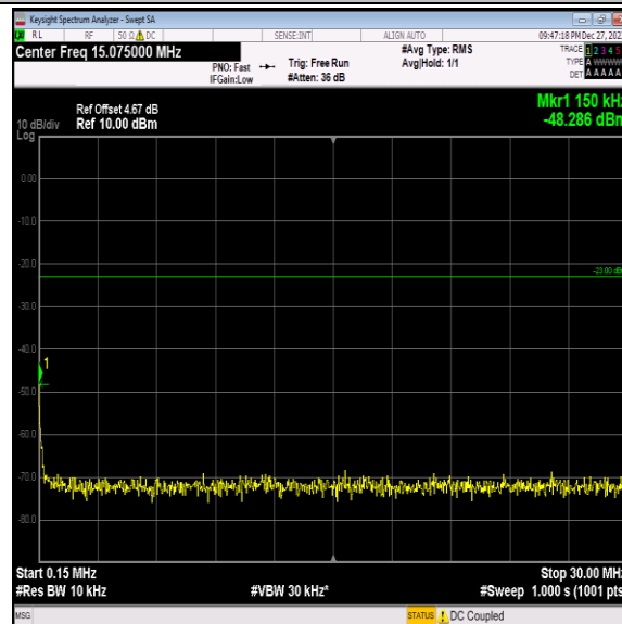
Band5-4182-4-0.15~30MHz-PASS
