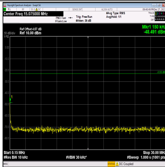
Band5-4233-2-0.15~30MHz-PASS
