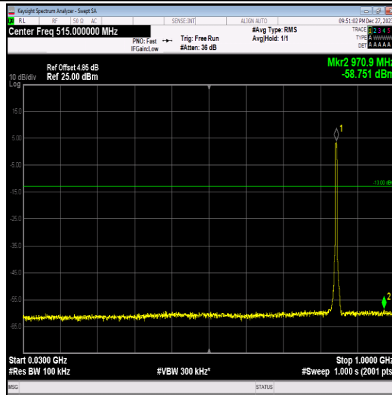
Band5-4233-5-30~1000MHz-PASS
