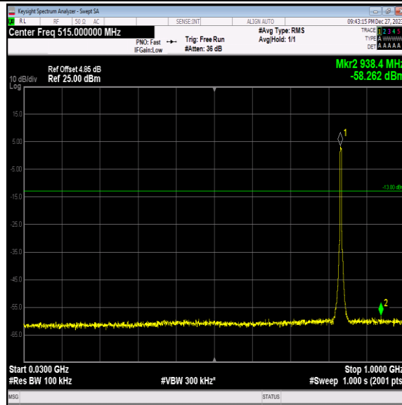
Band5-4182-3-30~1000MHz-PASS
