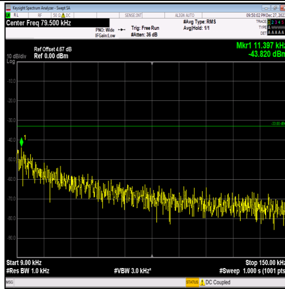
Band5-4182-5-0.009~0.15MHz-PASS
