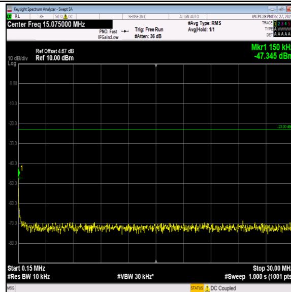
Band5-4182-2-0.15~30MHz-PASS
