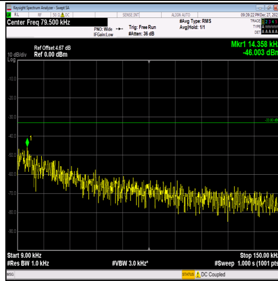
Band5-4182-2-0.009~0.15MHz-PASS
