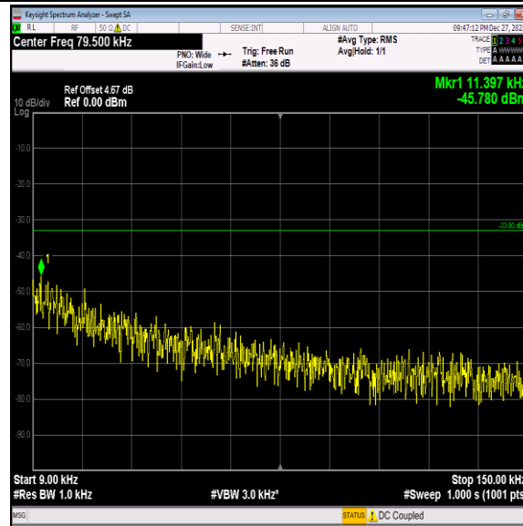
Band5-4182-4-0.009~0.15MHz-PASS
