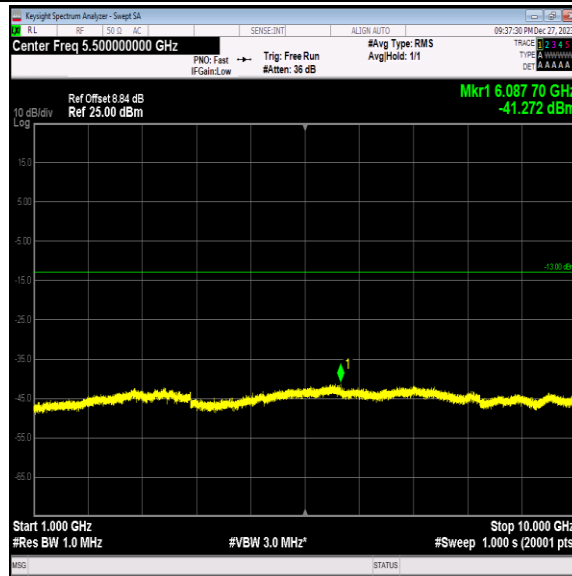
Band5-4233-1-1000~10000MHz-PASS
