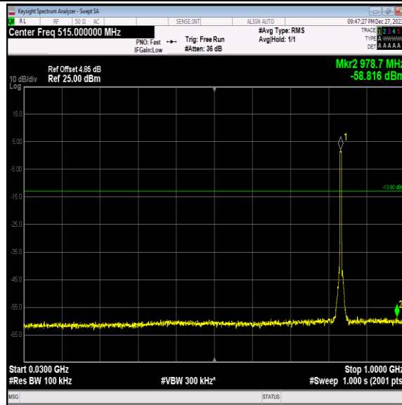
Band5-4182-4-30~1000MHz-PASS
