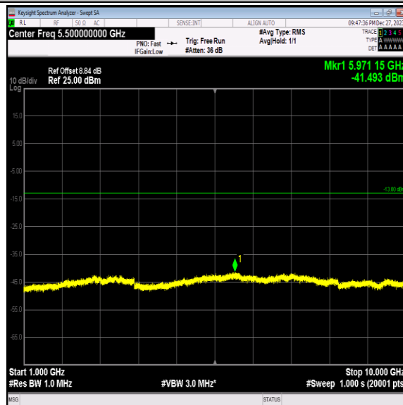
Band5-4182-4-1000~10000MHz-PASS
