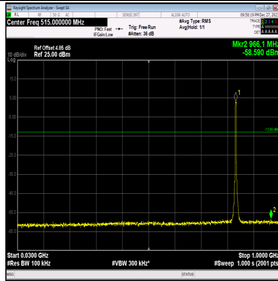
Band5-4182-5-30~1000MHz-PASS
