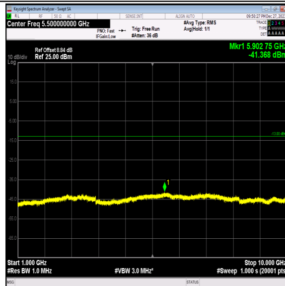
Band5-4182-5-1000~10000MHz-PASS
