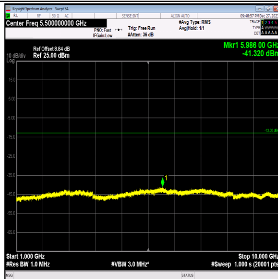
Band5-4233-4-1000~10000MHz-PASS
