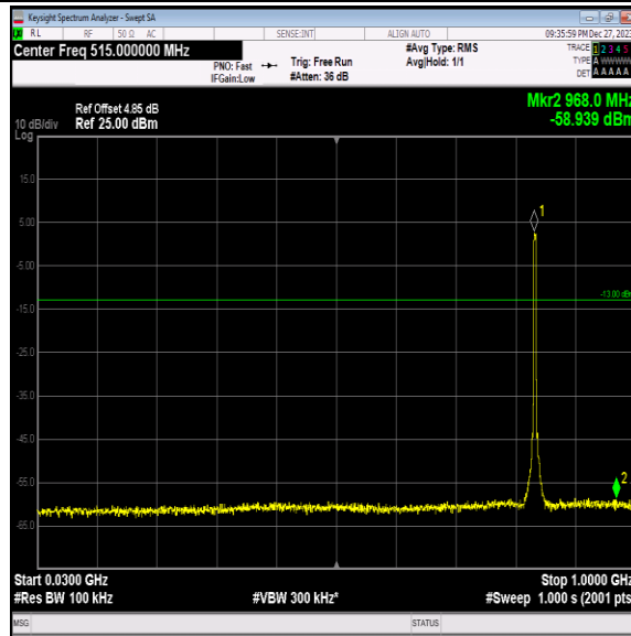
Band5-4182-1-30~1000MHz-PASS
