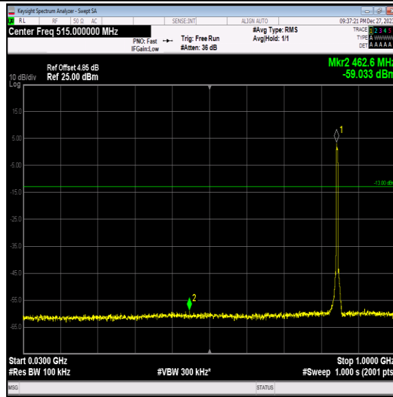
Band5-4233-1-30~1000MHz-PASS
