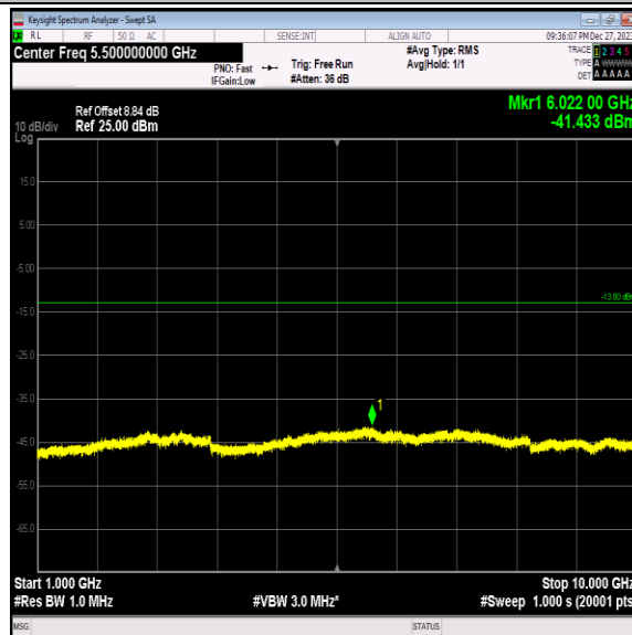
Band5-4182-1-1000~10000MHz-PASS
