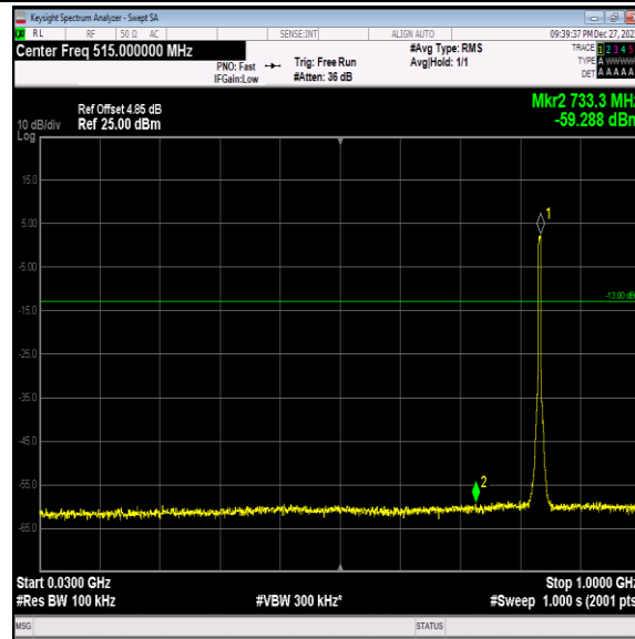
Band5-4182-2-30~1000MHz-PASS
