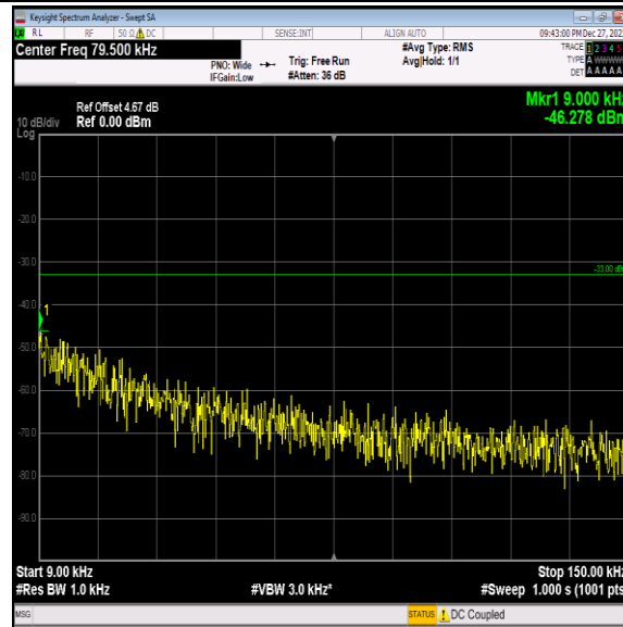
Band5-4182-3-0.009~0.15MHz-PASS
