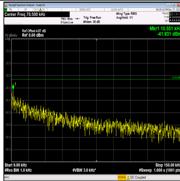
Band5-4182-1-0.009~0.15MHz-PASS
