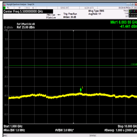
Band5-4182-2-1000~10000MHz-PASS
