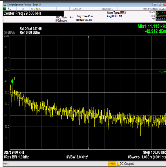
Band5-4233-5-0.009~0.15MHz-PASS
