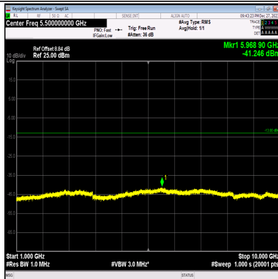
Band5-4182-3-1000~10000MHz-PASS
