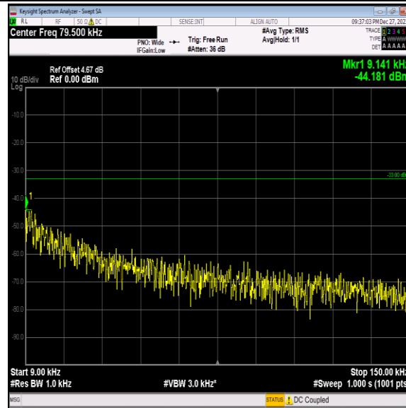
Band5-4233-1-0.009~0.15MHz-PASS
