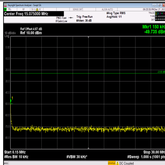
Band5-4182-1-0.15~30MHz-PASS
