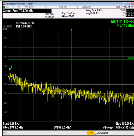
Band5-4233-2-0.009~0.15MHz-PASS
