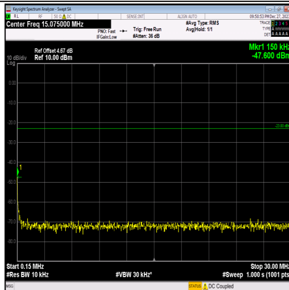
Band5-4233-5-0.15~30MHz-PASS
