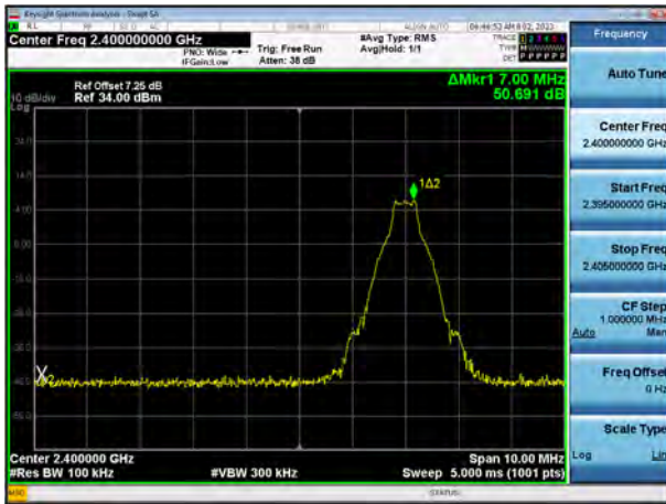
8DPSK(without hopping) Band Edge(CH.0)
