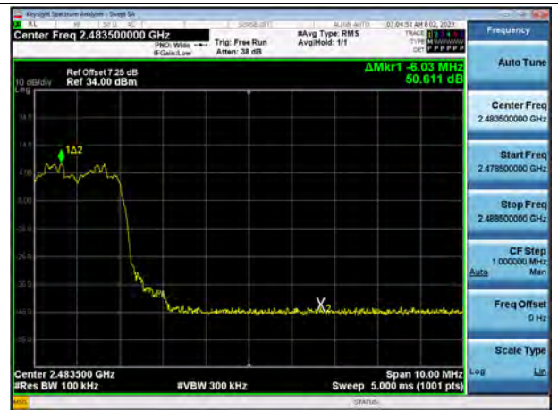
\pi/4 DQPSK (with hopping) Band Edge(CH.78)
