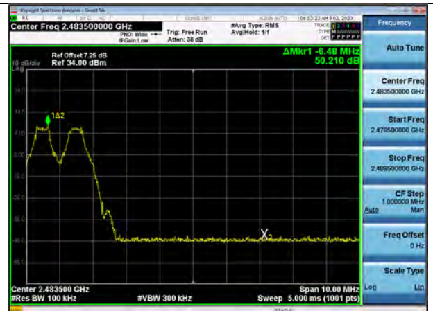
8DPSK(with hopping) Band Edge(CH.78)
