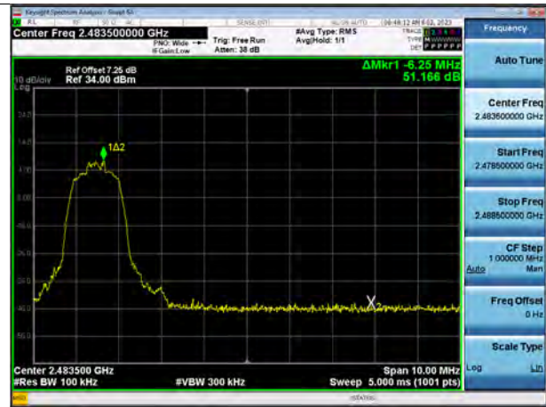
\pi/4 DQPSK (without hopping) Band Edge(CH.78)
