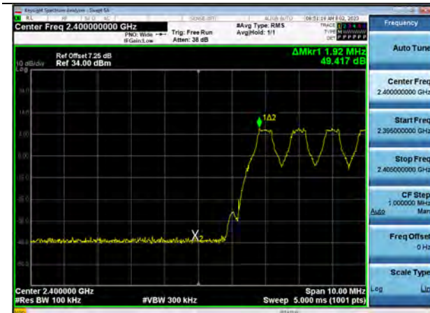
8DPSK(with hopping) Band Edge(CH.0)
