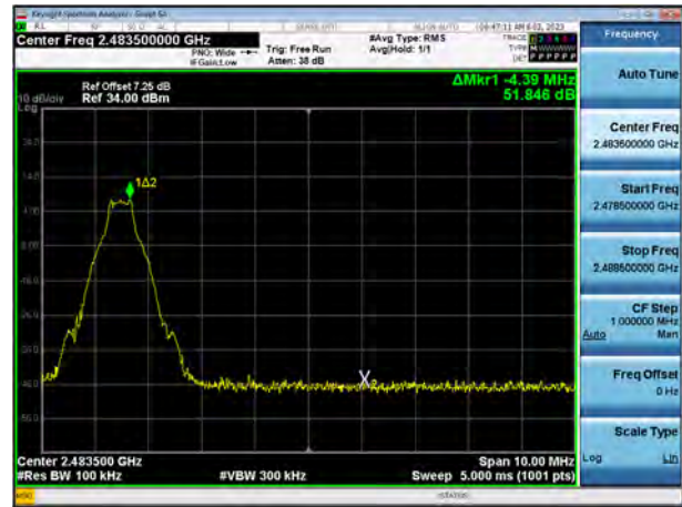
8DPSK(without hopping) Band Edge(CH.78)
