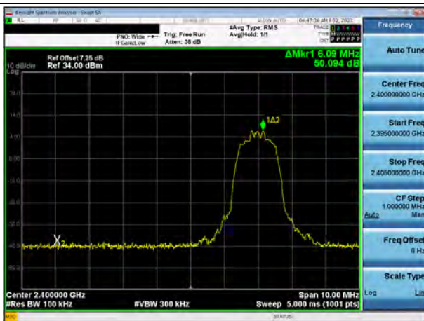
\pi/4 DQPSK(without hopping) Band Edge(CH.0)
