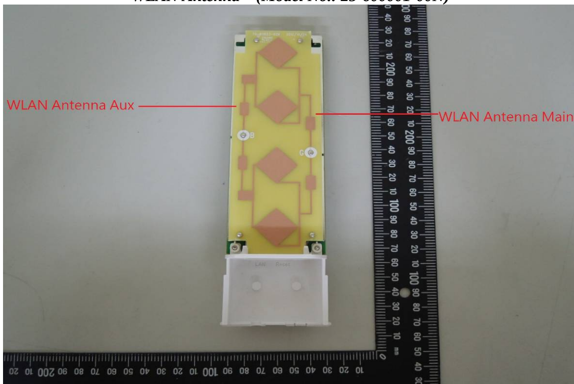
WLAN Antenna (Model No.: 25-600001-00N)
