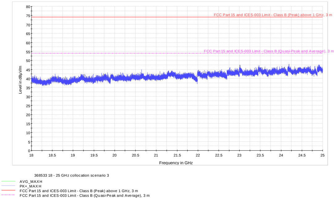
Figure 8.1-22: Radiated spurious emissions products from co-located transmitters within 18 - 25 GHz, Configuration 3
