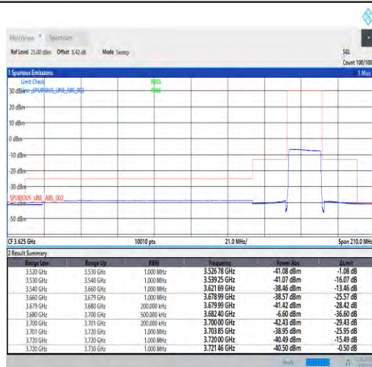
1-N48-30-20-H-3-CP-QPSK-Outer_Full-51@0-Ant 1-1--PASS-see graph
