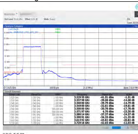
1-N48-30-30-L-3-DFT-PI2BPSK-Outer_Full-75@0-Ant1-1--PASS-see graph
