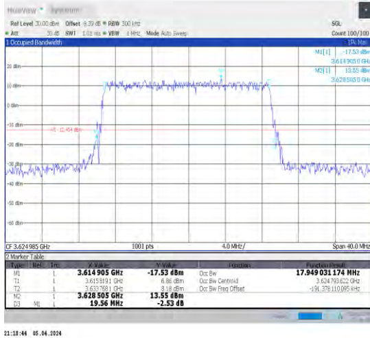
1-N48-30-20-M-3-DFT-16QAM-Outer_Full-50@0-Ant 1-17.949-19.560-≤20-PASS
