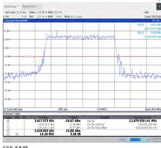
1-N48-30-15-M-1-DFT-QPSK-Outer_Full-36@0-Ant1 -12.88-14.280-<15-PASS
