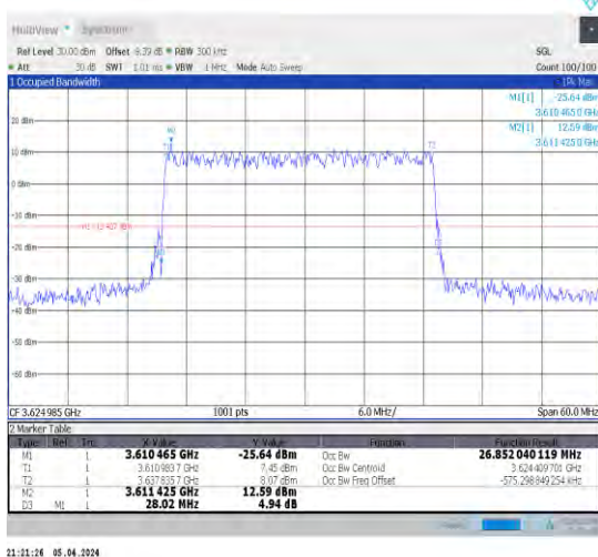
1-N48-30-30-M-4-DFT-64QAM-Outer_Full-75@0-Ant 1-26.852-28.020-≤30-PASS
