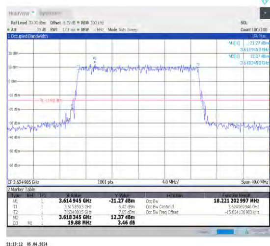
1-N48-30-20-M-6-CP-QPSK-Outer_Full-51@0-Ant1 18.221-19.880-≤20-PASS
