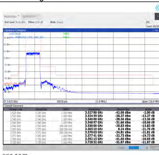
1-N48-30-20-L-3-DFT-PI2BPSK-Outer_Full-50@0-Ant1-1--PASS-see graph
