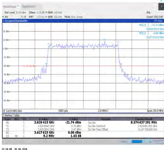
1-N48-30-10-M-9-CP-256QAM-Outer_Full-24@0-An t1-8.575-9.200-<10-PASS
