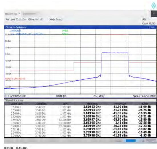
1-N48-30-40-H-6-CP-QPSK-Outer_Full-106@0-Ant1-1--PASS-see graph
