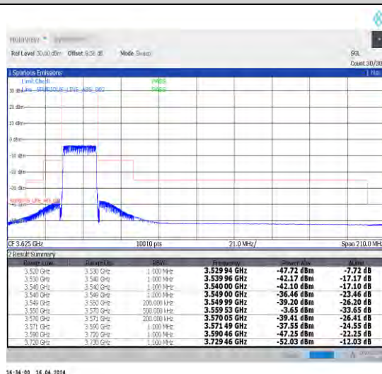
1-N48-30-20-L-6-CP-QPSK-Outer_Full-51@0-Ant1-1--PASS-see graph
