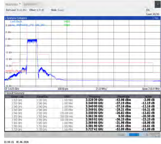
1-N48-30-15-L-3-DFT-PI2BPSK-Outer_Full-36@0-Ant1-1--PASS-see graph
