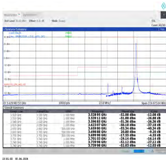
1-N48-30-40-H-5-CP-QPSK-Edge_1RB_Right-1@105-Ant1-1--PASS-see graph
