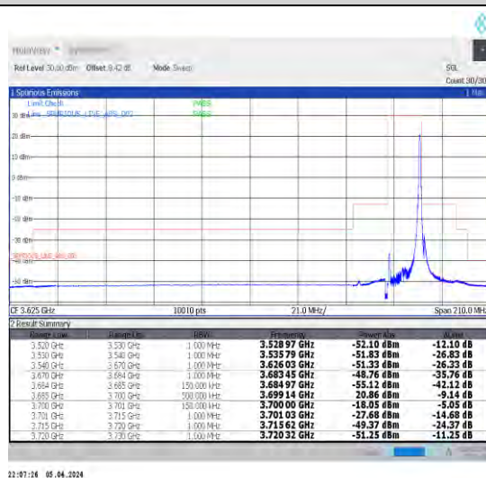
1-N48-30-15-H-5-CP-QPSK-Edge_1RB_Right-1@37-Ant1-1--PASS-see graph
