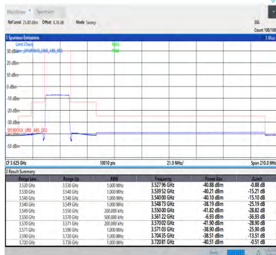
1-N48-30-20-L-3-CP-QPSK-Outer_Full-51@0-Ant 1-1--PASS-see graph
