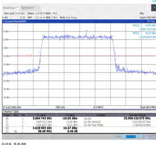
1-N48-30-40-M-3-DFT-16QAM-Outet_Full-100@0-Ant 1-35.996-38.480-≤40-PASS
