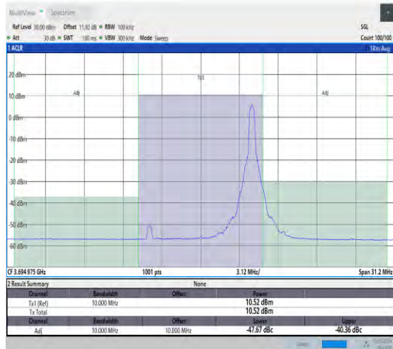
NTNV_N48_30_10_H_TID3_#1_-10_10
