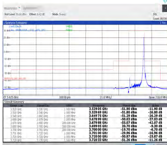
1-N48-30-20-H-5-CP-QPSK-Edge_1RB_Right-1@50-Ant1-1--PASS-see graph
