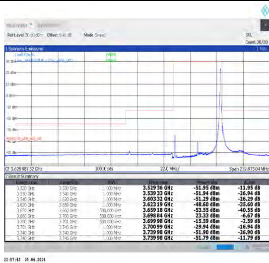
1-N48-30-40-H-2-DFT-PI2BPSK-Edge_1RB_Right-1@105-Ant1-1--PASS-see graph
