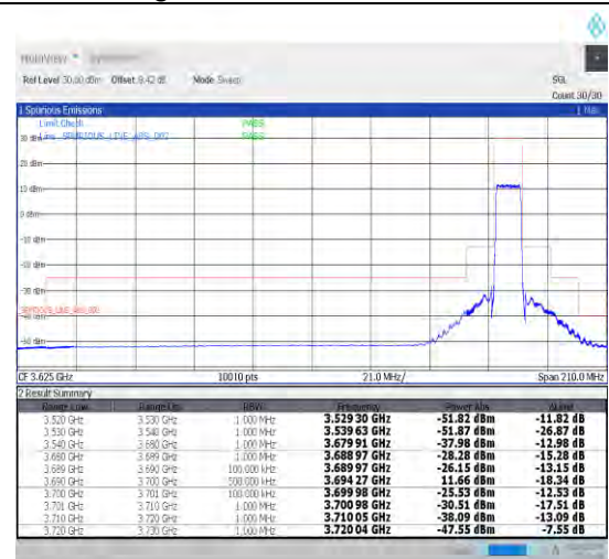
1-N48-30-10-H-3-DFT-PI2BPSK-Outer_Full-24@0-Ant1-1--PASS-see graph
