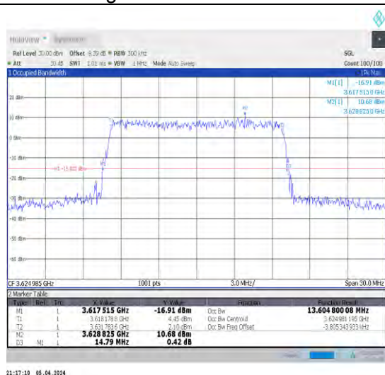
1-N48-30-15-M-9-CP-256QAM-Outer_Full-38@0-Ant 1-13.605-14.790≤15-PASS
