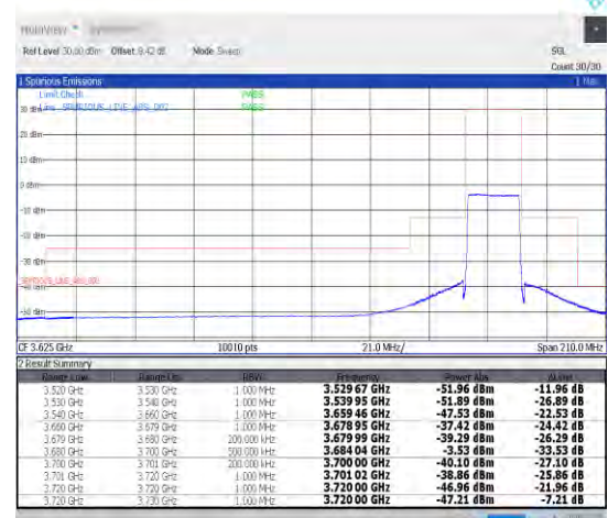
1-N48-30-20-H-6-CP-QPSK-Outer_Full-51@0-Ant1-1--PASS-see graph
