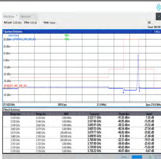
1-N48-30-20-H-2-CP-QPSK-Edge_1RB_Right-1@50-Ant1 -1--PASS-see graph
