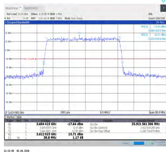
1-N48-30-40-M-4-DFT-64QAM-Outet_Full-100@0-Ant 1-35.922-38.800-≤40-PASS
