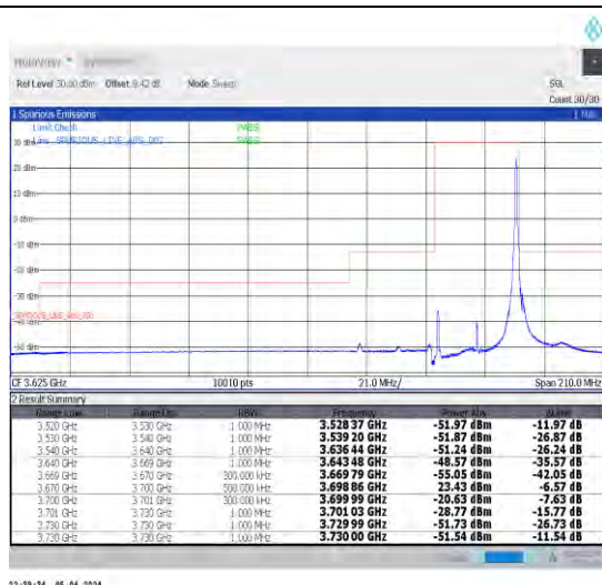
1-N48-30-30-H-2-DFT-PI2BPSK-Edge_1RB_Right-1@77-Ant1-1--PASS-see graph
