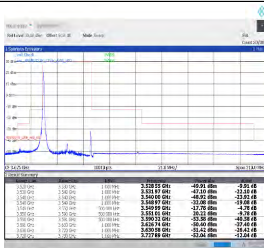
1-N48-30-40-L-1-DFT-PI2BPSK-Edge_1RB_Left-1@0-Ant1-1--PASS-see graph
