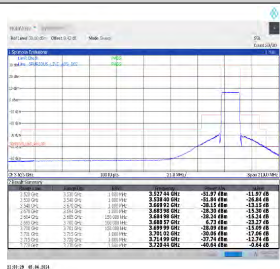
1-N48-30-15-H-6-CP-QPSK-Outer_Full-38@0-Ant1-1--PASS-see graph
