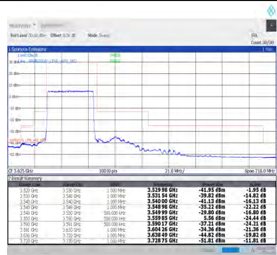
1-N48-30-40-L-3-DFT-PI2BPSK-Outer_Full-100@0-Ant1-1--PASS-see graph
