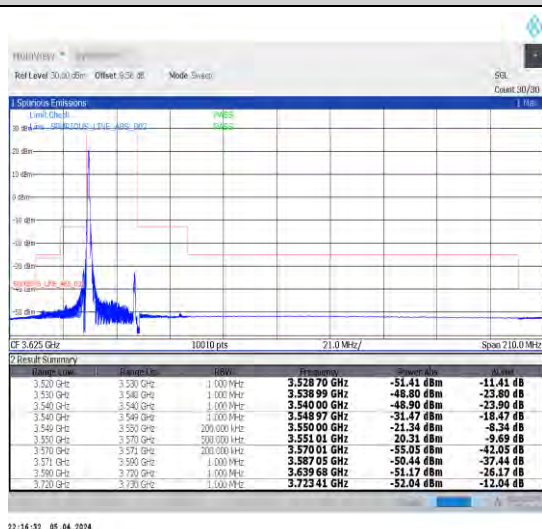
1-N48-30-20-L-4-CP-QPSK-Edge_1RB_Left-1@0-Ant1-1--PASS-see graph
