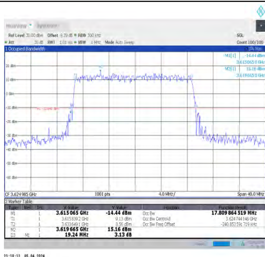
1-N48-30-20-M-1-DFT-QPSK-Outer_Full-50@0-Ant1 -17.81-19.240≤20-PASS
