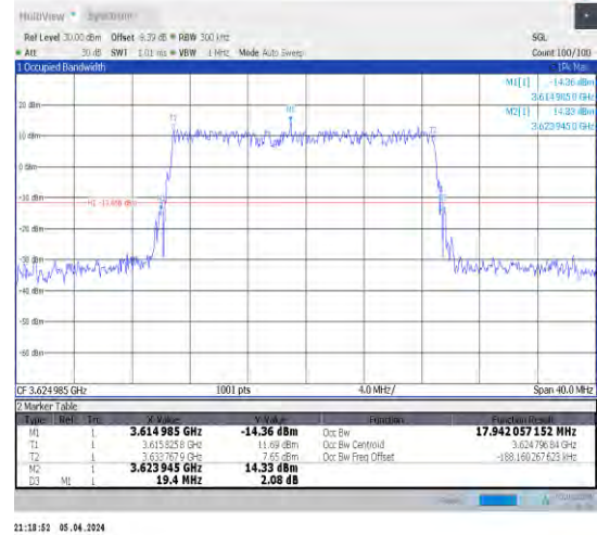
1-N48-30-20-M-4-DFT-64QAM-Outer_Full-50@0-Ant 1-17.942-19.400-≤20-PASS
