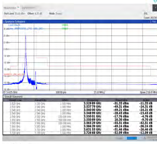
1-N48-30-15-L-4-CP-QPSK-Edge_1RB_Left-1@0-Ant1-1--PASS-see graph
