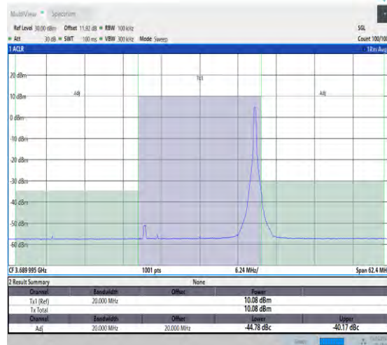
NTNV_N48_30_20_H_TID3_#1_-20_20
