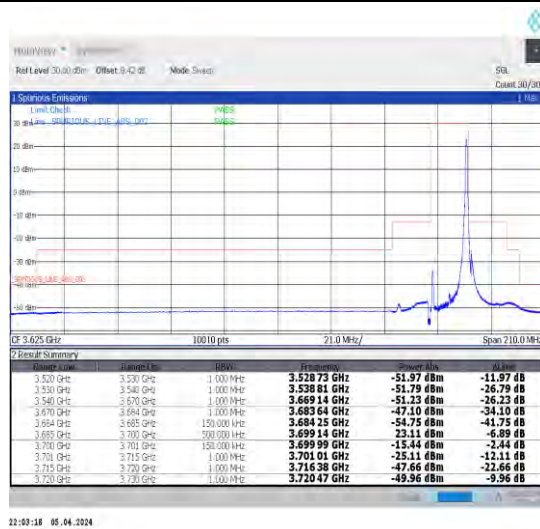
1-N48-30-15-H-2-DFT-PI2BPSK-Edge_1RB_Right-1@37-Ant1-1--PASS-see graph
