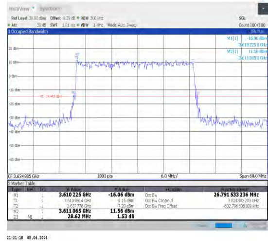
1-N48-30-30-M-3-DFT-16QAM-Outer_Full-75@0-Ant 1-26.793-28.620-≤30-PASS
