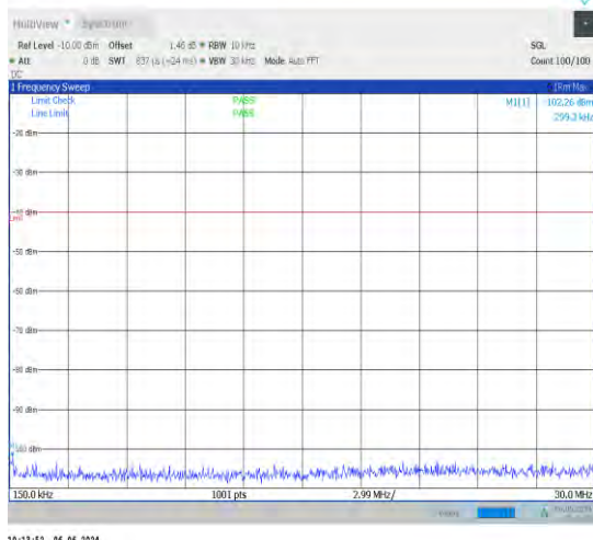
1-N48-30-40-M-1-DFT-PI2BPSK-Inner_1RB_Left-1 @1-0.15-30-Ant1-0.30--102.26--40-PASS
