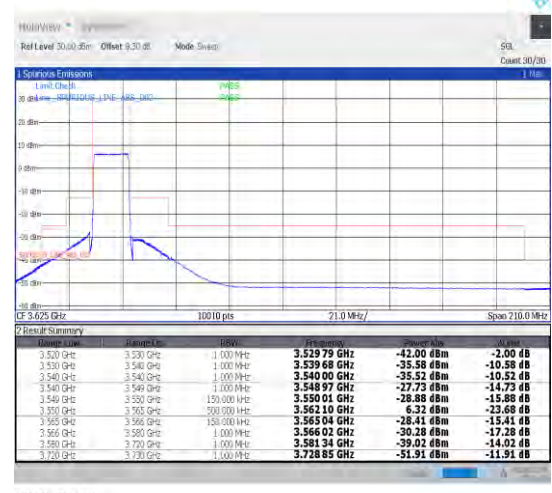
1-N48-30-15-L-6-CP-QPSK-Outer_Full-38@0-Ant1-1--PASS-see graph
