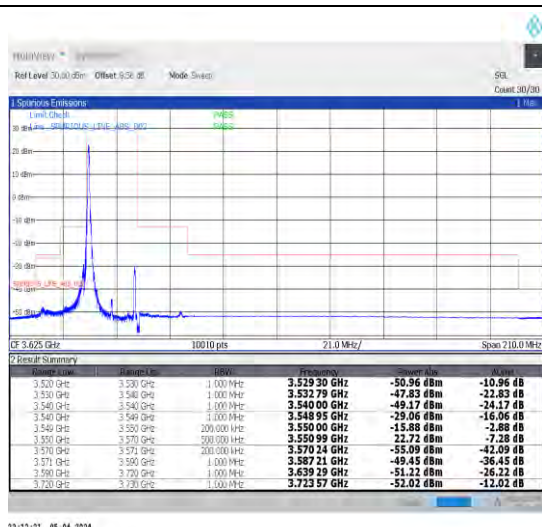
1-N48-30-20-L-1-DFT-PI2BPSK-Edge_1RB_Left-1@0-Ant1-1--PASS-see graph
