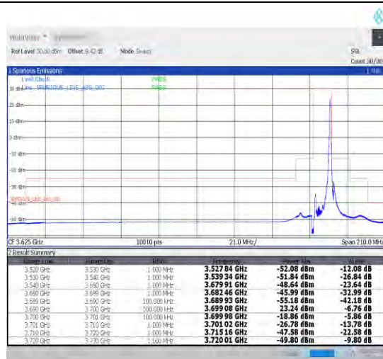
1-N48-30-10-H-2-DFT-PI2BPSK-Edge_1RB_Right-1@23-Ant1-1--PASS-see graph
