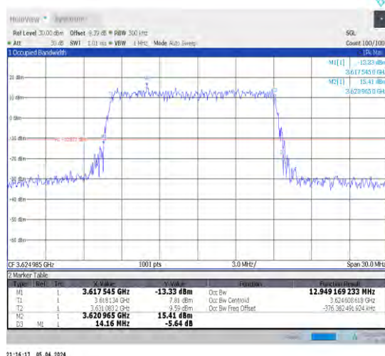
1-N48-30-15-M-3-DFT-16QAM-Outer_Full-36@0-Ant 1-12.949-14.160-<15-PASS
