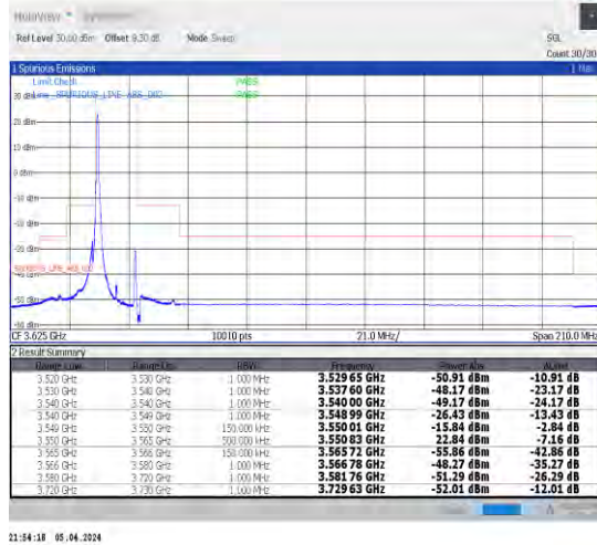
1-N48-30-15-L-1-DFT-PI2BPSK-Edge_1RB_Left-1@0-Ant1-1--PASS-see graph
