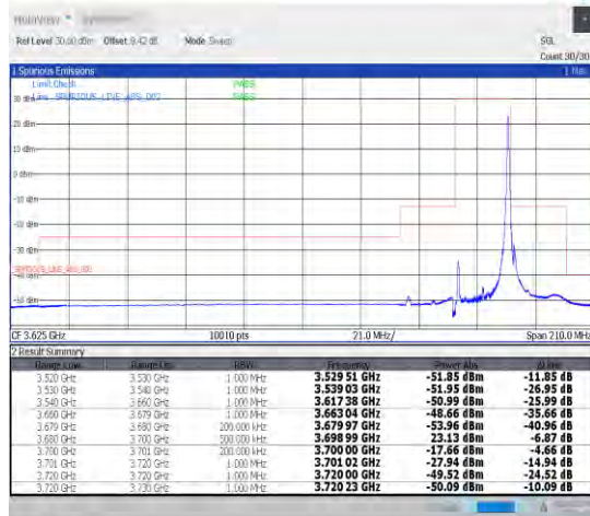
1-N48-30-20-H-2-DFT-PI2BPSK-Edge_1RB_Right-1@50-Ant1-1--PASS-see graph
