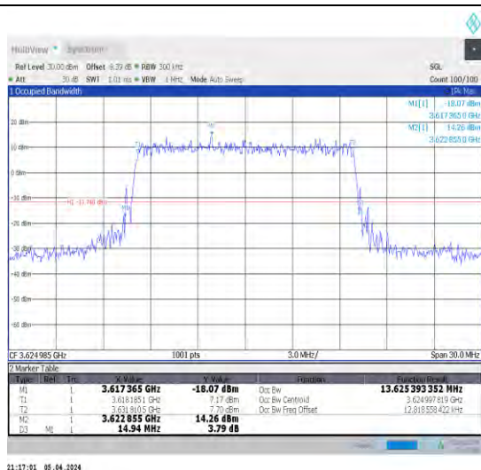
1-N48-30-15-M-8-CP-64QAM-Outer_Full-38@0-Ant 1-13.625-14.940≤15-PASS
