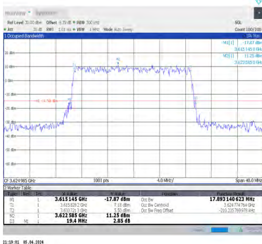
1-N48-30-20-M-5-DFT-256QAM-Outer_Full-50@0-A nt1-17.893-19.400-≤20-PASS
