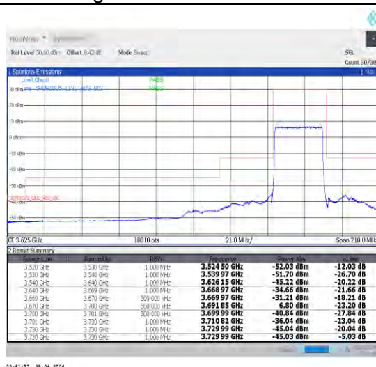
1-N48-30-30-H-3-DFT-PI2BPSK-Outer_Full-75@0-Ant1-1--PASS-see graph
