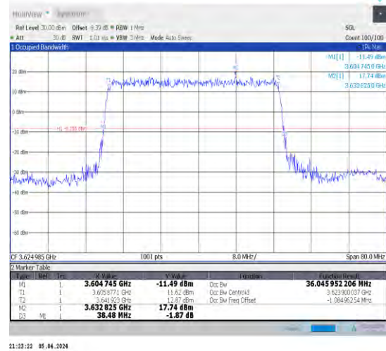
1-N48-30-40-M-2-DFT-PI2BPSK-Outet_Full-100@0-Ant 1-36.046-38.480-≤40-PASS
