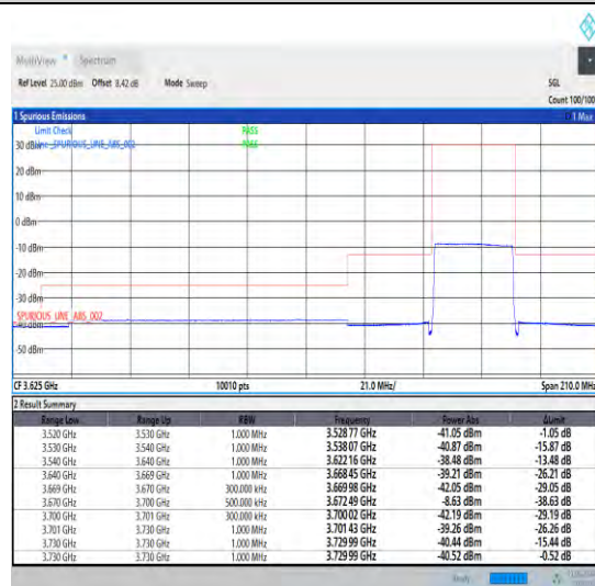
1-N48-30-30-H-3-CP-QPSK-Outer_Full-78@0-Ant1 1-1--PASS-see graph
