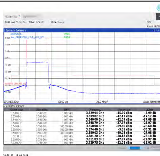
1-N48-30-30-L-6-CP-QPSK-Outer_Full-78@0-Ant1-1--PASS-see graph
