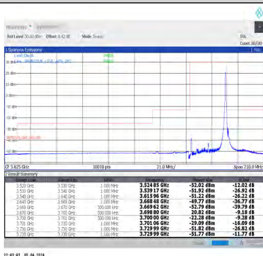
1-N48-30-30-H-5-CP-QPSK-Edge_1RB_Right-1@77-Ant1-1--PASS-see graph
