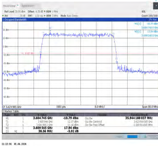
1-N48-30-40-M-1-DFT-QPSK-Outet_Full-100@0-Ant 1-35.944-38.560-≤40-PASS
