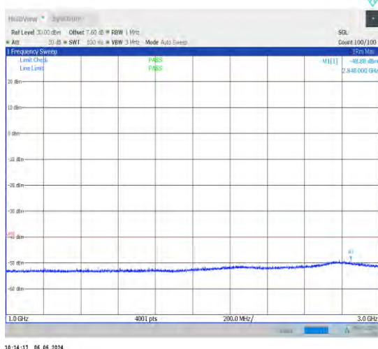
1-N48-30-40-M-1-DFT-PI2BPSK-Inner_1RB_Left-1 @1-1000-3000-Ant1-2848.00--48.88--40-PASS
