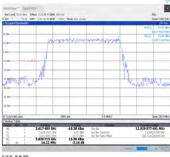
1-N48-30-15-M-2-DFT-PI2BPSK-Outer_Full-36@0-A nt1-12.929-14.220-<15-PASS
