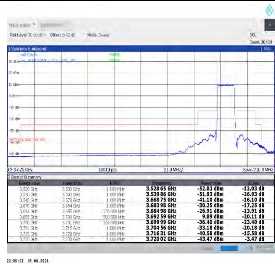
1-N48-30-15-H-3-DFT-PI2BPSK-Outer_Full-36@0-Ant1-1--PASS-see graph
