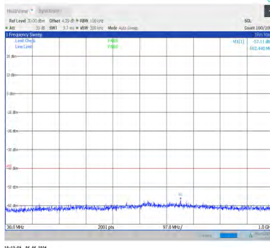
1-N48-30-40-M-1-DFT-PI2BPSK-Inner_1RB_Left-1 @1-30-1000-Ant1-662.44--57.11--40-PASS
