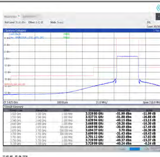
1-N48-30-30-H-6-CP-QPSK-Outer_Full-78@0-Ant1-1--PASS-see graph
