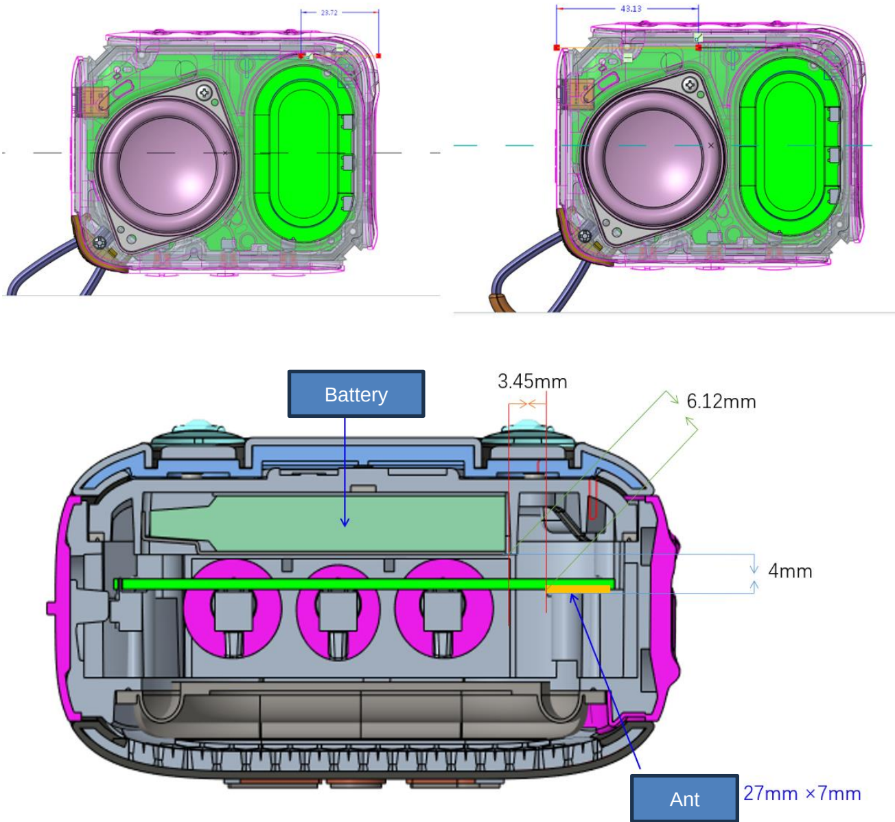
Antenna location diagram
