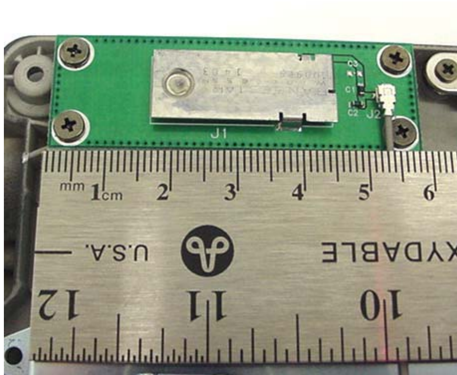
Spacing between Antennas (WLAN)
