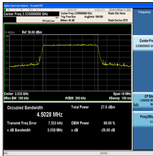
Band7-5MHz-16QAM-21100-25RB#0-4.5028
