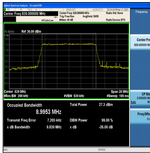
Band5-10MHz-QPSK-20450-50RB#0-8.9953
