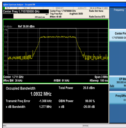
Band66-1.4MHz-QPSK-131979-6RB#0-1.0932
