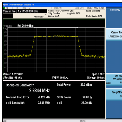
Band4-3MHz-QPSK-19965-15RB#0-2.6844
