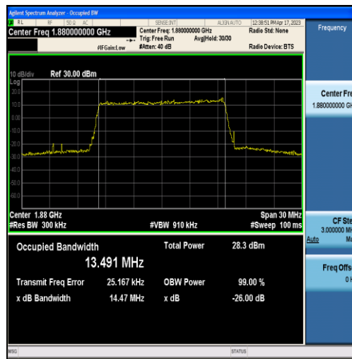
Band2-15MHz-16QAM-18900-75RB#0-13.491
