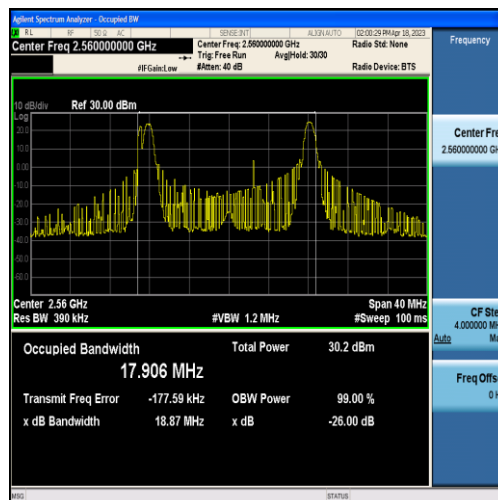
Band7-20MHz-16QAM-21350-60RB#0-17.906
