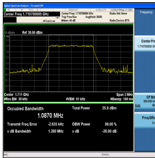
Band4-1.4MHz-16QAM-19957-6RB#0-1.0870
