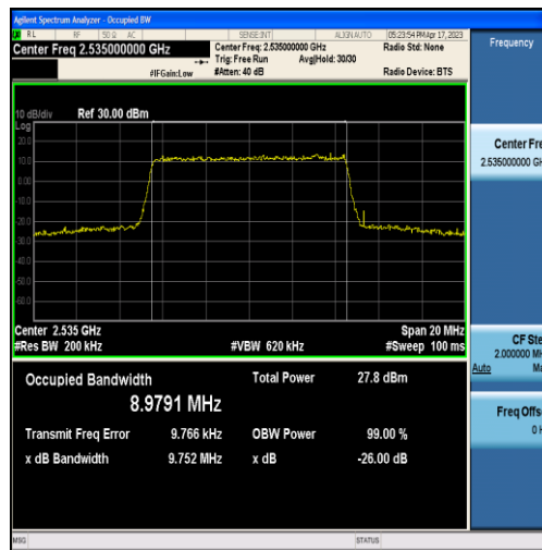
Band7-10MHz-16QAM-21100-50RB#0-8.9791
