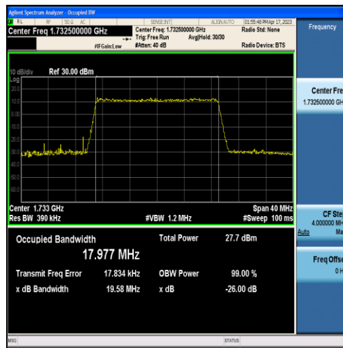
Band4-20MHz-16QAM-20175-100RB#0-17.977
