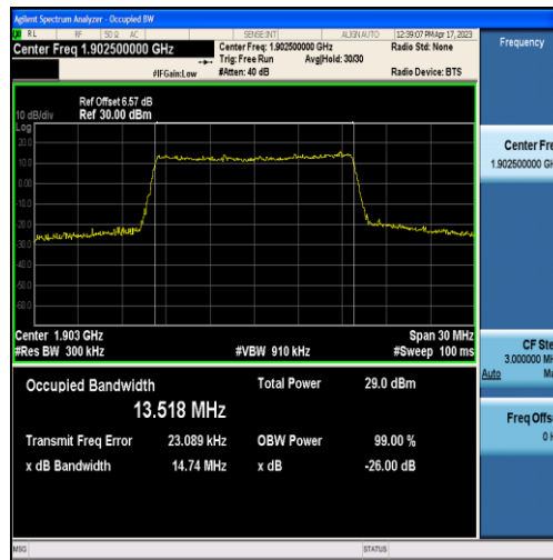
Band2-15MHz-QPSK-19125-75RB#0-13.518
