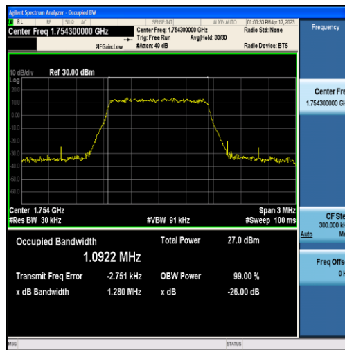
Band4-1.4MHz-QPSK-20393-6RB#0-1.0922
