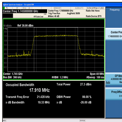
Band4-20MHz-16QAM-20300-100RB#0-17.910
