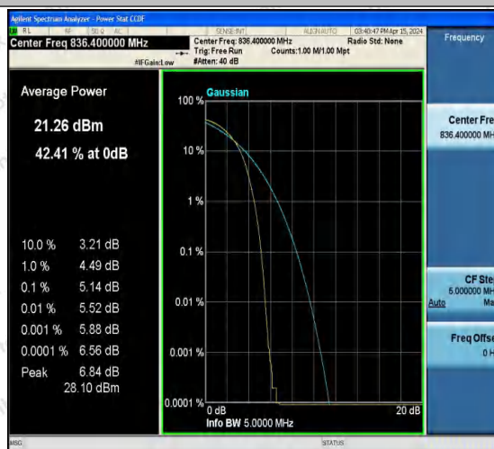
Band5-4182-4-PASS
