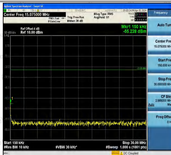
Band5-4182-5-0.15~30MHz-PASS
