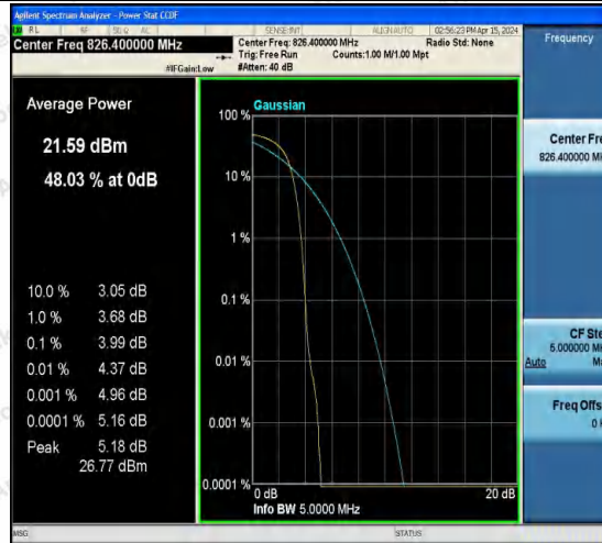
Band5-4132-4-PASS
