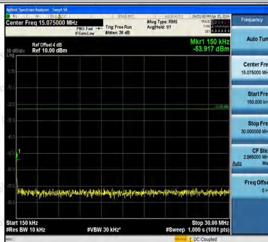
Band5-4182-1-0.15~30MHz-PASS
