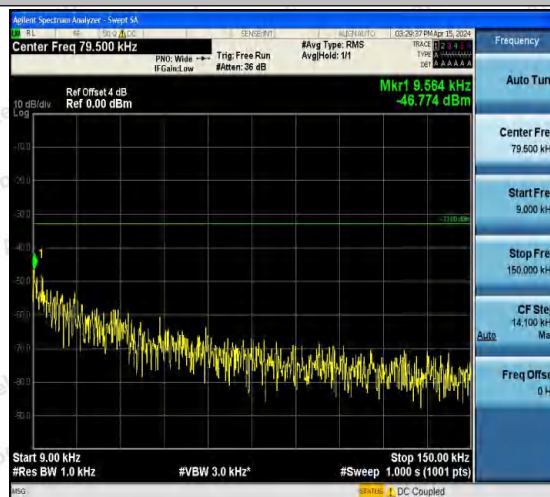
Band5-4233-4-0.009~0.15MHz-PASS
