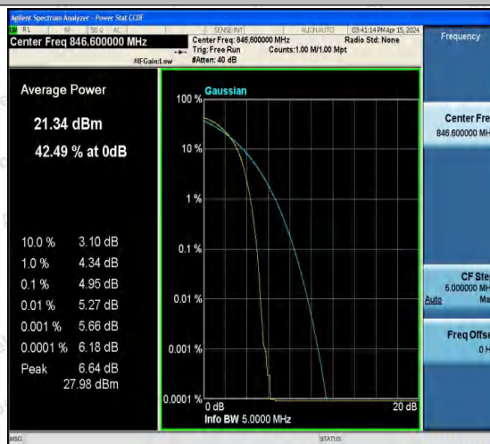
Band5-4233-4-PASS
