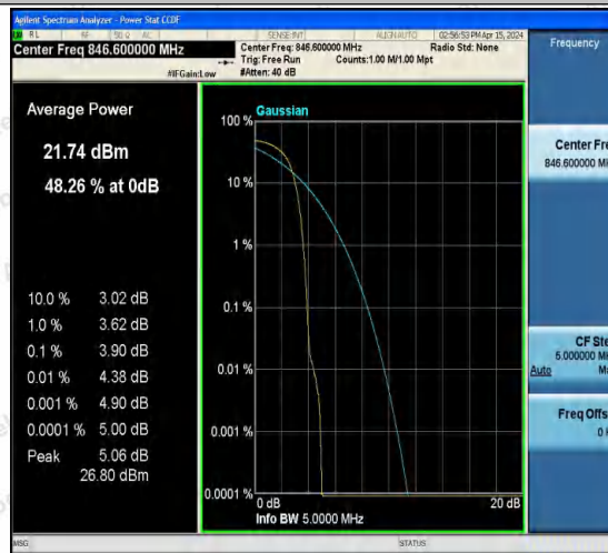
Band5-4233-4-PASS
