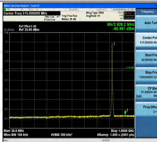
Band5-4132-5-30~1000MHz-PASS
