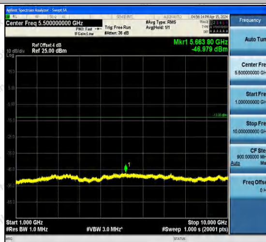
Band5-4182-3-1000~10000MHz-PASS
