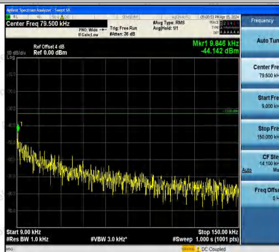
Band5-4233-5-0.009~0.15MHz-PASS
