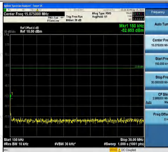
Band5-4132-3-0.15~30MHz-PASS
