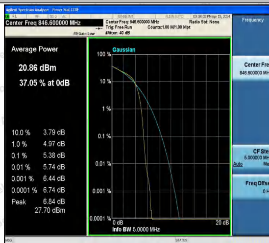
Band5-4233-2-PASS
