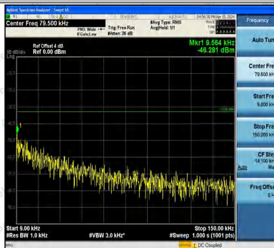
Band5-4233-3-0.009~0.15MHz-PASS
