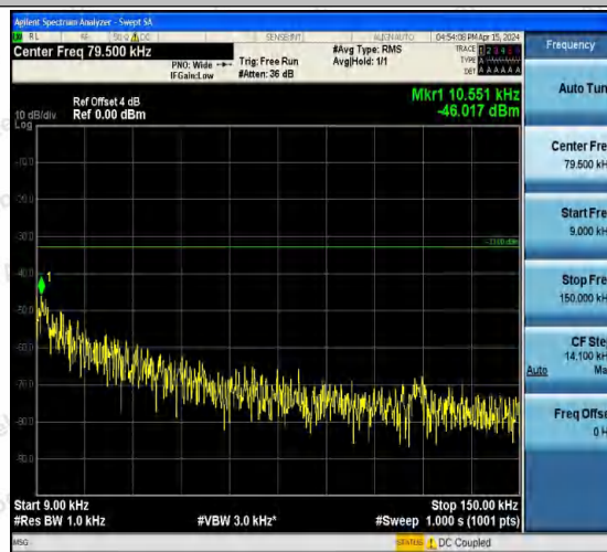
Band5-4233-2-0.009~0.15MHz-PASS
