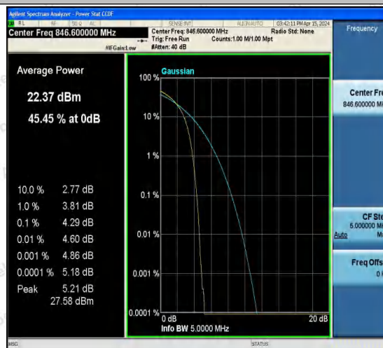
Band5-4233-5-PASS
