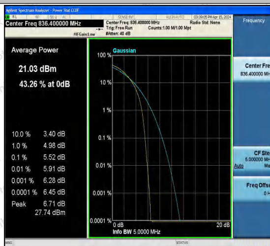
Band5-4182-3-PASS
