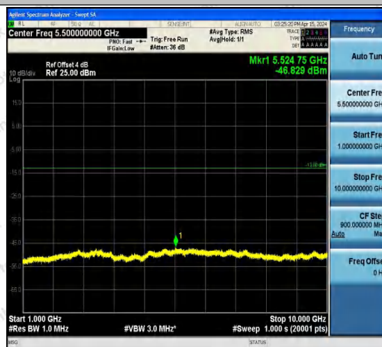
Band5-4182-2-1000~10000MHz-PASS
