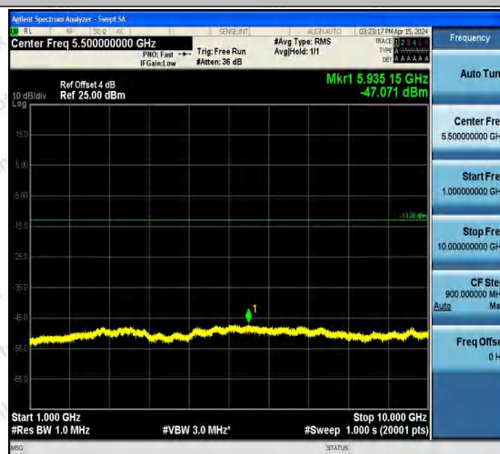
Band5-4182-1-1000~10000MHz-PASS
