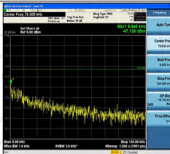
Band5-4233-1-0.009~0.15MHz-PASS
