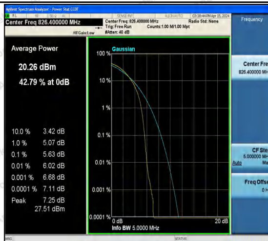
Band5-4132-3-PASS
