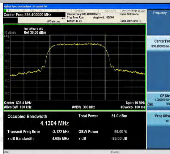
Band5-4182-5-PASS
