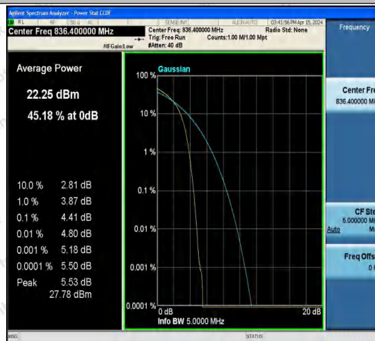
Band5-4182-5-PASS
