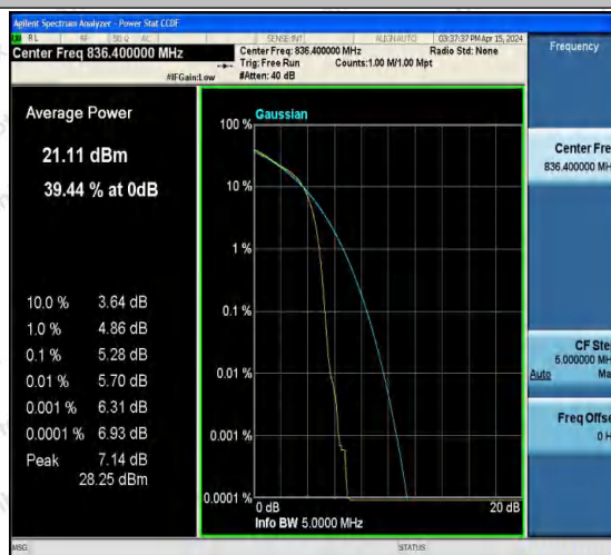
Band5-4182-2-PASS
