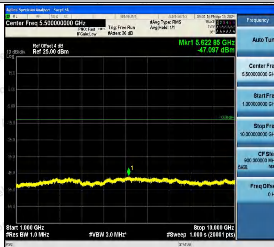
Band5-4233-5-1000~10000MHz-PASS
