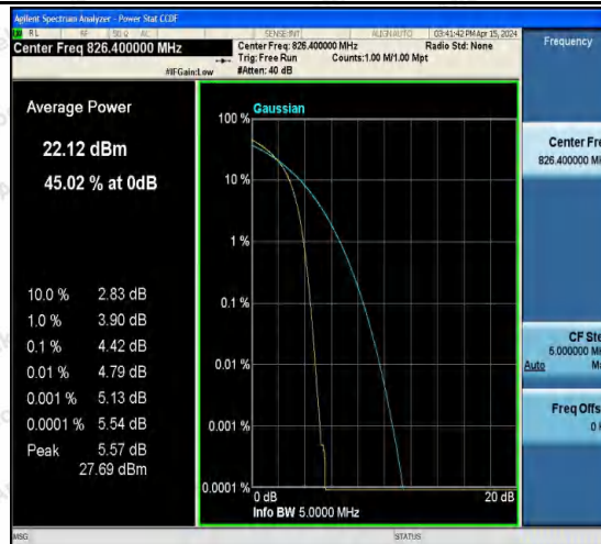
Band5-4132-5-PASS
