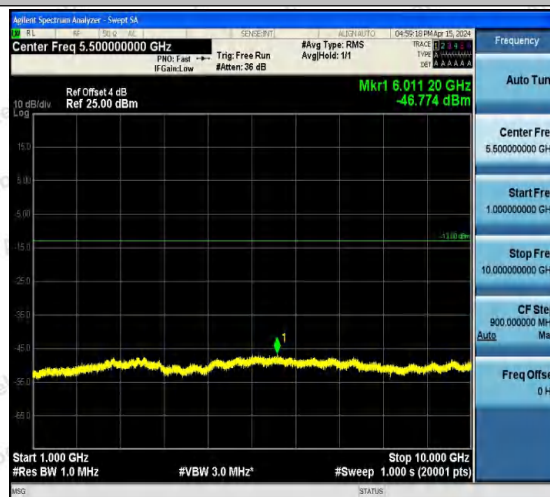
Band5-4233-4-1000~10000MHz-PASS
