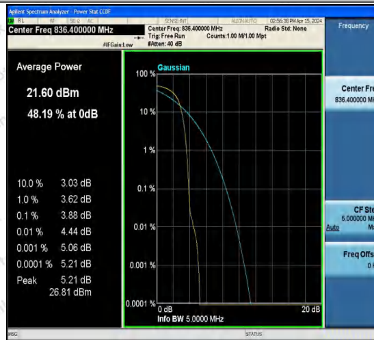
Band5-4182-4-PASS
