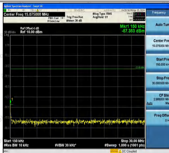
Band5-4182-3-0.15~30MHz-PASS
