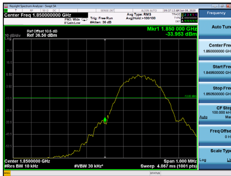
(Plot C:GPRS 1900 Channel = 512)
