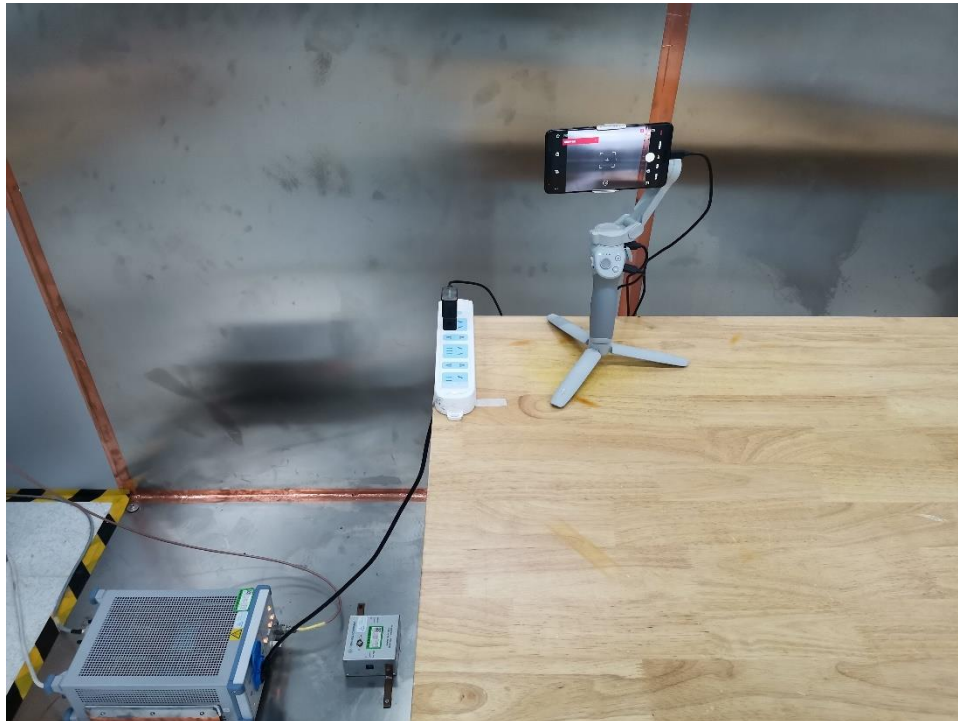
Photograph 1: Set-up photo for Conducted Emissions
