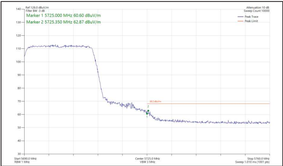
Figure 361 - 802.11ax HE20, SU, SISO, Core 0 - 5700 MHz Band Edge Frequency 5725 MHz
