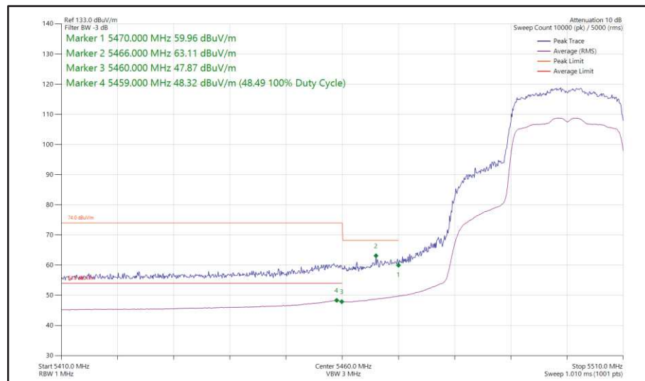
Figure 375 - 802.11ax HE20, SU, SISO, Core 1 - 5500 MHz Band Edge Frequency 5470 MHz
