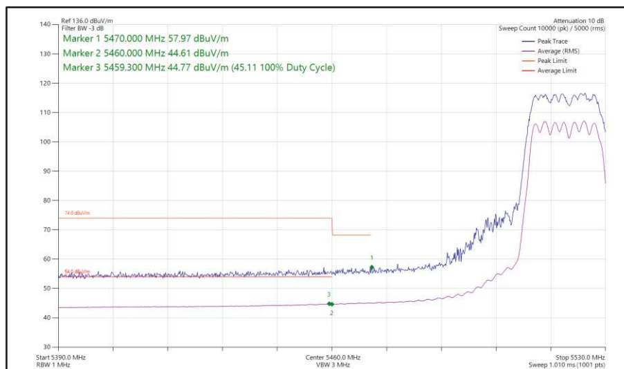
Figure 399- 802.11n HT20, CDD, Core 0-1 - 5520 MHz Band Edge Frequency 5470 MHz
