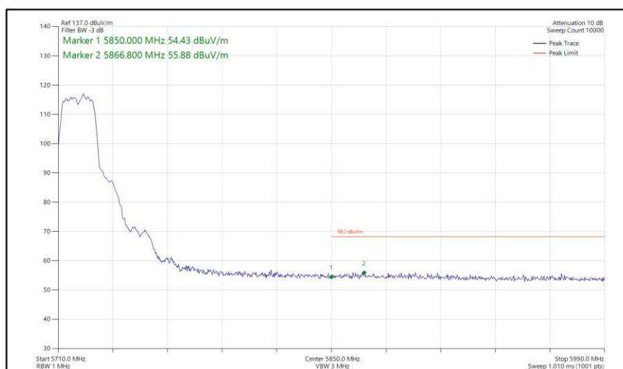
Figure 390- 802.11a, SISO, Core 1 - 5720 MHz Band Edge Frequency 5850 MHz
