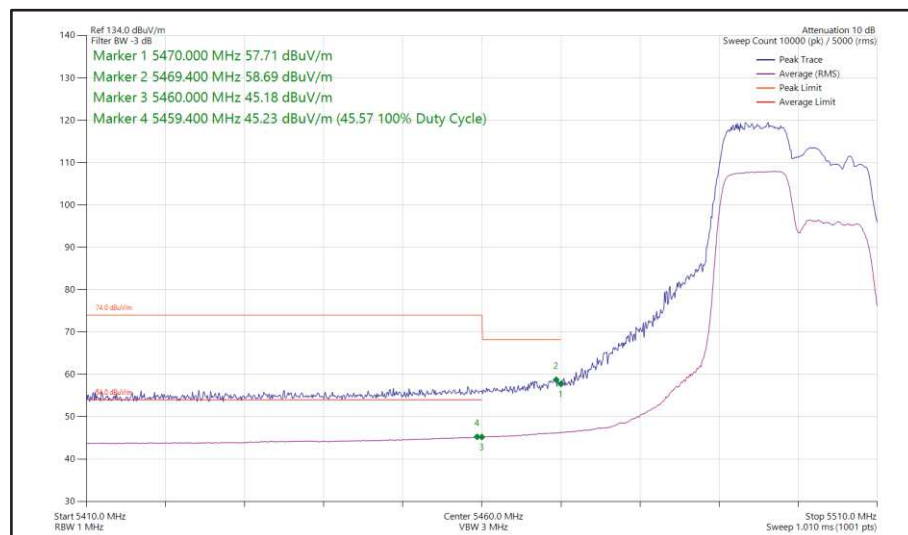
Figure 376 - 802.11ax HE20, RU 106-53, SISO, Core 1 - 5500 MHz Band Edge Frequency 5470 MHz
