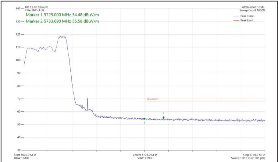
Figure 360 - 802.11ax HE20, RU 52-40, SISO, Core 0 - 5680 MHz Band Edge Frequency 5725 MHz
