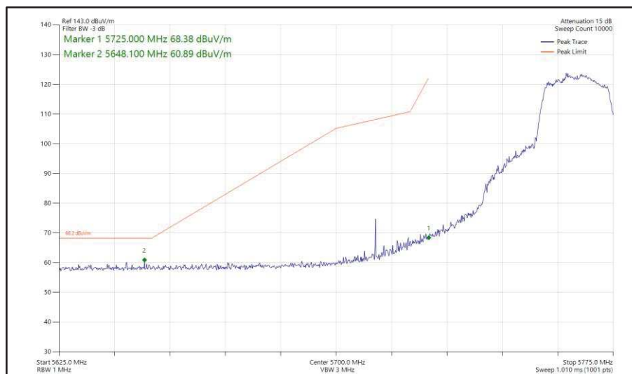
Figure 438 - 802.11ac VHT20, TxBF, Core 0 + Core 1 - 5765 MHz Band Edge Frequency 5725 MHz
