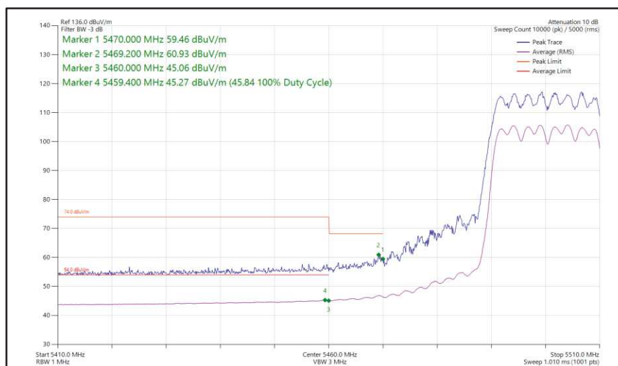
Figure 400- 802.11ax HE20, SU, CDD, Core 0-1 - 5500 MHz Band Edge Frequency 5470 MHz
