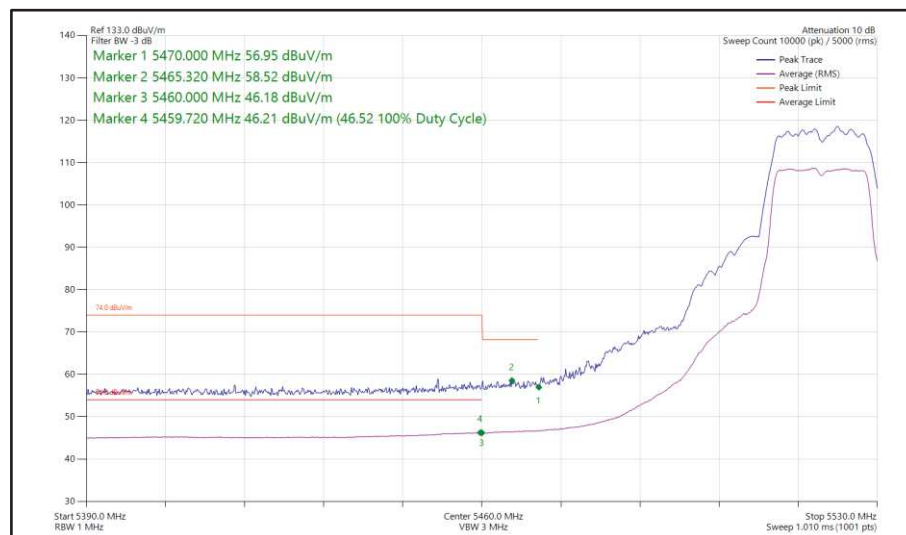
Figure 372 - 802.11a, SISO, Core 1 - 5520 MHz Band Edge Frequency 5470 MHz
