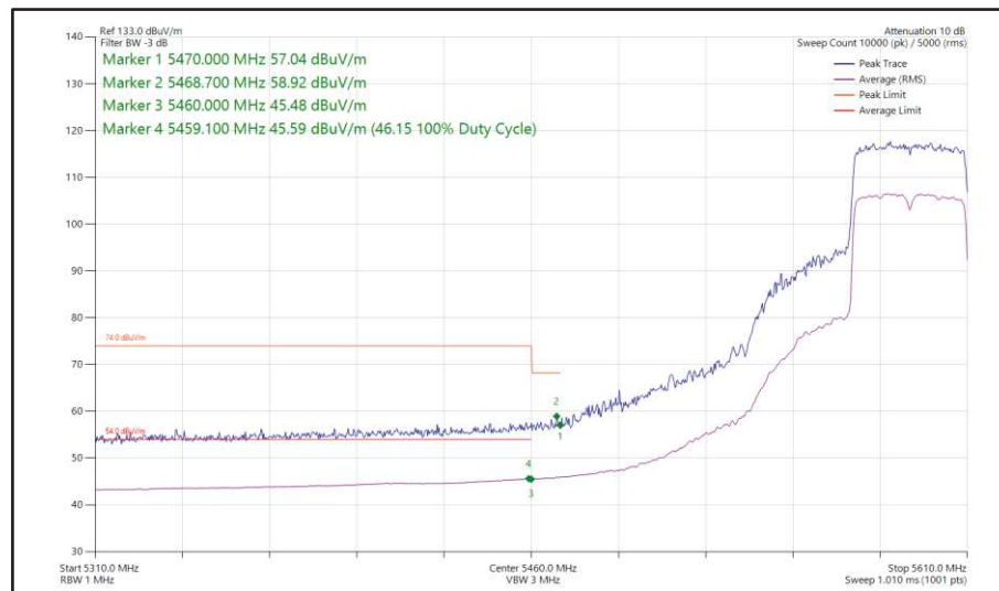
Figure 451 - 802.11ax HE40, SU, SISO, Core 0 - 5590 MHz Band Edge Frequency 5470 MHz
