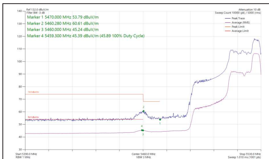
Figure 448 - 802.11ax HE40, RU 52-44, SISO, Core 0 - 5510 MHz Band Edge Frequency 5470 MHz
