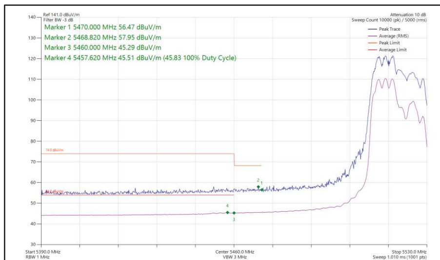
Figure 420 - 802.11ax HE20, RU 106-53, SDM, Core 0-1 - 5520 MHz Band Edge Frequency 5470 MHz
