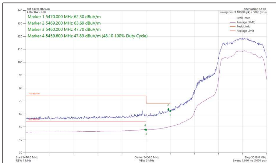
Figure 435 - 802.11ac VHT20, TxBF, Core 0 + Core 1 - 5500 MHz Band Edge Frequency 5470 MHz
