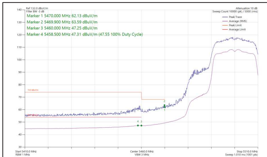
Figure 373 - 802.11n HT20, SISO, Core 1 - 5500 MHz Band Edge Frequency 5470 MHz
