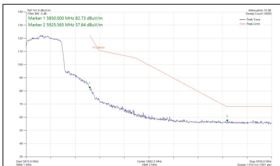
Figure 433 - 802.11ax HE20, SU, SDM, Core 0-1 - 5825 MHz Band Edge Frequency 5850 MHz
