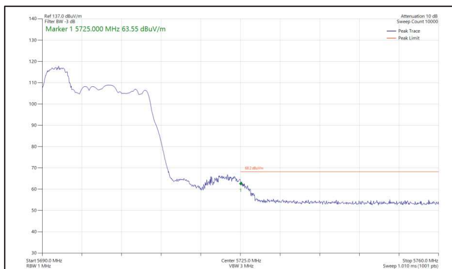
Figure 389- 802.11ax HE20, RU 52-37, SISO, Core 1 - 5700 MHz Band Edge Frequency 5725 MHz
