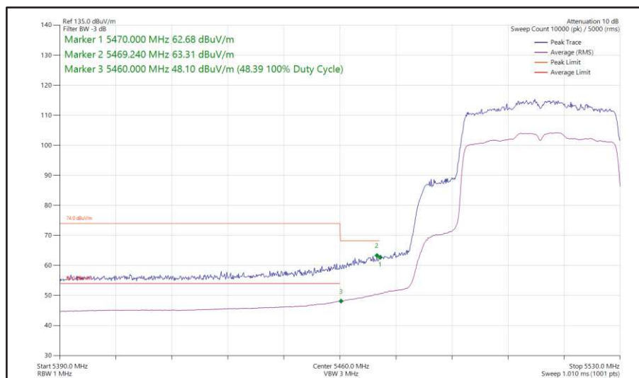
Figure 447 - 802.11ax HE40, SU, SISO, Core 0 - 5510 MHz Band Edge Frequency 5470 MHz
