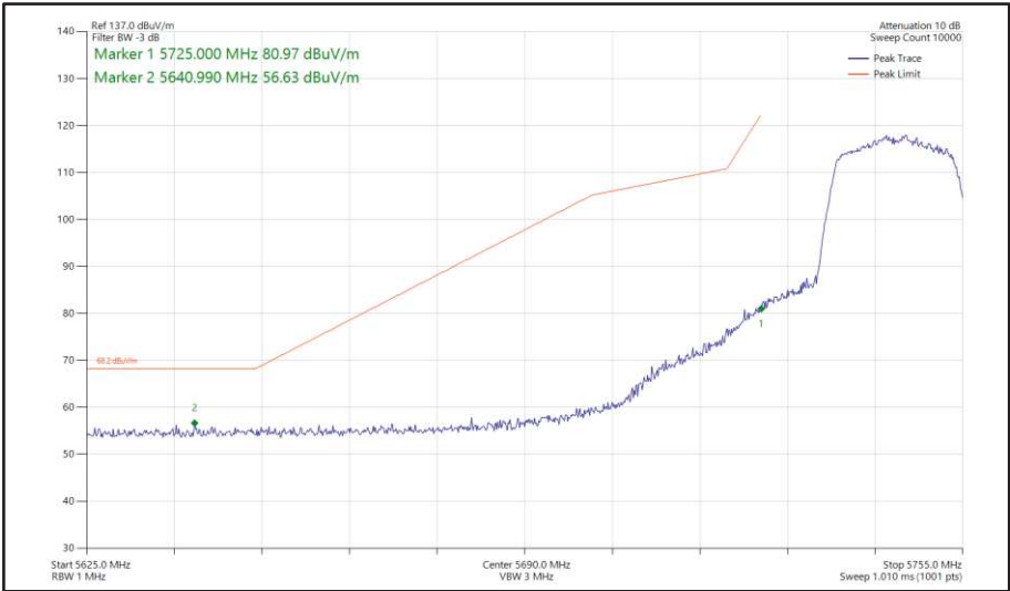
Figure 379 - 802.11n HT20, SISO, Core 1 - 5745 MHz Band Edge Frequency 5725 MHz
