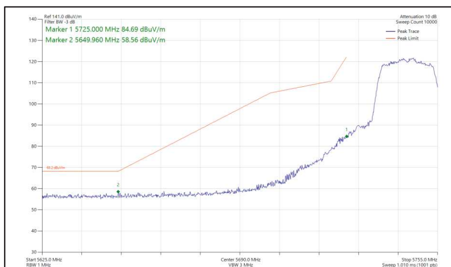
Figure 421 - 802.11n HT20, SDM, Core 0-1 - 5745 MHz Band Edge Frequency 5725 MHz
