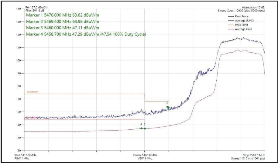
Figure 346 - 802.11n HT20, SISO, Core 0 - 5500 MHz Band Edge Frequency 5470 MHz
