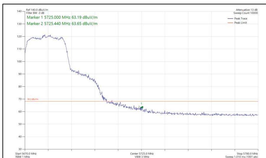
Figure 439 - 802.11ac VHT20, TxBF, Core 0 + Core 1 - 5680 MHz Band Edge Frequency 5725 MHz
