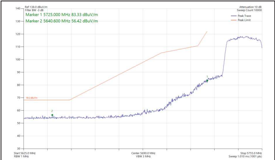
Figure 380 - 802.11ax HE20, SU, SISO, Core 1 - 5745 MHz Band Edge Frequency 5725 MHz
