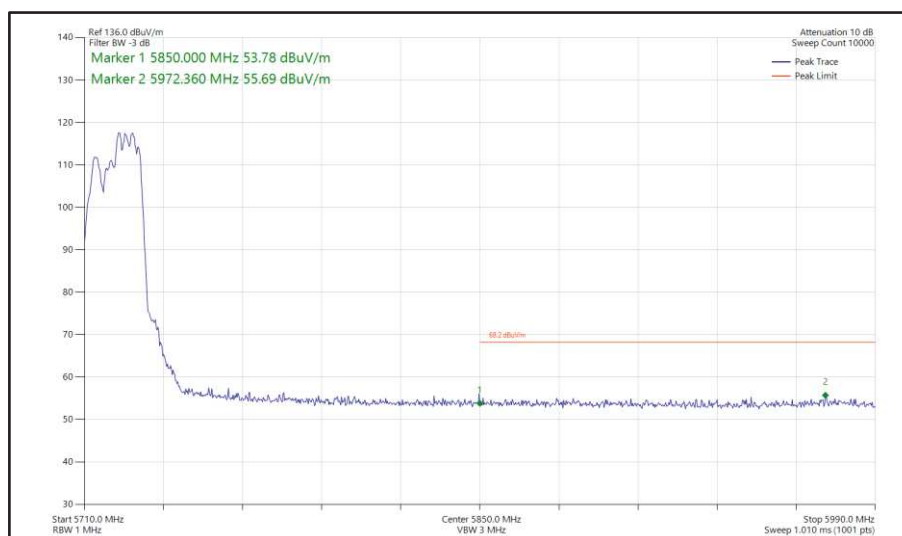
Figure 432 - 802.11ax HE20, RU 106-54, SDM, Core 0-1 - 5720 MHz Band Edge Frequency 5850 MHz
