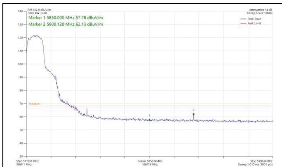
Figure 441 - 802.11ac VHT20, TxBF, Core 0 + Core 1 - 5720 MHz Band Edge Frequency 5850 MHz
