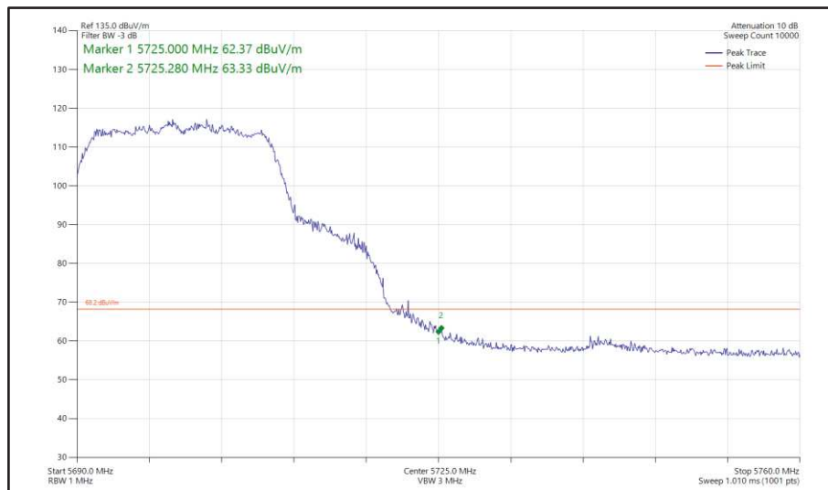
Figure 440 - 802.11ac VHT20, TxBF, Core 0 + Core 1 - 5700 MHz Band Edge Frequency 5725 MHz
