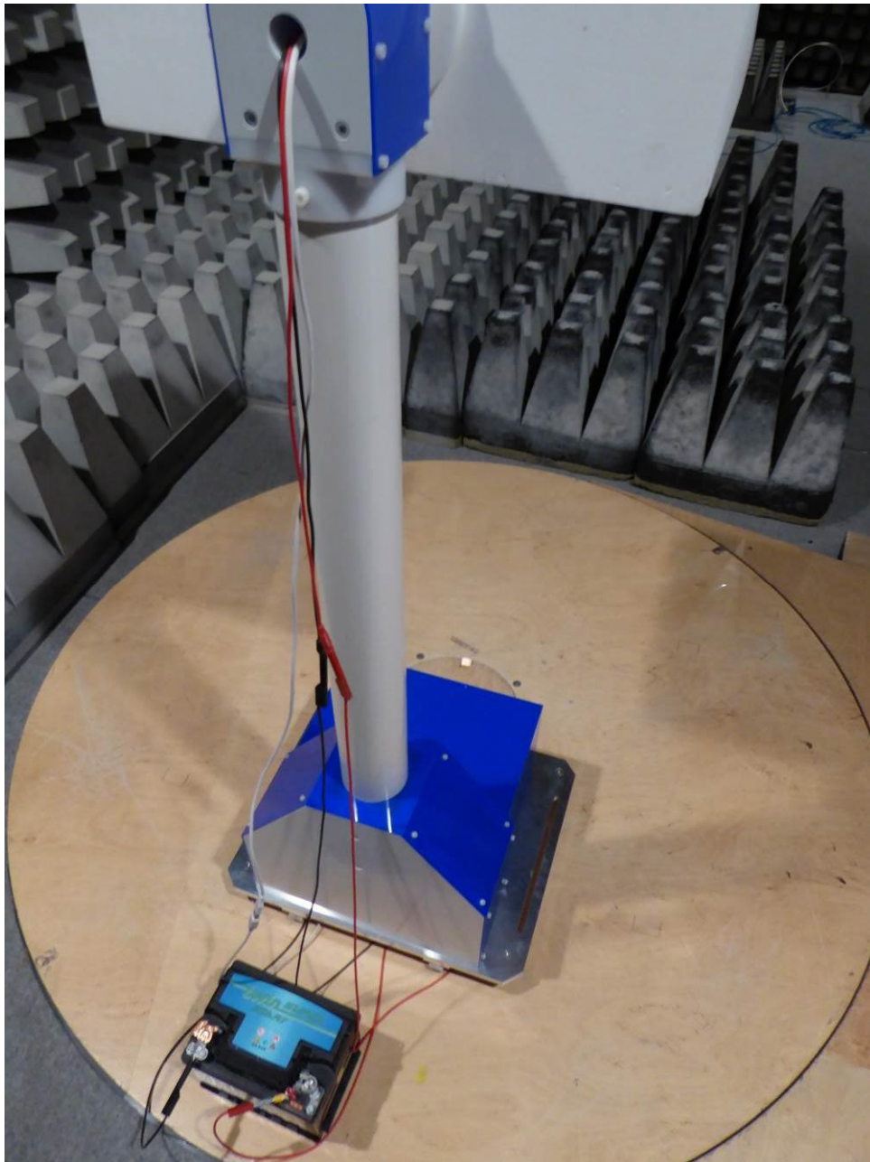
160090_40.jpg: Test setup - Radiated emission > 1 GHz (fully anechoic chamber)
