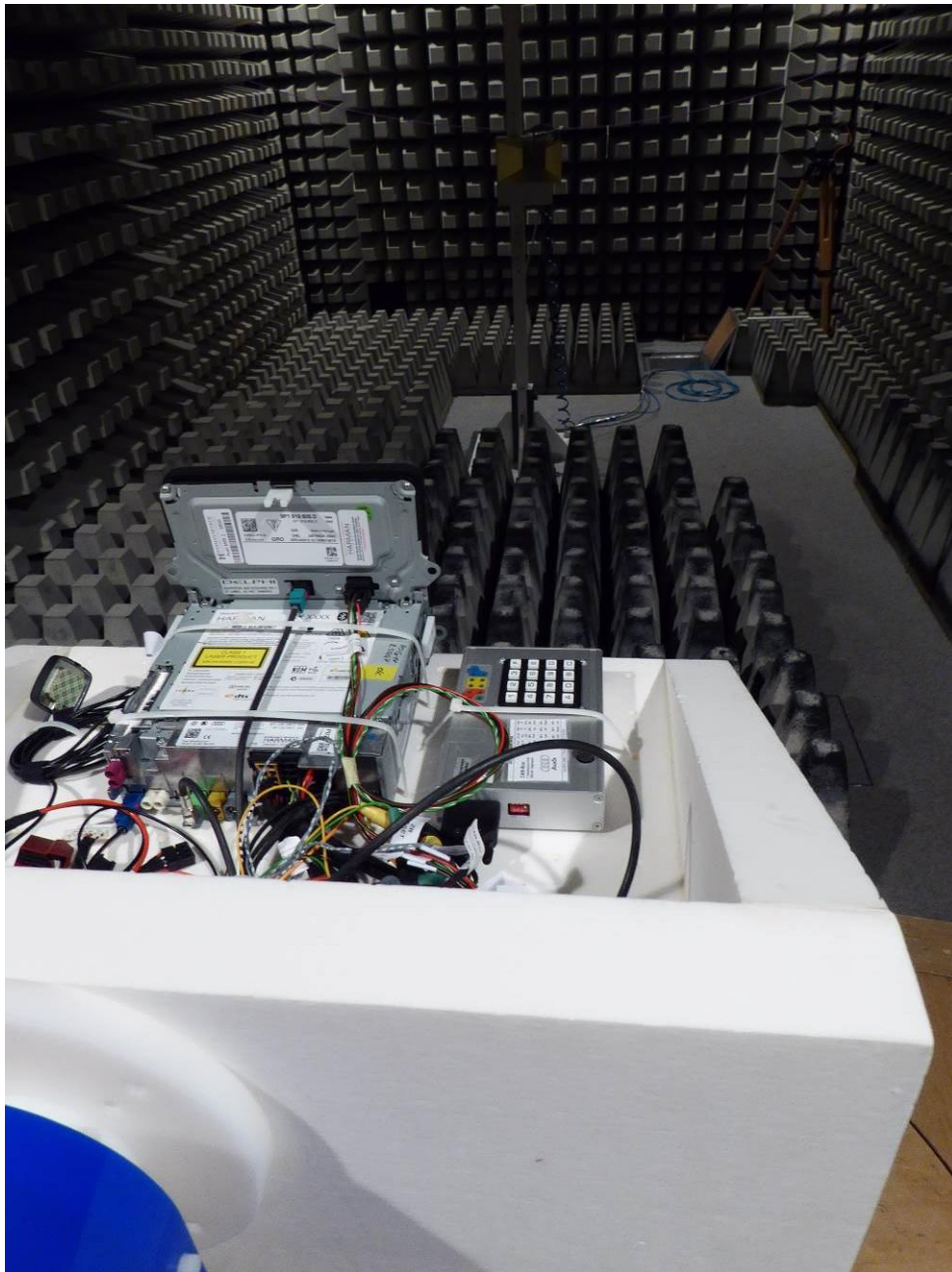
160090_41.jpg: Test setup - Radiated emission > 1 GHz (fully anechoic chamber)
