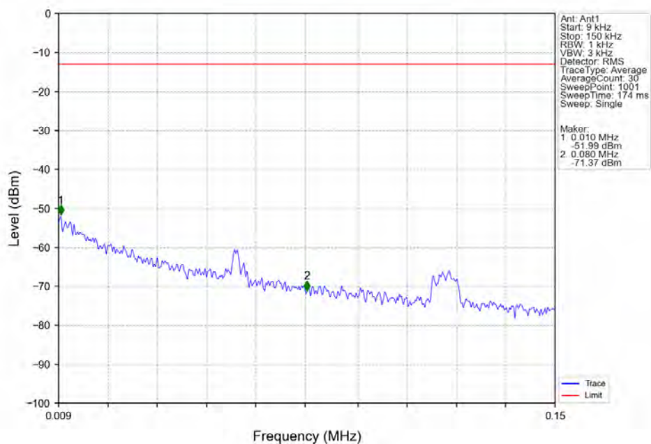
Band66 10MHz 16QAM HCH 1775MHz RB 1 0 NTV
