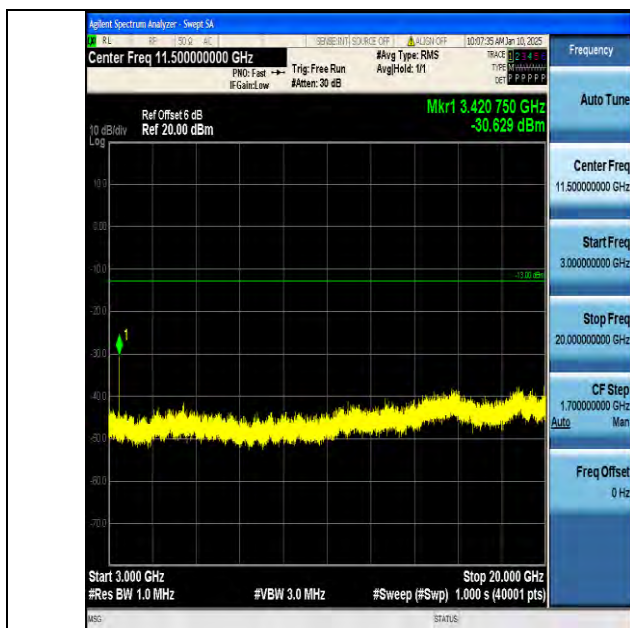
Band66_3MHz_QPSK_131987_1RB#0_3000~20000_3000~20000
