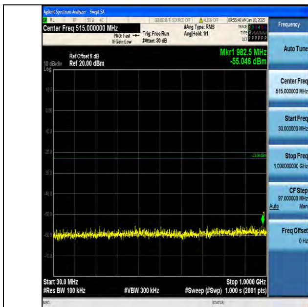
Band66_1.4MHz_16QAM_132322_1RB#0_30~1000_30~1000
