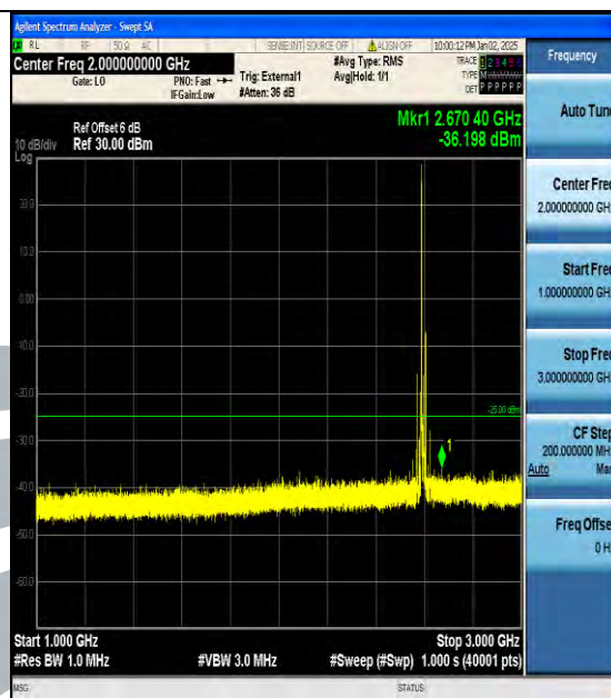
Band38_20MHz_16QAM_38000_1RB#0_1000~3000_1000~3000
