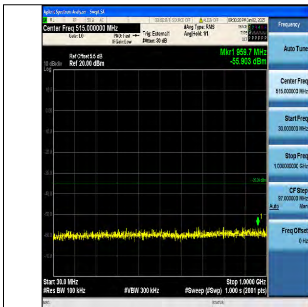
Band38_15MHz_QPSK_38000_1RB#0_30~1000_30~1000
