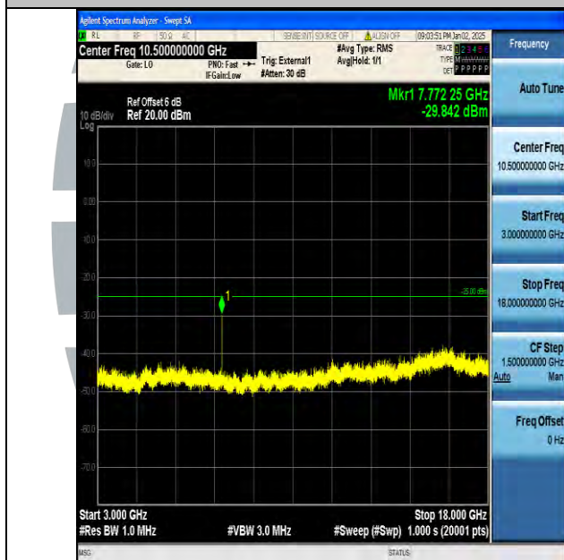
Band38_10MHz_16QAM_38000_1RB#0_3000~18000_3000~18000
