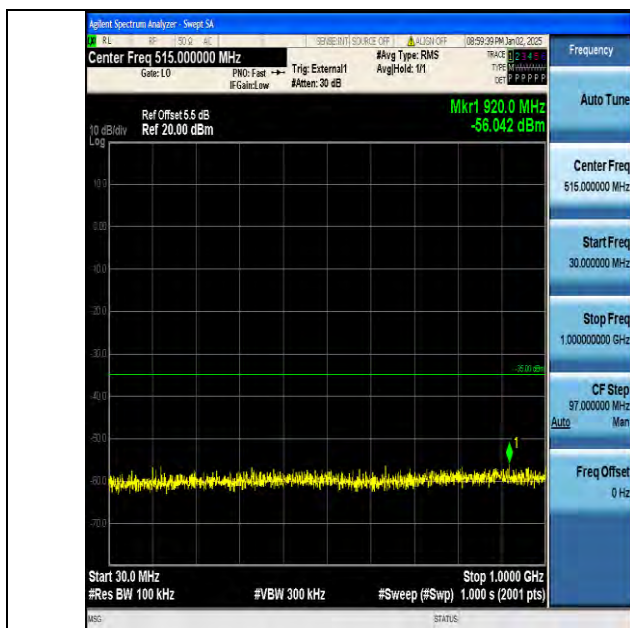
Band38_10MHz_16QAM_37800_1RB#0_30~1000_30~1000
