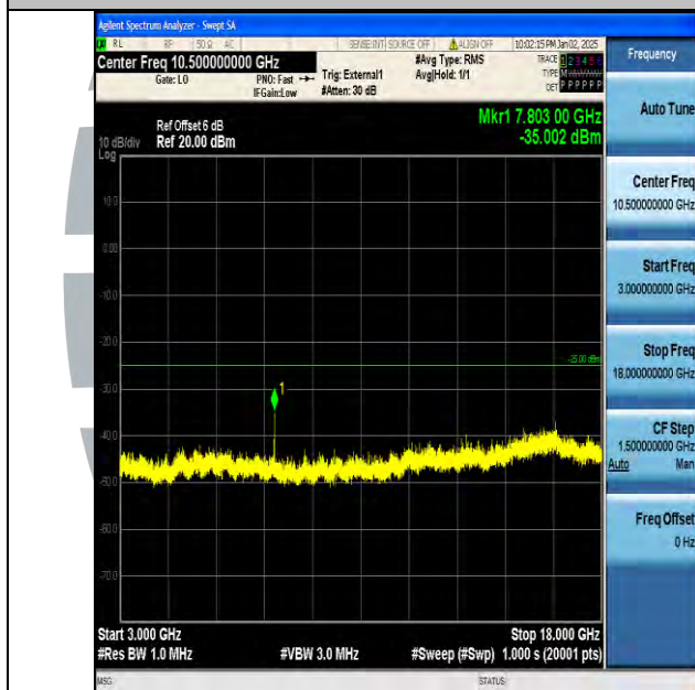
Band38_20MHz_QPSK_38150_1RB#0_3000~18000_3000~18000
