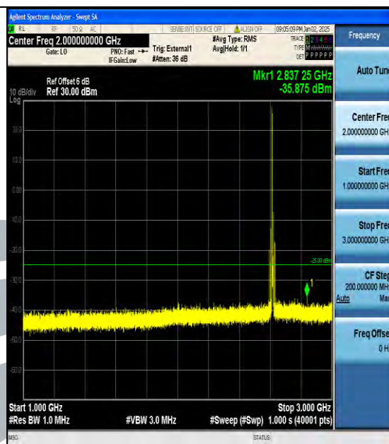
Band38_10MHz_QPSK_38200_1RB#0_1000~3000_1000~3000
