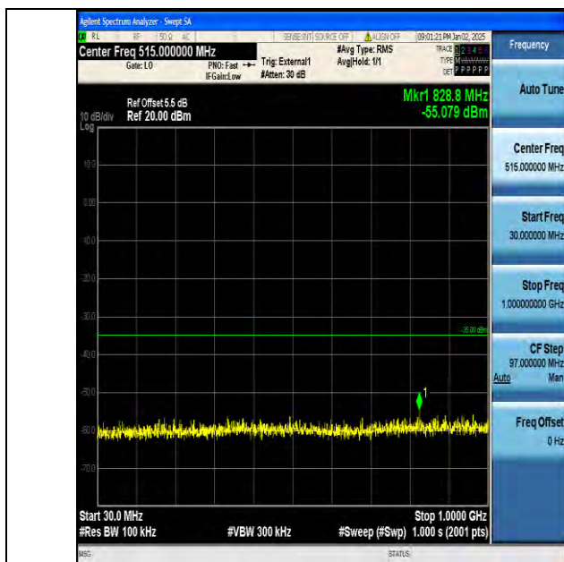
Band38_10MHz_QPSK_38000_1RB#0_30~1000_30~1000
