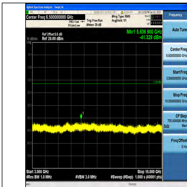
Band17_10MHz_QPSK_23780_1RB#0_3000~10000_3000~10000
