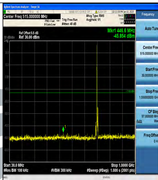
Band17_10MHz_QPSK_23790_1RB#0_30~1000_30~1000
