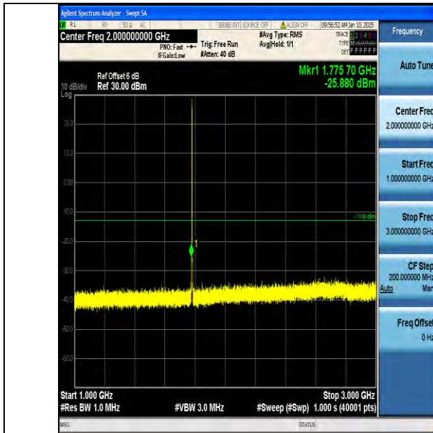
Band66_1.4MHz_16QAM_132665_1RB#0_1000~3000_1000~3000
