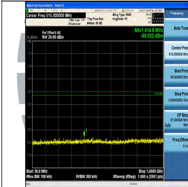
Band66_3MHz_QPSK_131987_1RB#0_30~1000_30~1000
