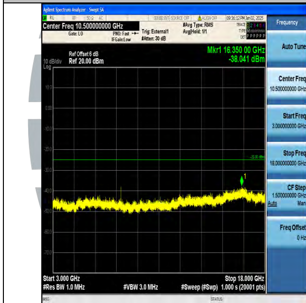
Band38_15MHz_16QAM_38175_1RB#0_3000~18000_3000~18000
