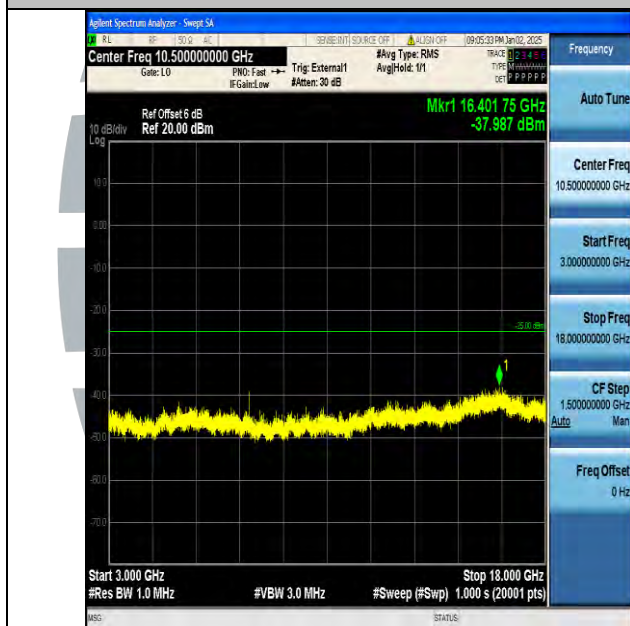
Band38_10MHz_QPSK_38200_1RB#0_3000~18000_3000~18000
