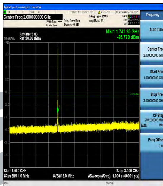
Band66_1.4MHz_16QAM_132322_1RB#0_1000~3000_1000~3000
