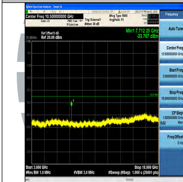
Band38_15MHz_QPSK_37825_1RB#0_3000~18000_3000~18000
