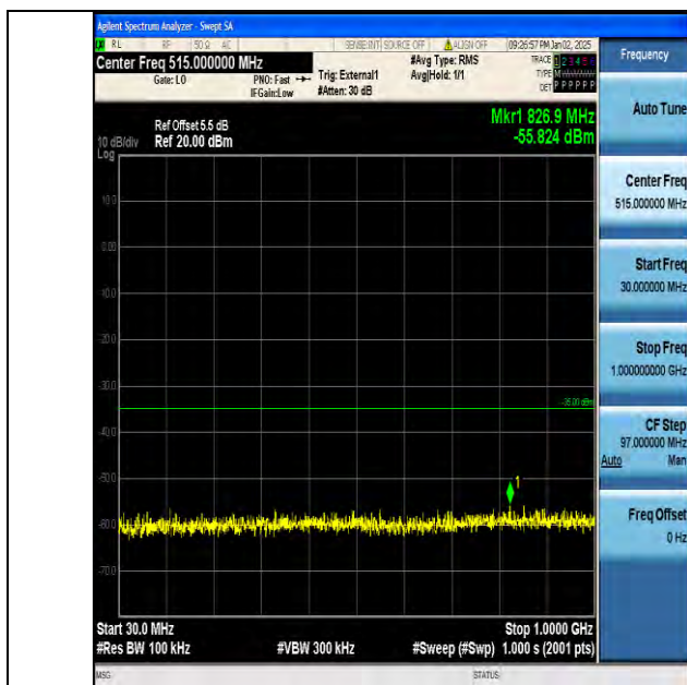
Band38_15MHz_QPSK_37825_1RB#0_30~1000_30~1000
