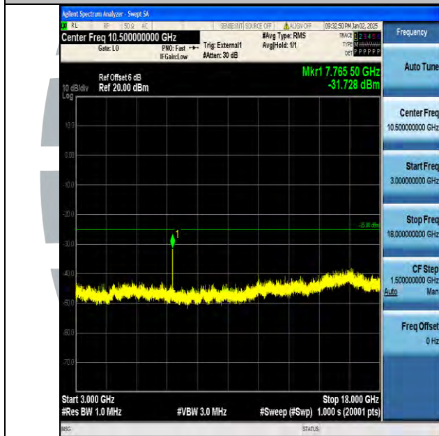
Band38_15MHz_16QAM_38000_1RB#0_3000~18000_3000~18000
