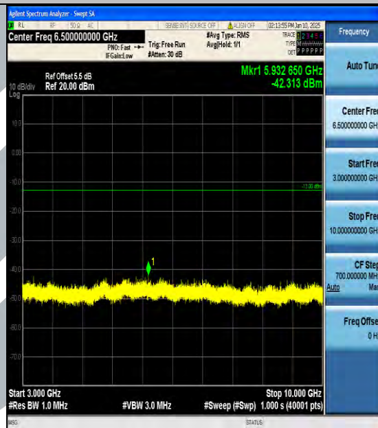
Band17_10MHz_QPSK_23790_1RB#0_3000~10000_3000~10000
