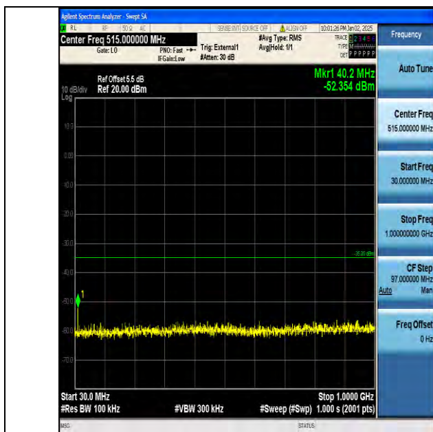
Band38_20MHz_QPSK_38150_1RB#0_30~1000_30~1000
