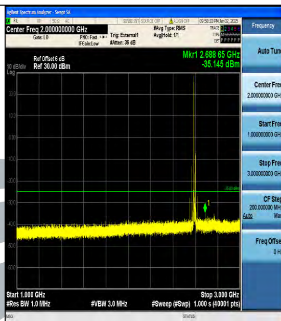
Band38_20MHz_QPSK_38000_1RB#0_1000~3000_1000~3000
