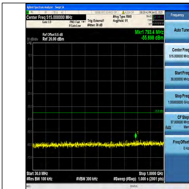
Band38_5MHz_16QAM_37775_1RB#0_30~1000_30~1000
