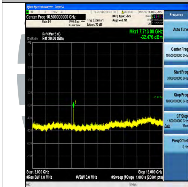
Band38_20MHz_16QAM_37850_1RB#0_3000~18000_3000~18000
