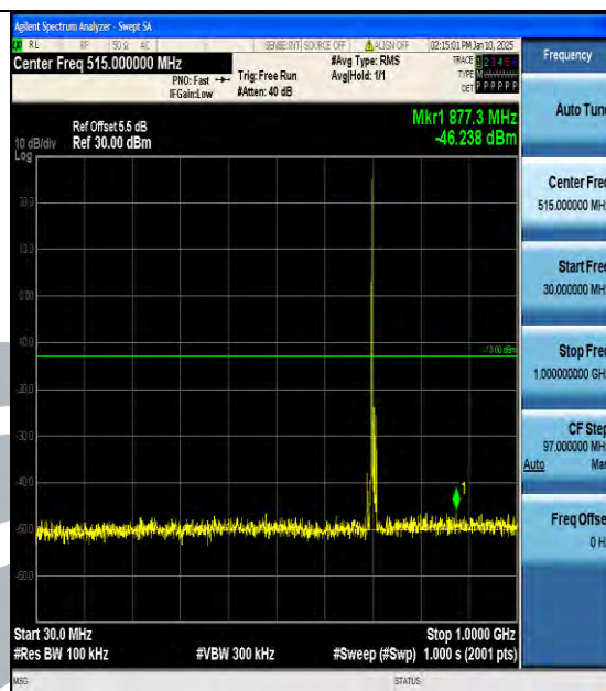
Band17_10MHz_16QAM_23800_1RB#0_30~1000_30~1000
