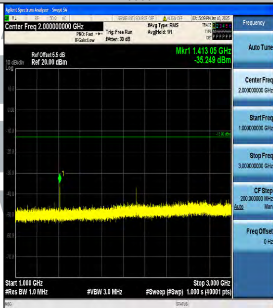
Band17_10MHz_16QAM_23800_1RB#0_1000~3000_1000~3000
