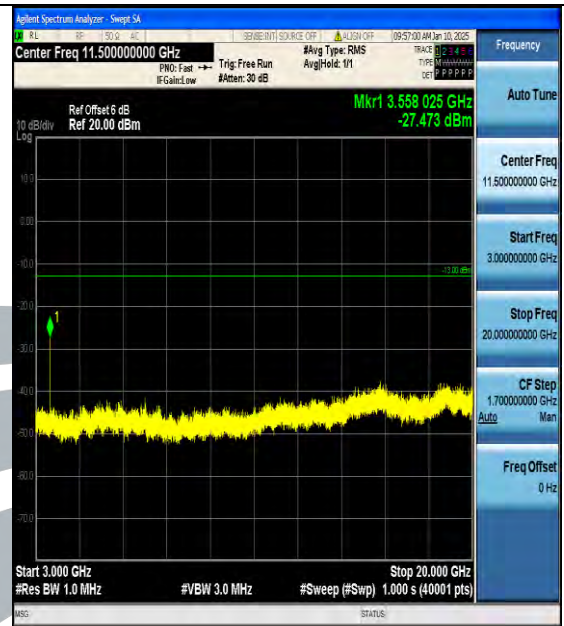
Band66_1.4MHz_16QAM_132665_1RB#0_3000~20000_3000~20000
