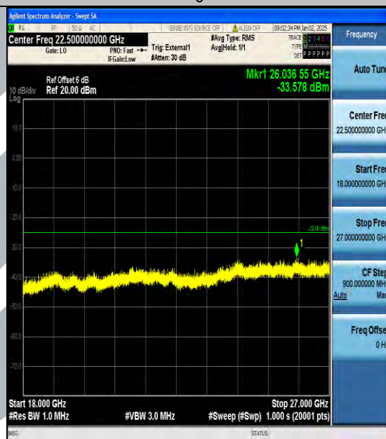
Band38_10MHz_QPSK_38000_1RB#0_18000~27000_18000~27000
