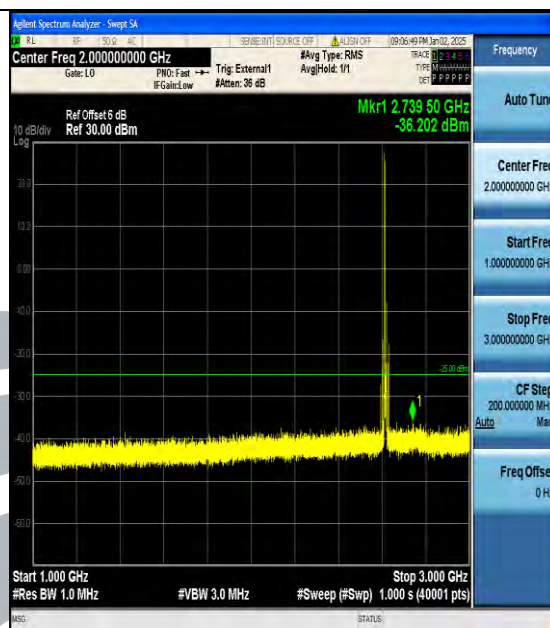
Band38_10MHz_16QAM_38200_1RB#0_1000~3000_1000~3000
