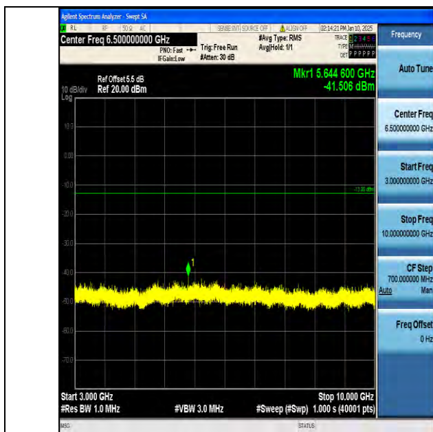
Band17_10MHz_16QAM_23790_1RB#0_3000~10000_3000~10000
