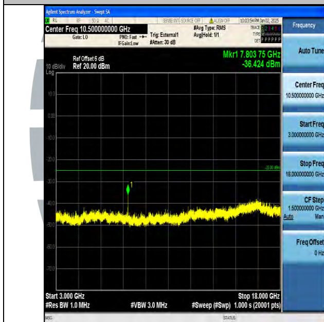
Band38_20MHz_16QAM_38150_1RB#0_3000~18000_3000~18000
