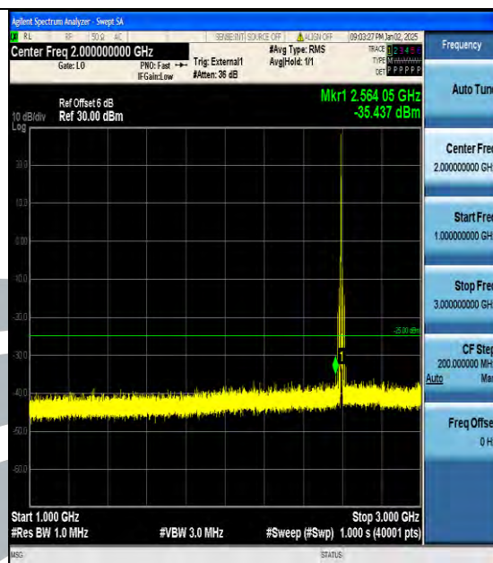
Band38_10MHz_16QAM_38000_1RB#0_1000~3000_1000~3000
