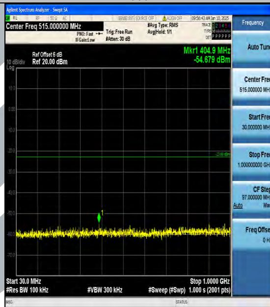
Band66_1.4MHz_16QAM_132665_1RB#0_30~1000_30~1000
