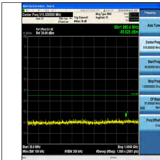
Band38_20MHz_16QAM_38000_1RB#0_30~1000_30~1000
