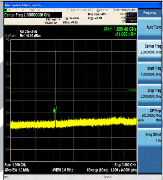
Band66_3MHz_QPSK_131987_1RB#0_1000~3000_1000~3000
