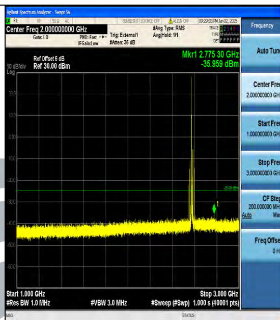
Band38_15MHz_16QAM_37825_1RB#0_1000~3000_1000~3000
