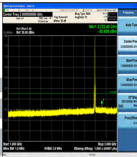
Band38_10MHz_QPSK_38000_1RB#0_1000~3000_1000~3000
