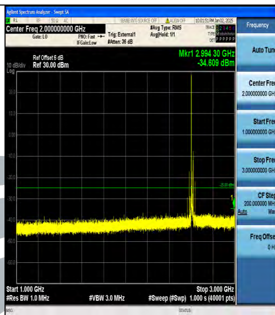
Band38_20MHz_QPSK_38150_1RB#0_1000~3000_1000~3000
