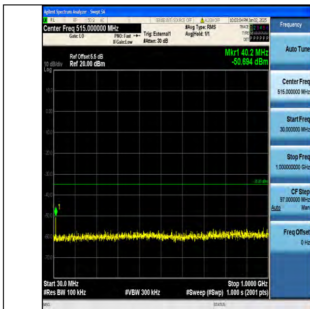
Band38_20MHz_16QAM_38150_1RB#0_30~1000_30~1000
