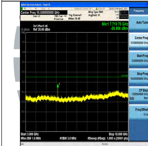
Band38_5MHz_16QAM_37775_1RB#0_3000~18000_3000~18000
