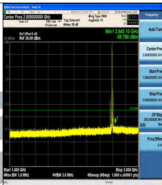
Band38_15MHz_QPSK_38000_1RB#0_1000~3000_1000~3000
