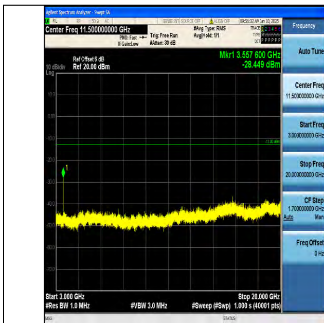
Band66_1.4MHz_QPSK_132665_1RB#0_3000~20000_3000~20000
