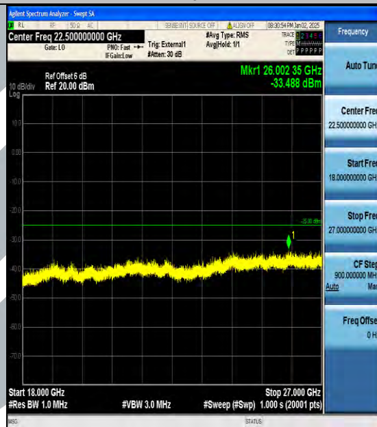
Band38_5MHz_16QAM_37775_1RB#0_18000~27000_18000~27000
