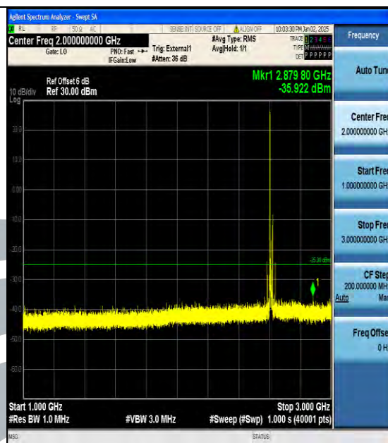
Band38_20MHz_16QAM_38150_1RB#0_1000~3000_1000~3000
