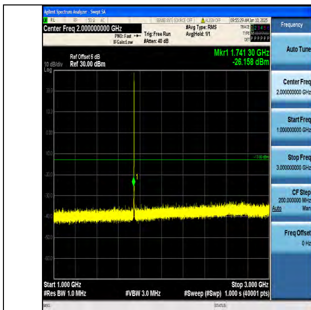
Band66_1.4MHz_QPSK_132322_1RB#0_1000~3000_1000~3000
