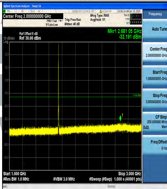
Band66_3MHz_QPSK_132322_1RB#0_1000~3000_1000~3000
