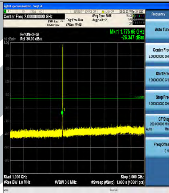
Band66_1.4MHz_QPSK_132665_1RB#0_1000~3000_1000~3000
