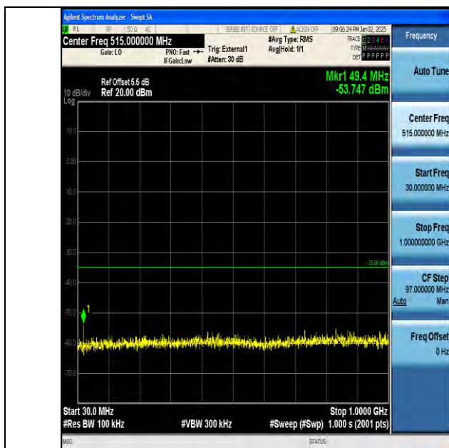
Band38_10MHz_16QAM_38200_1RB#0_30~1000_30~1000
