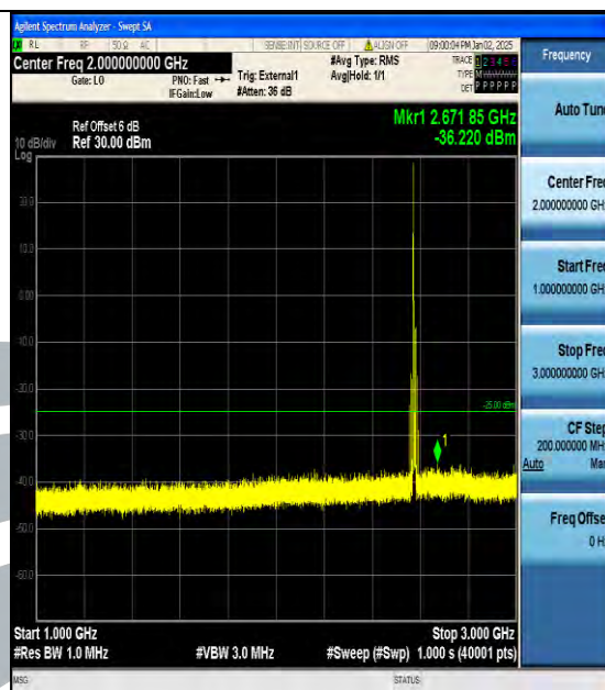
Band38_10MHz_16QAM_37800_1RB#0_1000~3000_1000~3000
