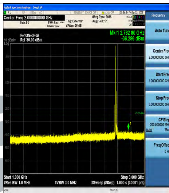
Band38_20MHz_16QAM_37850_1RB#0_1000~3000_1000~3000
