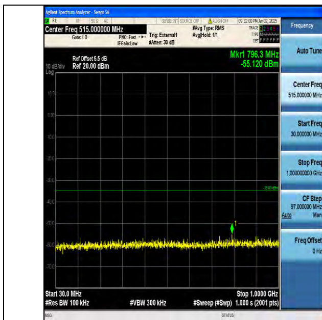
Band38_15MHz_16QAM_38000_1RB#0_30~1000_30~1000
