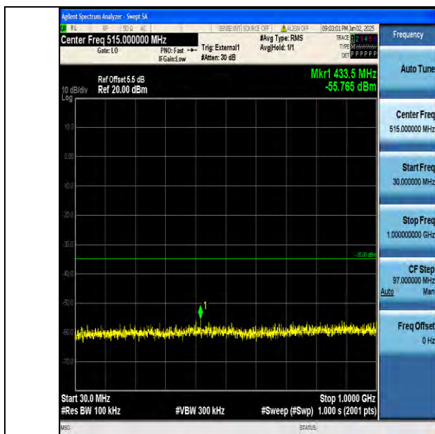
Band38_10MHz_16QAM_38000_1RB#0_30~1000_30~1000
