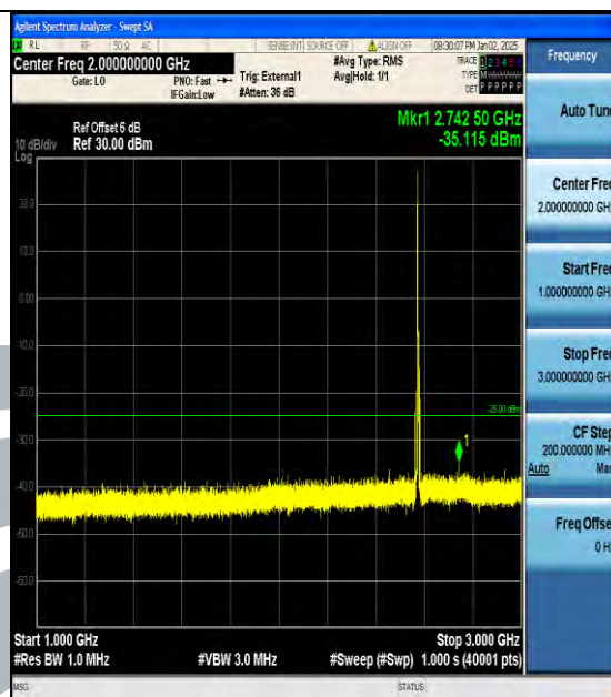
Band38_5MHz_16QAM_37775_1RB#0_1000~3000_1000~3000
