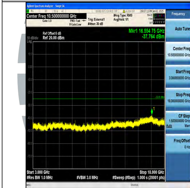
Band38_10MHz_16QAM_38200_1RB#0_3000~18000_3000~18000
