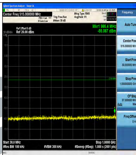
Band66_3MHz_QPSK_132322_1RB#0_30~1000_30~1000
