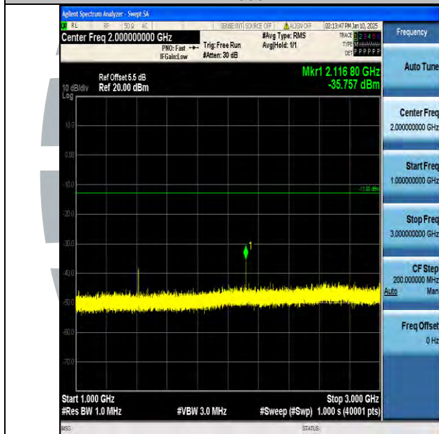
Band17_10MHz_QPSK_23790_1RB#0_1000~3000_1000~3000
