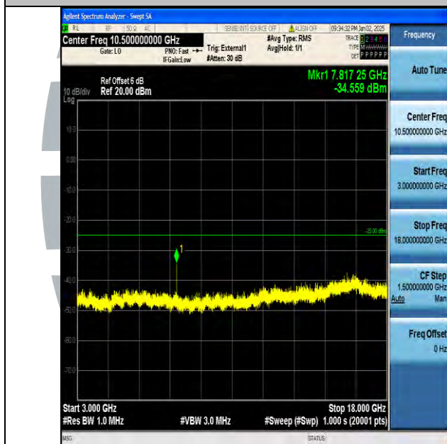
Band38_15MHz_QPSK_38175_1RB#0_3000~18000_3000~18000
