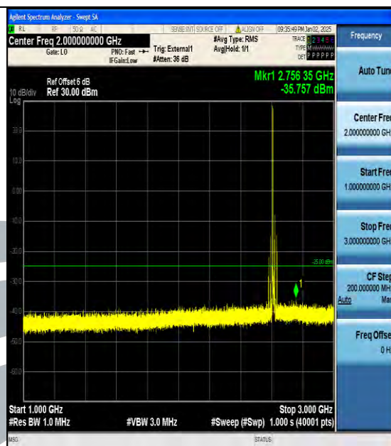
Band38_15MHz_16QAM_38175_1RB#0_1000~3000_1000~3000
