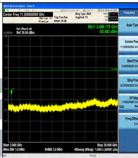
Band66_1.4MHz_QPSK_132322_1RB#0_3000~20000_3000~20000
