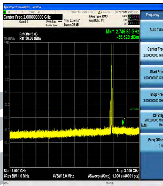
Band38_15MHz_QPSK_37825_1RB#0_1000~3000_1000~3000
