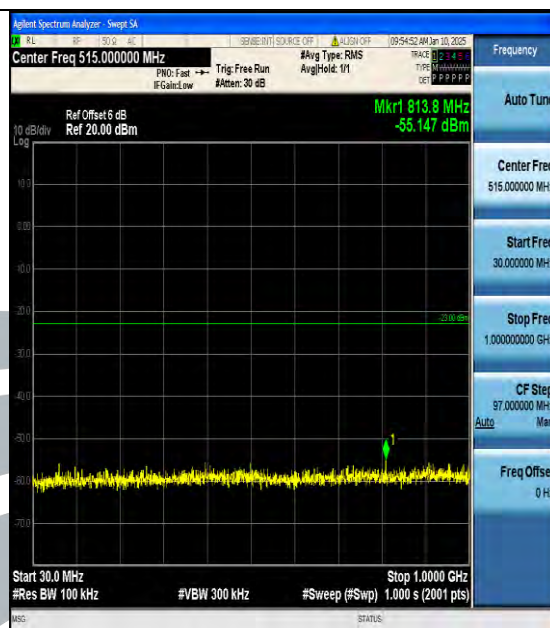
Band66_1.4MHz_16QAM_131979_1RB#0_30~1000_30~1000
