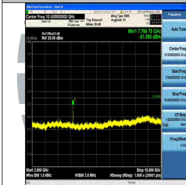
Band38_15MHz_QPSK_38000_1RB#0_3000~18000_3000~18000
