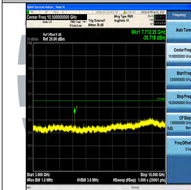
Band38_10MHz_16QAM_37800_1RB#0_3000~18000_3000~18000
