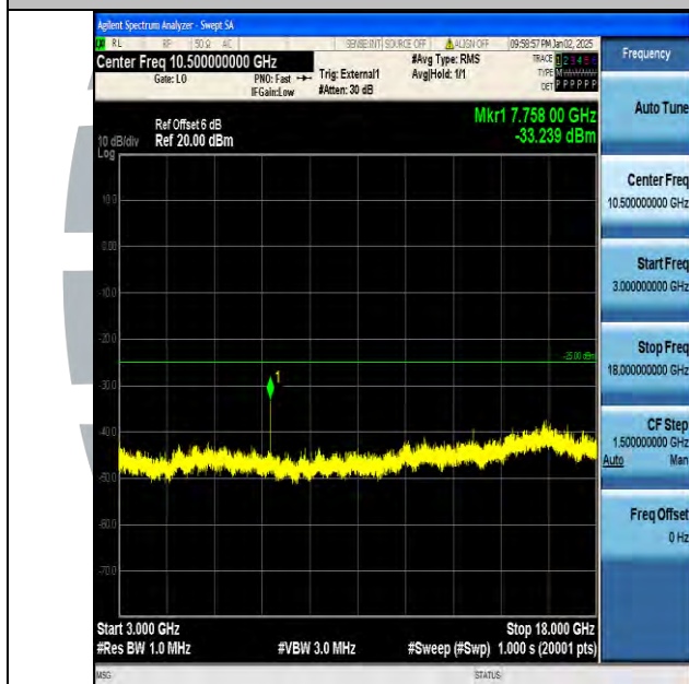
Band38_20MHz_QPSK_38000_1RB#0_3000~18000_3000~18000
