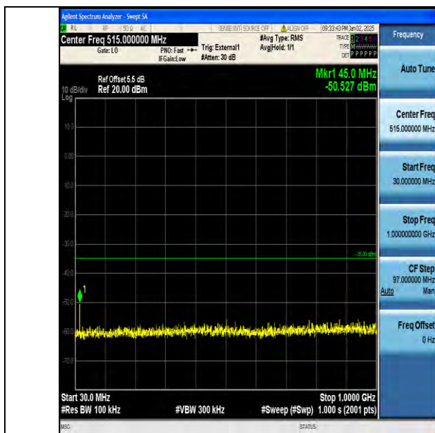
Band38_15MHz_QPSK_38175_1RB#0_30~1000_30~1000
