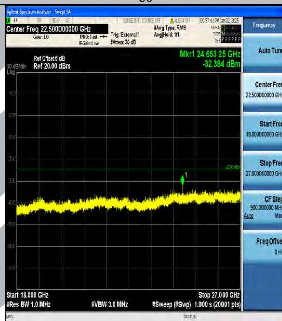
Band38_20MHz_16QAM_37850_1RB#0_18000~27000_18000~27000
