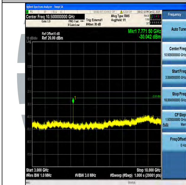
Band38_10MHz_QPSK_38000_1RB#0_3000~18000_3000~18000
