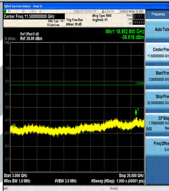
Band66_3MHz_QPSK_132322_1RB#0_3000~20000_3000~20000
