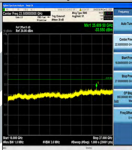
Band38_10MHz_QPSK_38200_1RB#0_18000~27000_18000~27000
