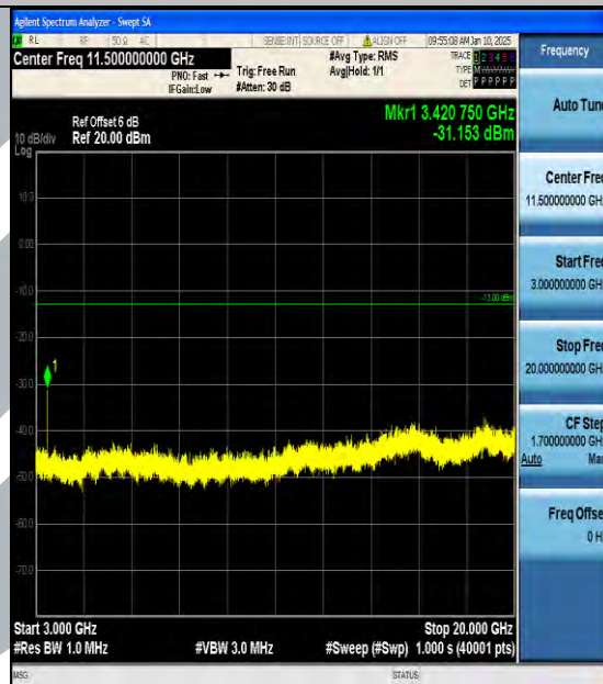
Band66_1.4MHz_16QAM_131979_1RB#0_3000~20000_3000~20000
