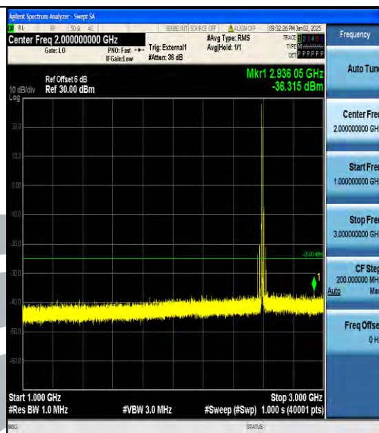
Band38_15MHz_16QAM_38000_1RB#0_1000~3000_1000~3000
