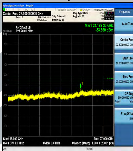
Band38_15MHz_QPSK_37825_1RB#0_18000~27000_18000~27000
