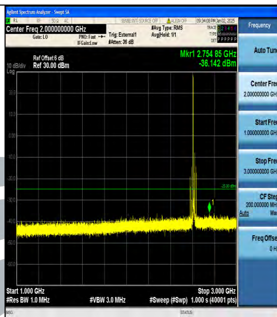
Band38_15MHz_QPSK_38175_1RB#0_1000~3000_1000~3000
