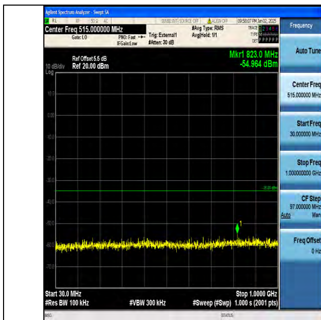
Band38_20MHz_QPSK_38000_1RB#0_30~1000_30~1000
