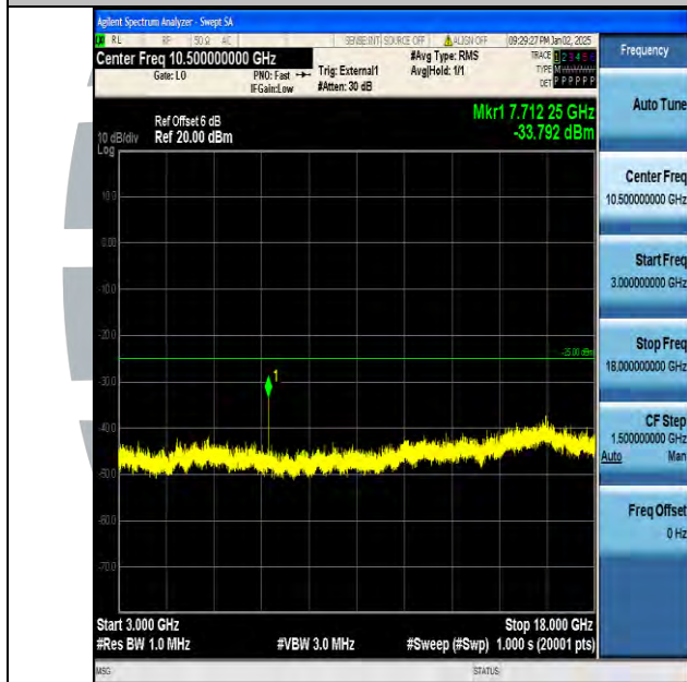
Band38_15MHz_16QAM_37825_1RB#0_3000~18000_3000~18000
