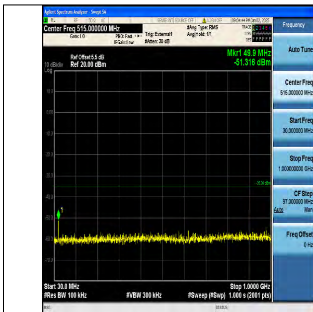
Band38_10MHz_QPSK_38200_1RB#0_30~1000_30~1000
