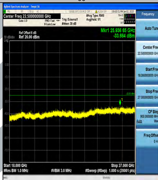
Band38_10MHz_16QAM_37800_1RB#0_18000~27000_18000~27000
