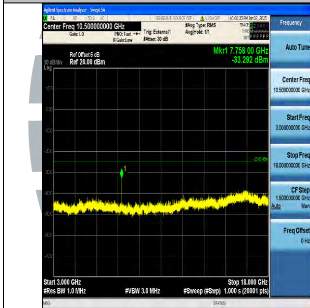
Band38_20MHz_16QAM_38000_1RB#0_3000~18000_3000~18000
