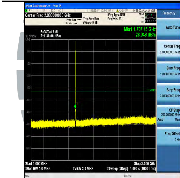
Band66_1.4MHz_16QAM_131979_1RB#0_1000~3000_1000~3000
