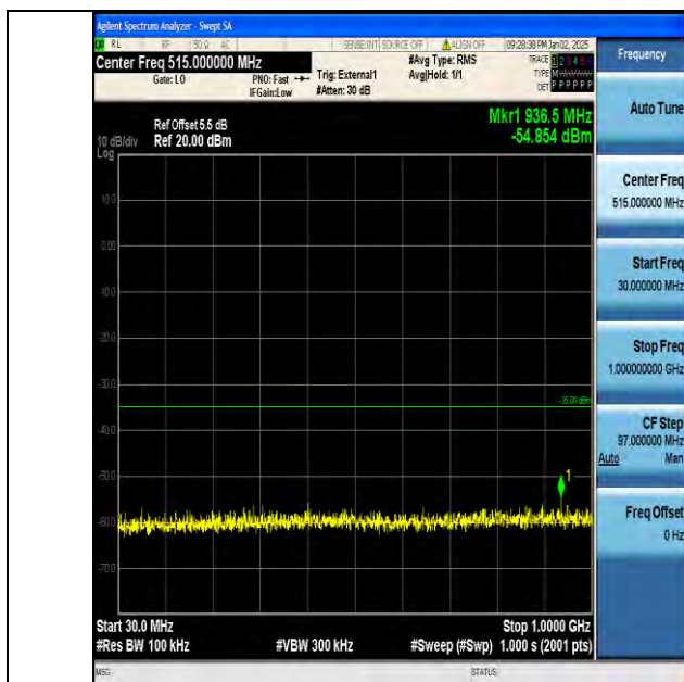
Band38_15MHz_16QAM_37825_1RB#0_30~1000_30~1000
