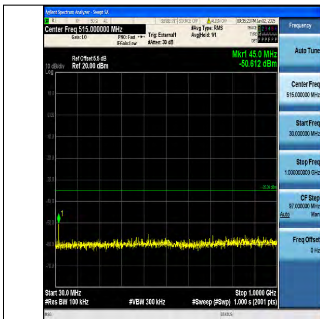
Band38_15MHz_16QAM_38175_1RB#0_30~1000_30~1000
