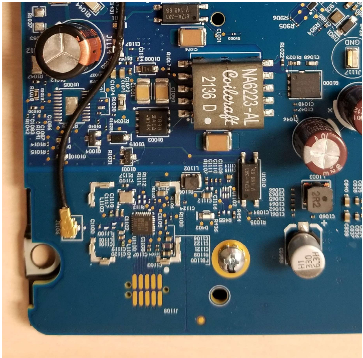
View of the 802.15.4 Transceiver Circuitry with RF Shield Removed
