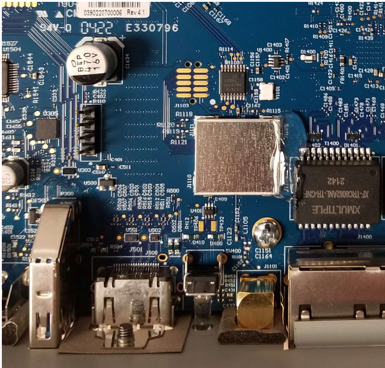
View of the Z-Wave Transceiver Circuitry with RF shield
