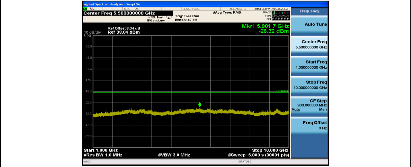
GPRS850-251-1000~10000
