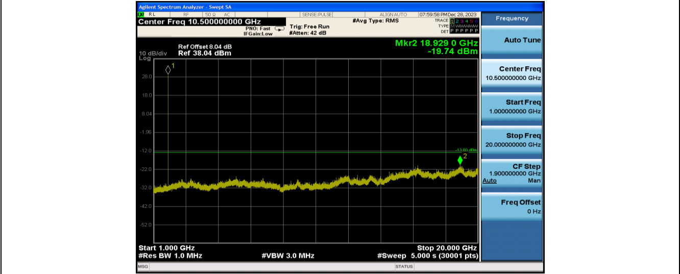
EGPRS1900-512-1000~20000
