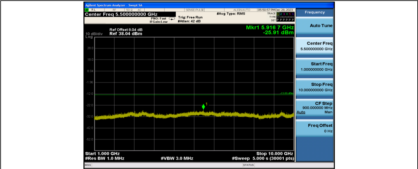
GPRS850-190-1000~10000
