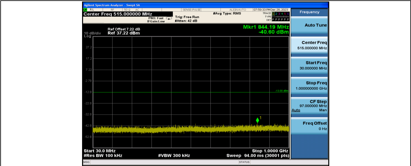
EGPRS1900-512-30~1000
