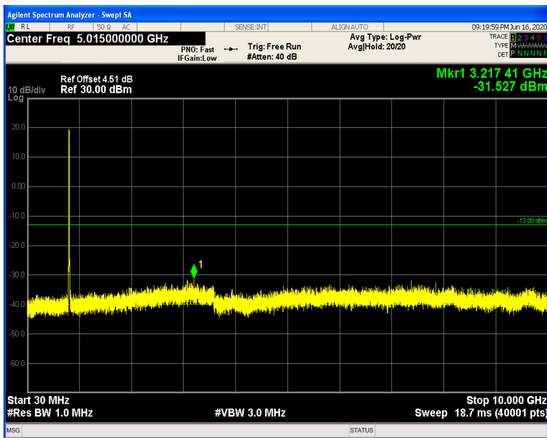
LTE Band5 QAM16 BW=10MHz Channel=20450 RB Size=1 Position=#0
