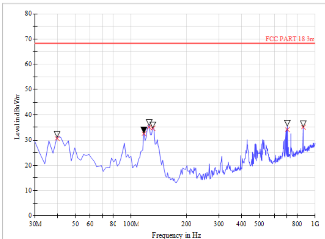
(Plot B: Test Antenna Vertical 30M - 1G)
