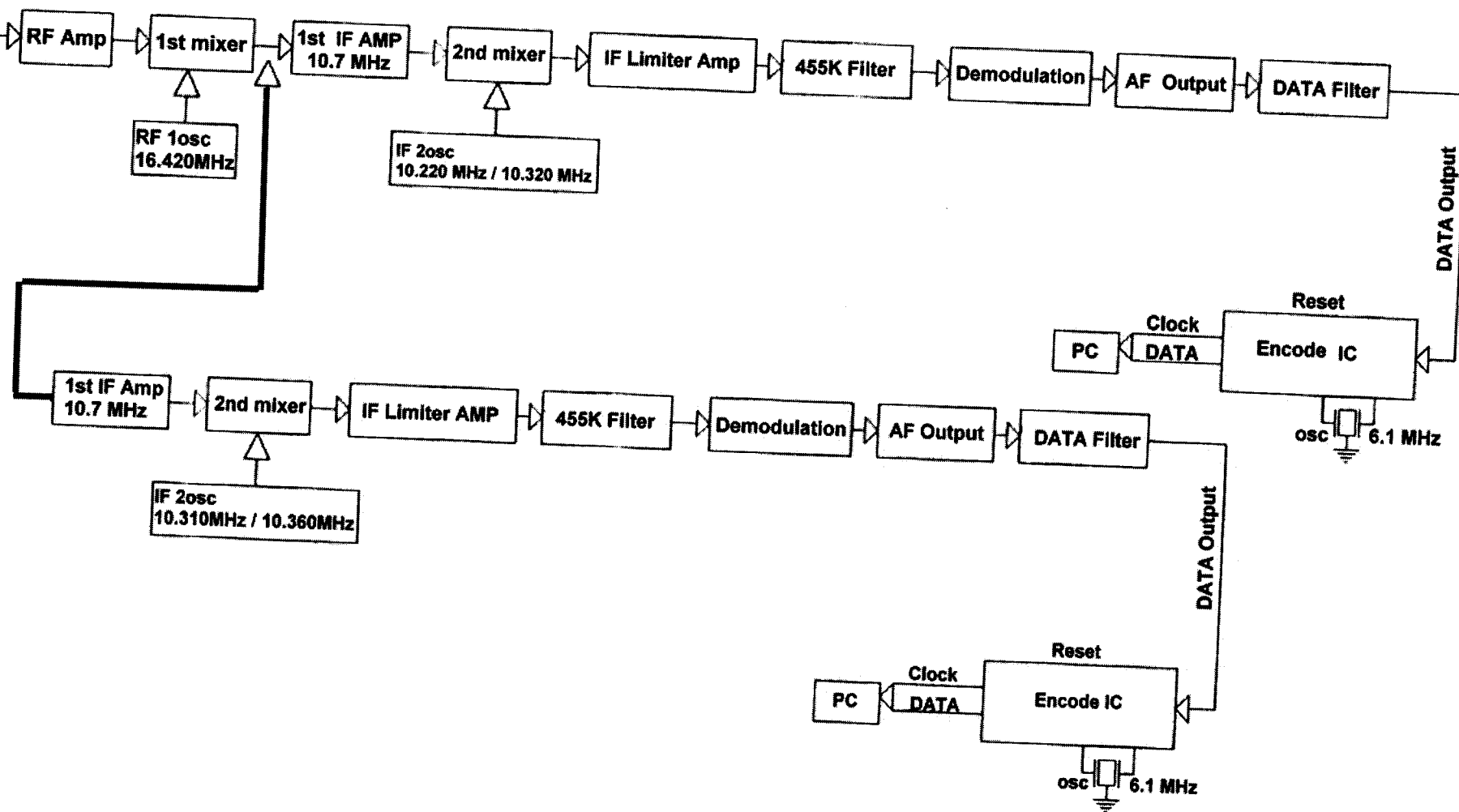
Receiver Block Diagram
