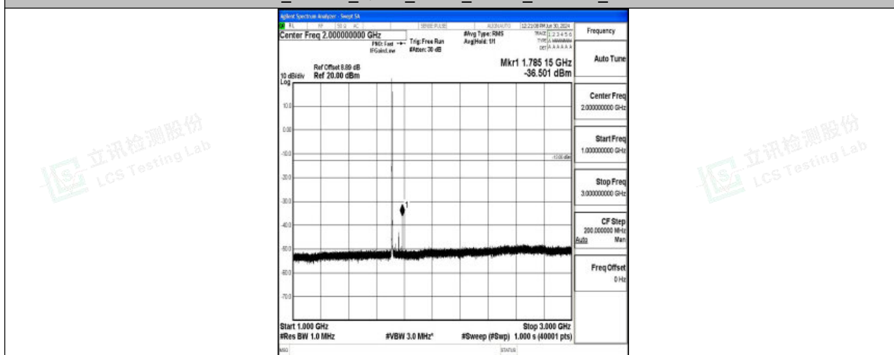
Band4_1.4MHz_QPSK_19957_1RB#0_1000~3000_1000~3000
