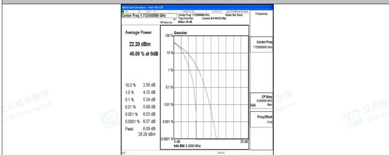
Band4-5MHz-QPSK-20175-1RB#0-PASS
