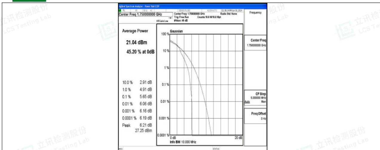
Band4-10MHz-16QAM-20350-1RB#0-PASS
