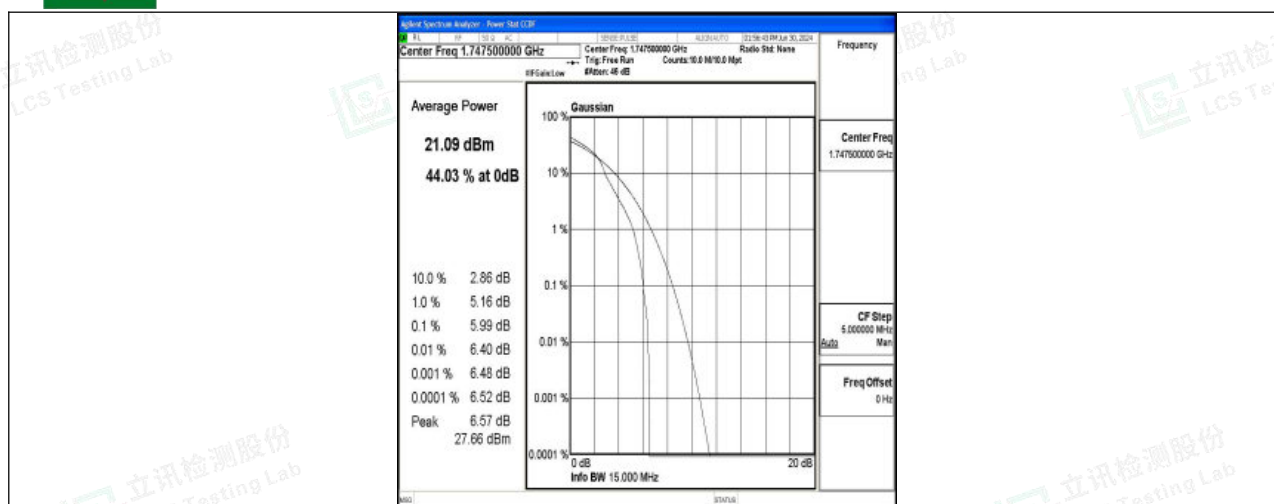
Band4-15MHz-16QAM-20325-1RB#0-PASS
