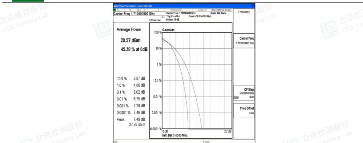
Band4-5MHz-16QAM-19975-25RB#0-PASS
