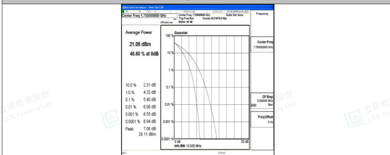
Band4-10MHz-QPSK-20350-50RB#0-PASS
