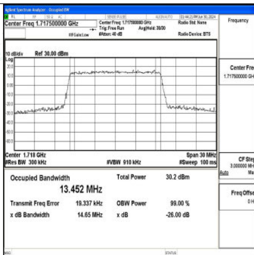
Band4-15MHz-QPSK-20025-75RB#0-PASS
