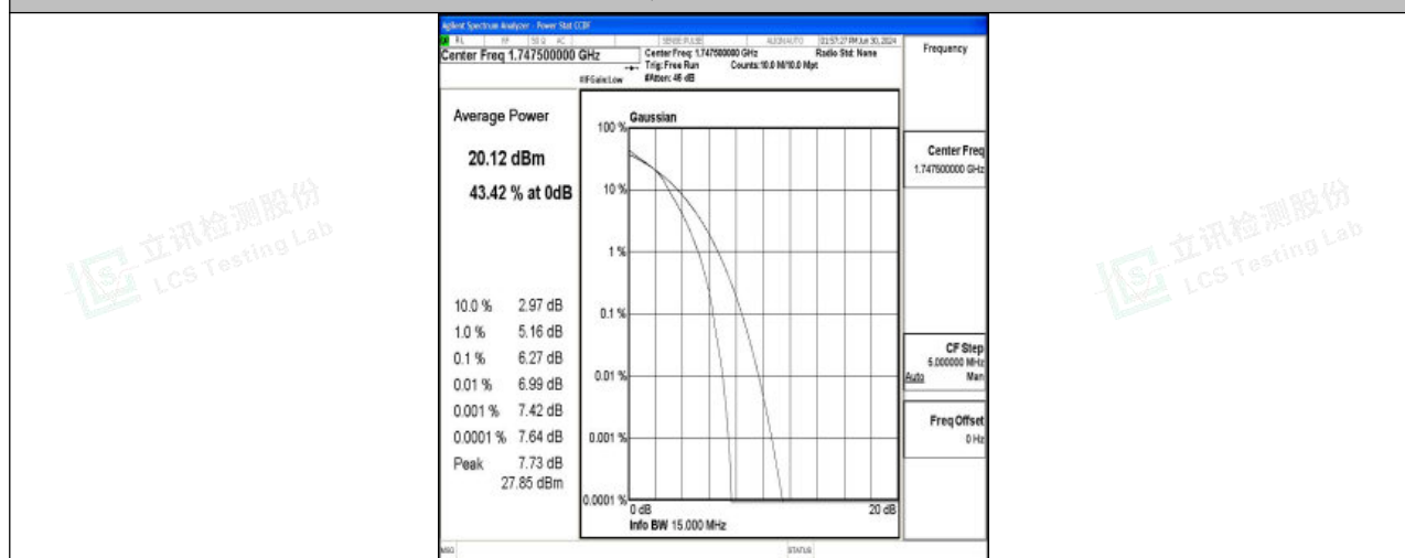
Band4-15MHz-16QAM-20325-75RB#0-PASS
