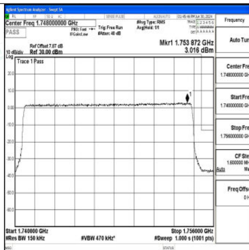
Band4_15MHz_QPSK_20325_75RB#0
