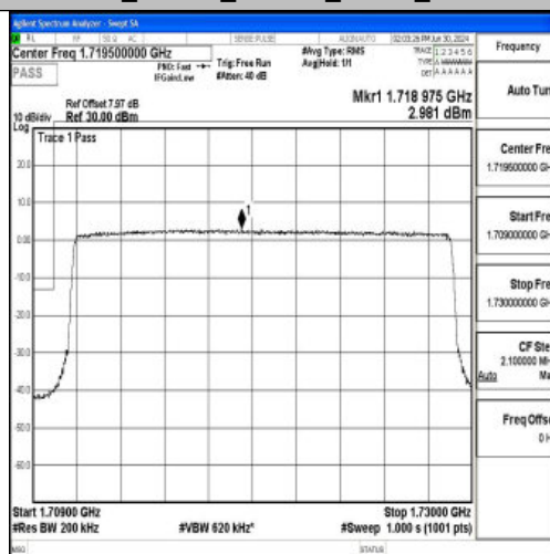
Band4_20MHz_QPSK_20050_100RB#0
