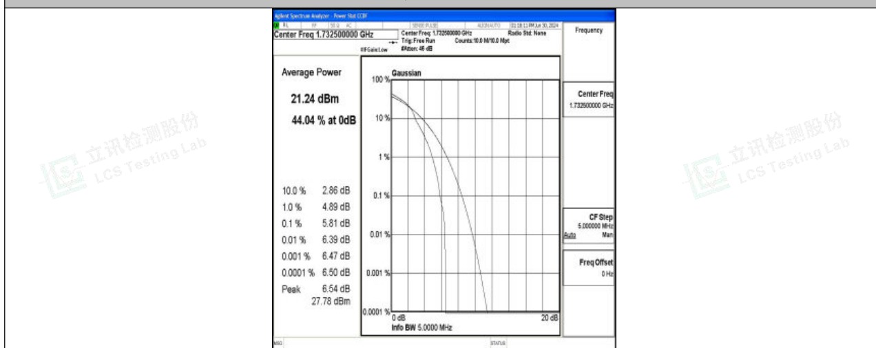
Band4-5MHz-16QAM-20175-1RB#0-PASS
