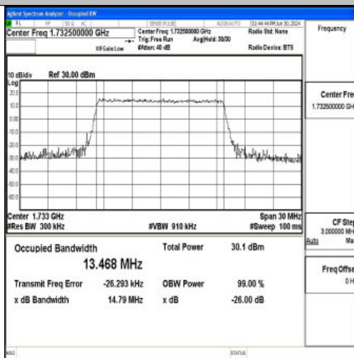
Band4-15MHz-QPSK-20175-75RB#0-PASS
