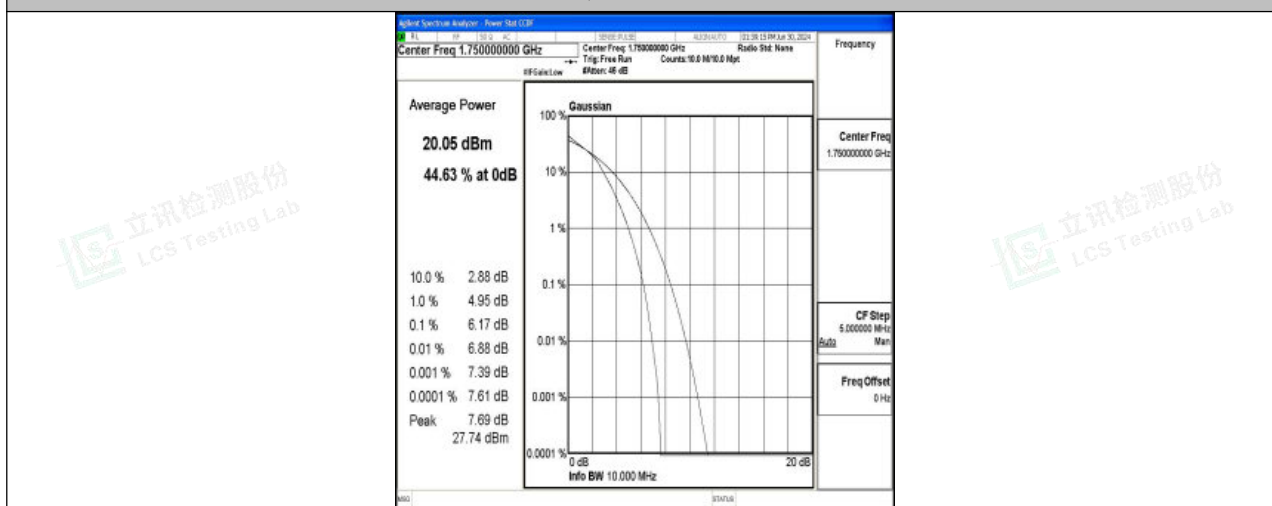
Band4-10MHz-16QAM-20350-50RB#0-PASS
