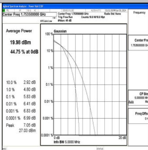
Band4-3MHz-16QAM-20385-15RB#0-PASS
