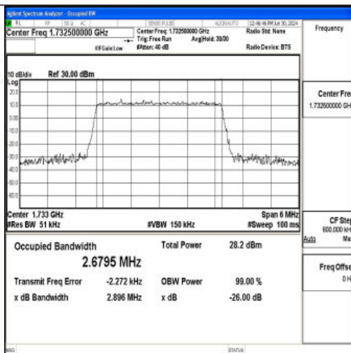
Band4-3MHz-16QAM-20175-15RB#0-PASS
