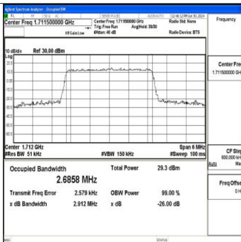
Band4-3MHz-QPSK-19965-15RB#0-PASS
