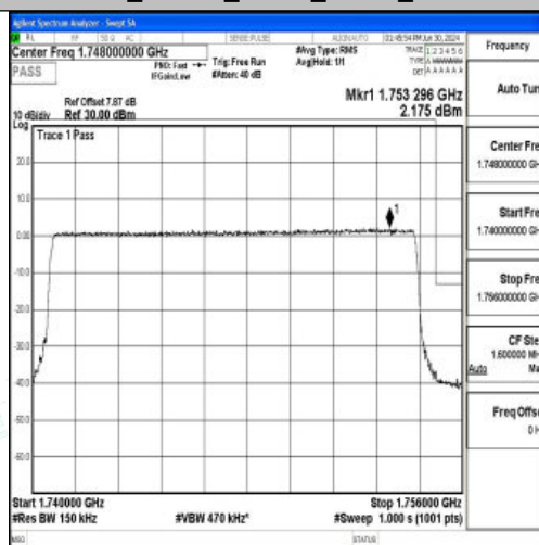
Band4_15MHz_16QAM_20325_75RB#0
