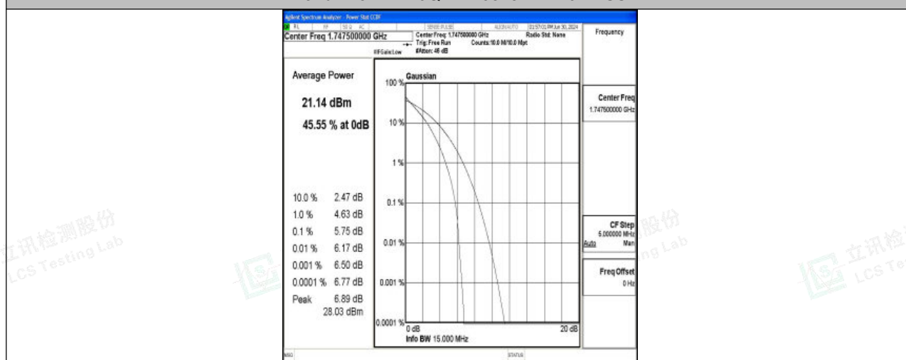
Band4-15MHz-QPSK-20325-75RB#0-PASS
