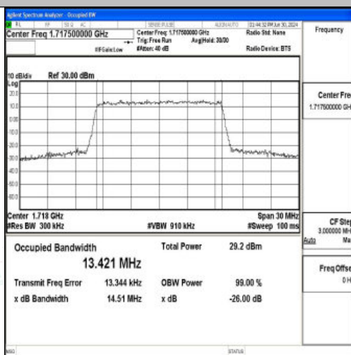
Band4-15MHz-16QAM-20025-75RB#0-PASS
