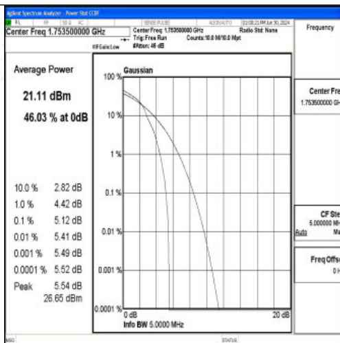
Band4-3MHz-16QAM-20385-1RB#0-PASS
