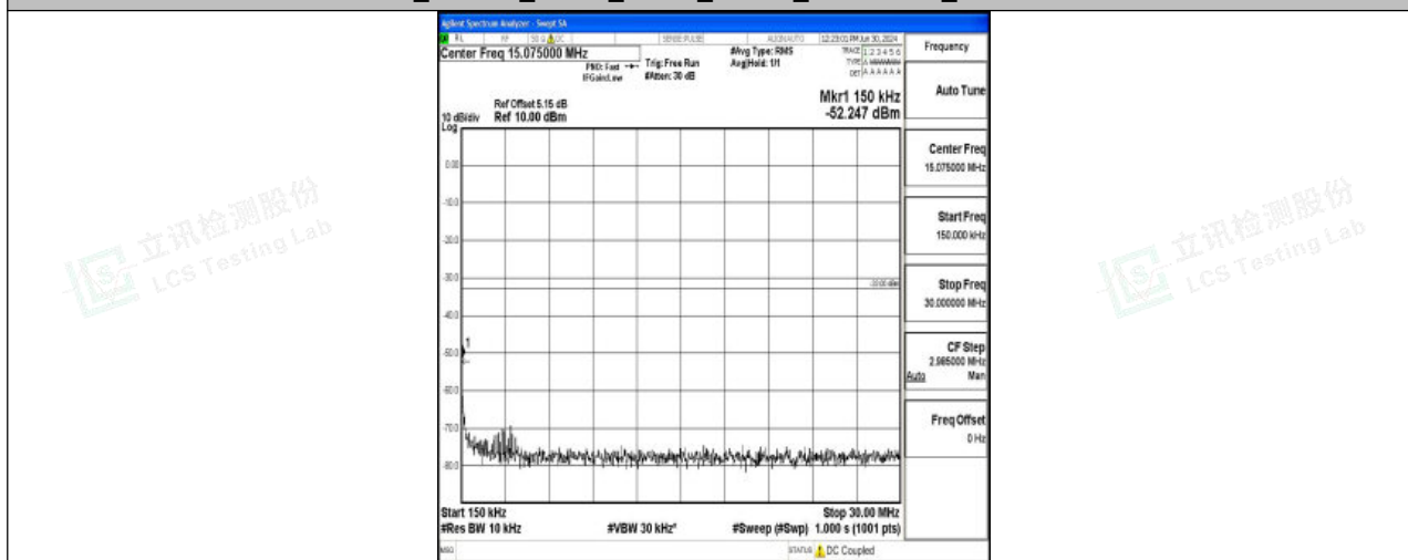
Band4_1.4MHz_QPSK_20393_1RB#0_0.15~30_0.15~30
