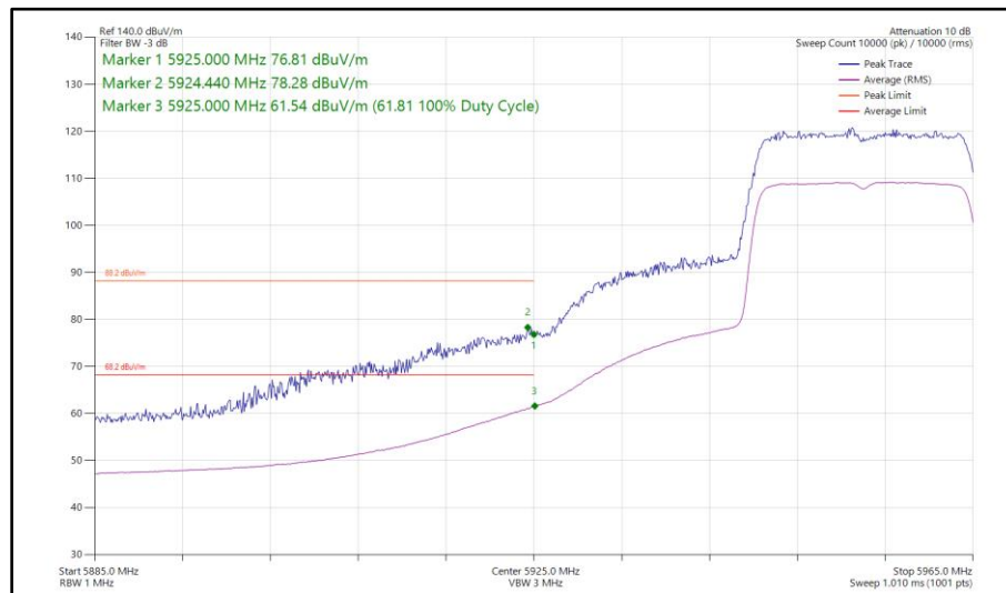
Figure 163 - 802.11ax HE20, SU, SISO, Core 0 - 5955 MHz Band Edge Frequency 5925 MHz
