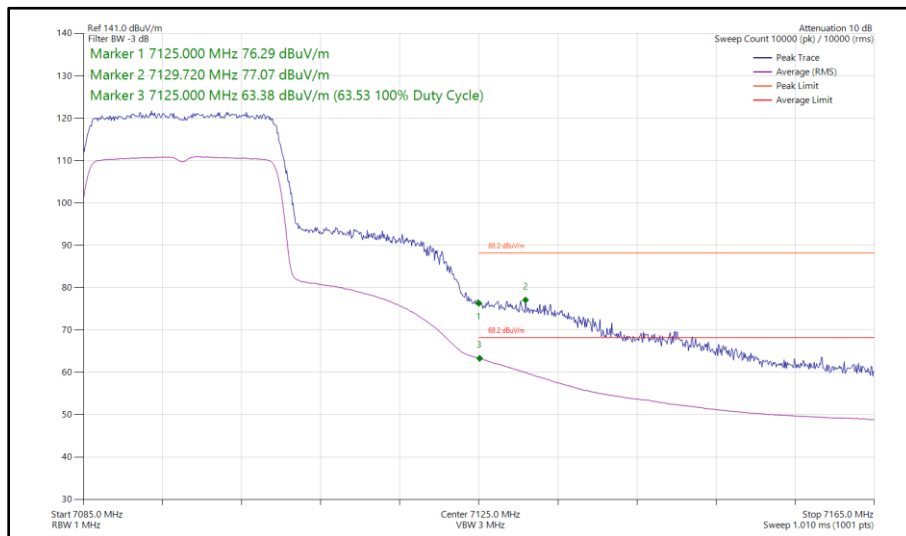
Figure 167 - 802.11ax HE20, SU, SISO, Core 0 - 7095 MHz Band Edge Frequency 7125 MHz
