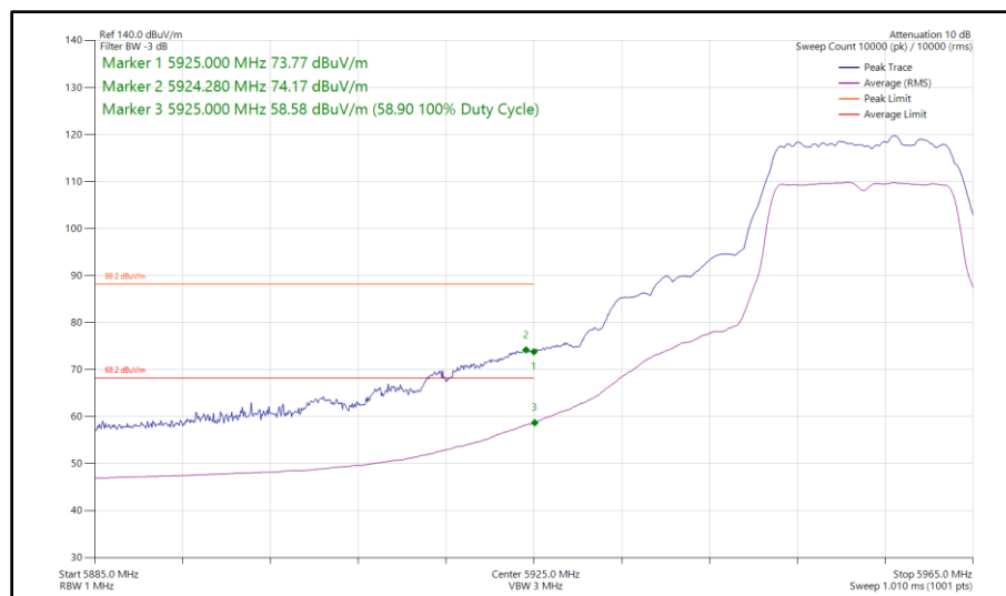
Figure 162 - 802.11a, SISO, Core 0 - 5955 MHz Band Edge Frequency 5925 MHz
