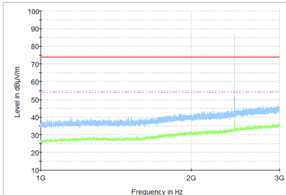
Fig.51 Radiated Spurious Emission (Ch19, 1 GHz - 3 GHz), 2M
