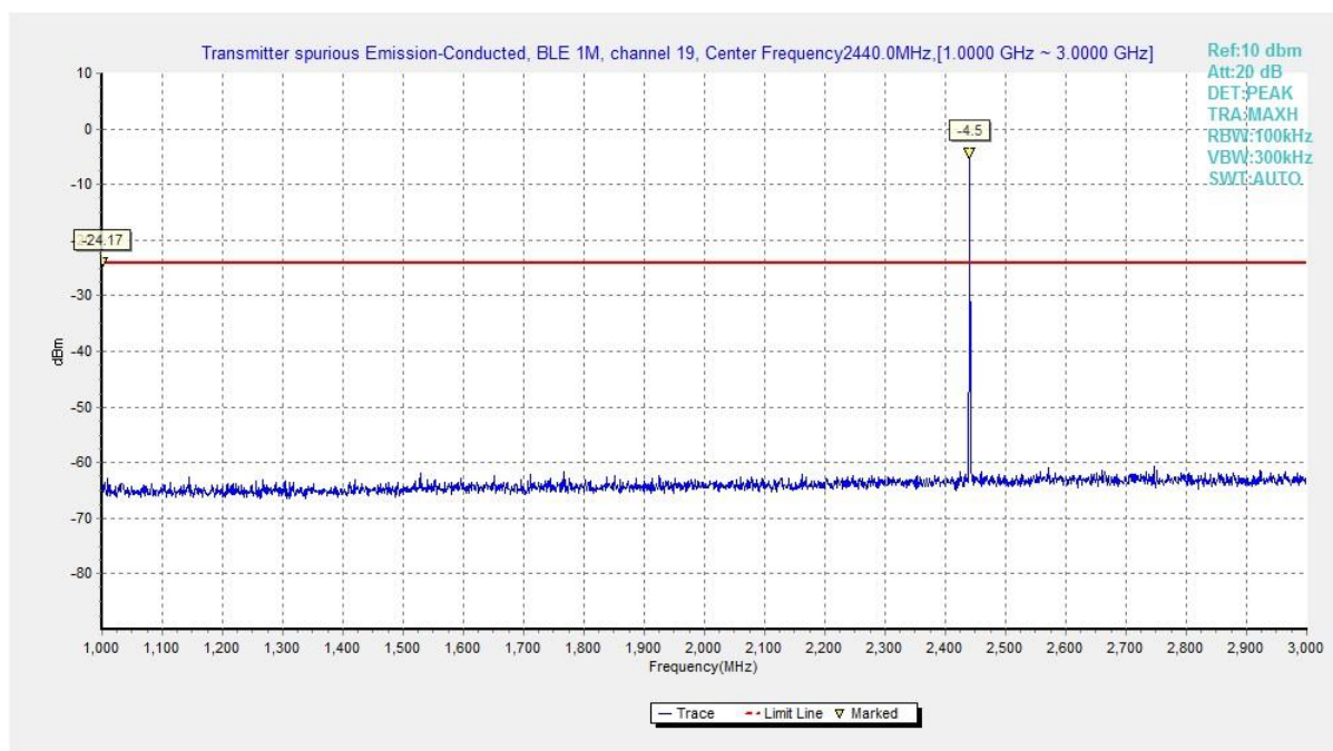
Fig.21 Conducted Spurious Emission (Ch19, 1 GHz-3 GHz), LE 1M
