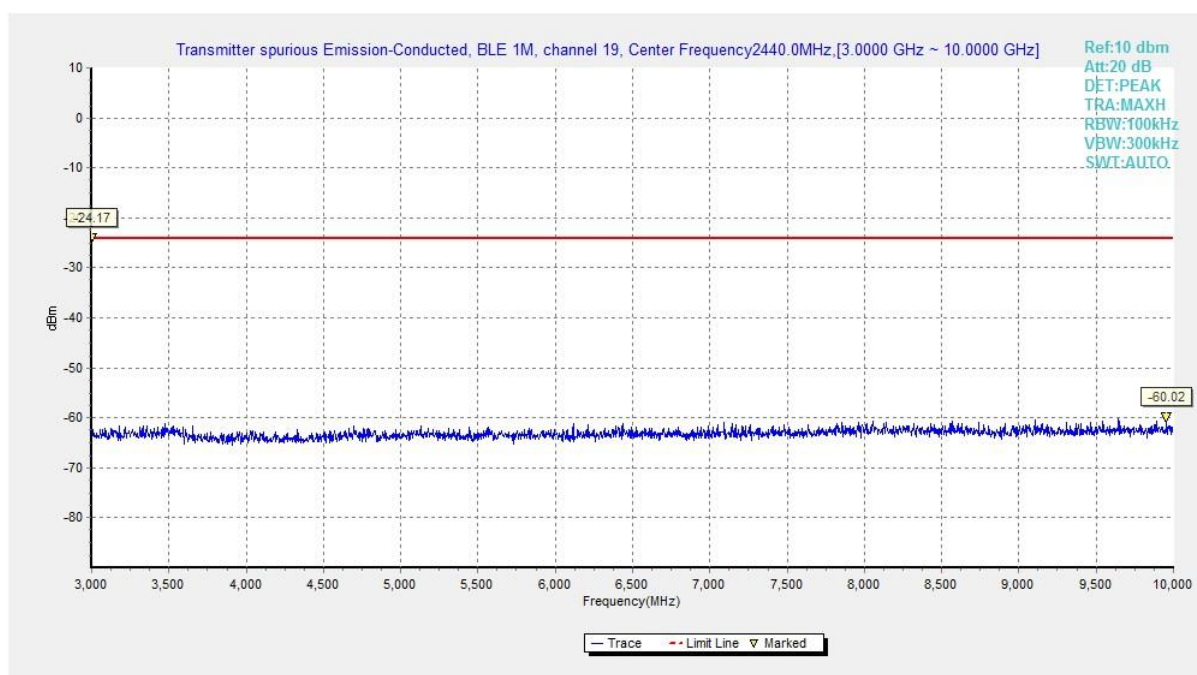
Fig.22 Conducted Spurious Emission (Ch19, 3 GHz-10 GHz), LE 1M
