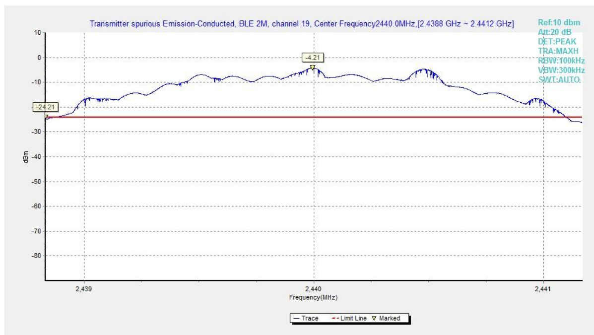
Fig.31 Conducted Spurious Emission (Ch19, Center Frequency), LE 2M
