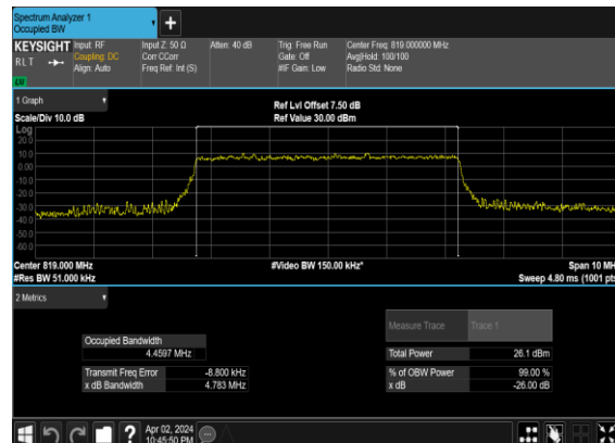
N26(5M)_CP-OFDM_16 QAM_Outer_Full_Mid_CH
