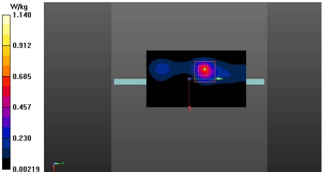
Fig. 13 LTE Band 41(PC3) Body
