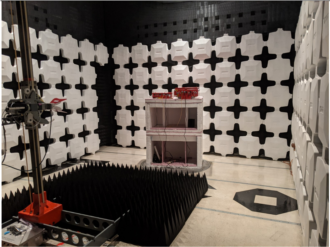
Radiated, Above 1 GHz
