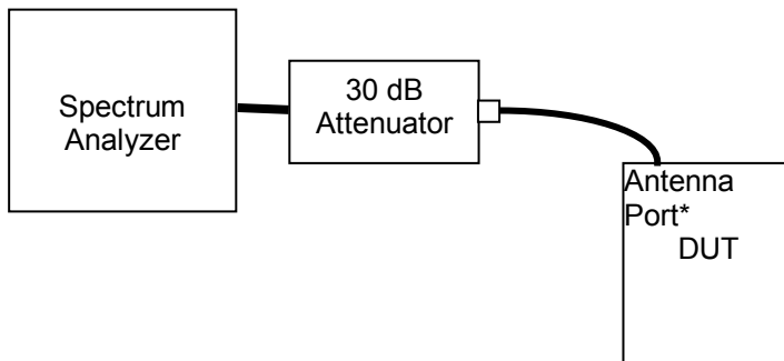
Figure A.6-1 - Setup Drawing GPRS & EDGE Conducted Power Measurements
